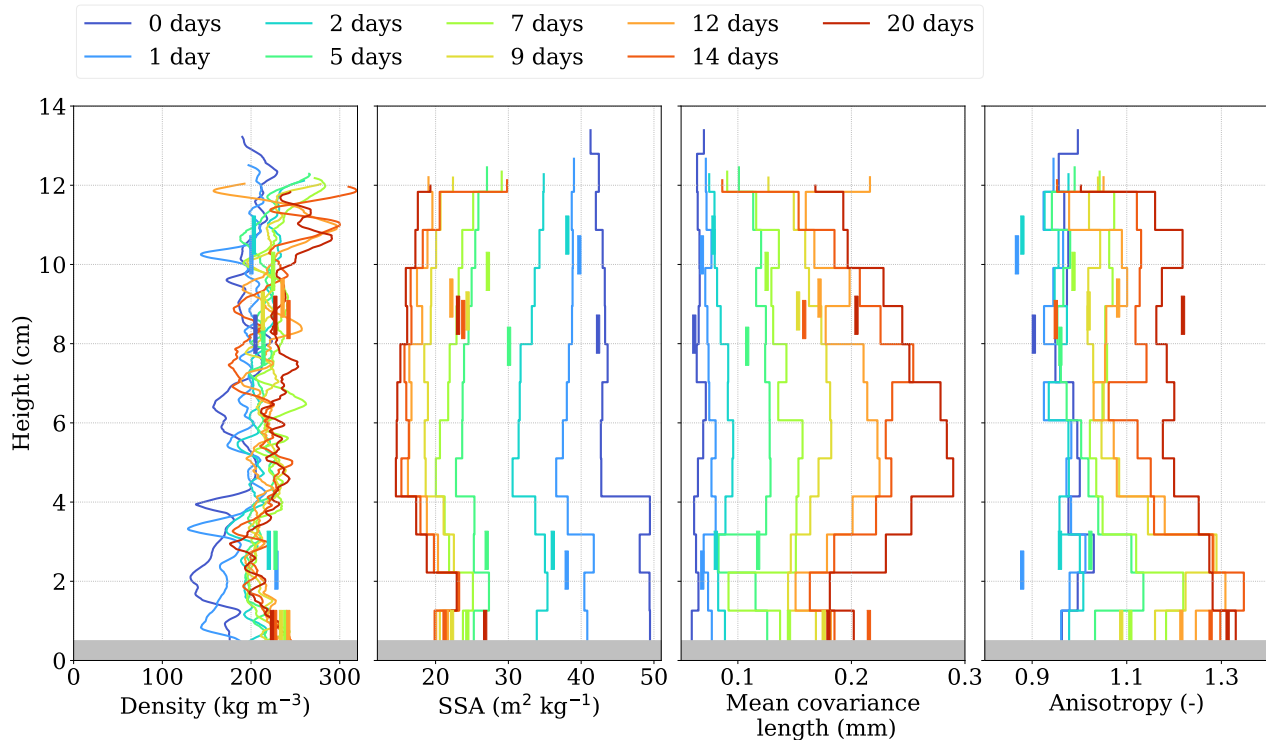
Figure 5. Vertical profiles of the microstructural properties of Experiment A. Properties computed from the large samples at 21\ \mu\text{m} are shown by step curves and those from the small samples at 8\ \mu\text{m} by vertical bars. The density of the samples at 21\ \mu\text{m} is computed on each slice with a running average (see Sec. 1.2). The grey area at the bottom represents the disturbed area caused by the snow sampling.
