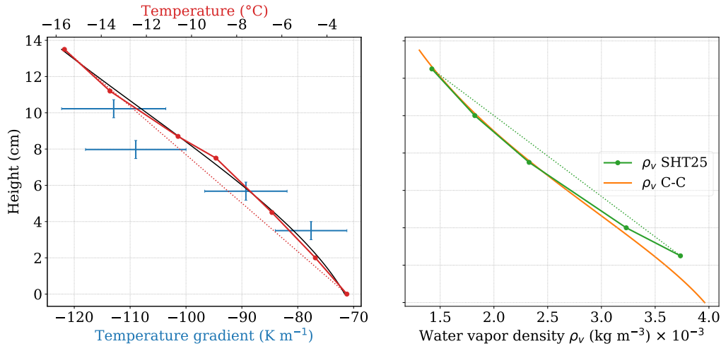
Figure 3. Temperature, temperature gradient and water vapor density profiles during the steady condition stage of Experiment A. The black line represents the polynomial fit on the PT100 data. The orange line displays the Clausius-Clapeyron equation applied to the temperature fit. The straight dotted red and green lines, which connect the higher and lower points of the temperature and the water vapor density, respectively, are presented to help highlighting the shape of the curves.
