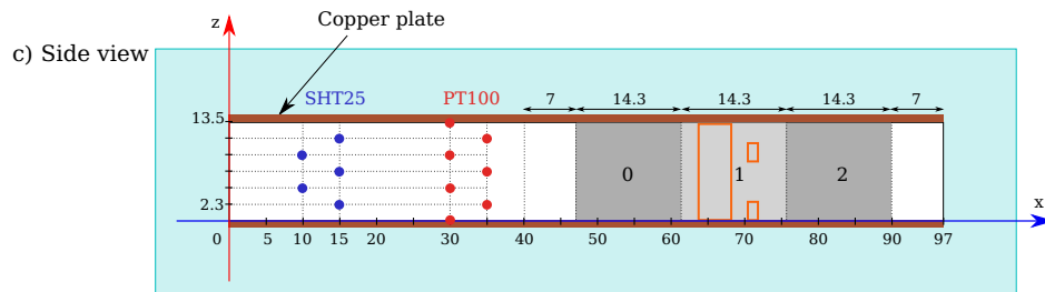
Figure 1. (a) Photograph of the experimental setup of Experiment A. (b) Schematic view from above the instrumented box. (c) Schematic view from the side. The locations (in cm) of the 2 types of sensors are shown with blue and red dots. The tomography sample locations are numbered from 0 to 8 following the chronology of the samplings. The orange contours represent the tomographies areas for the session 1.
