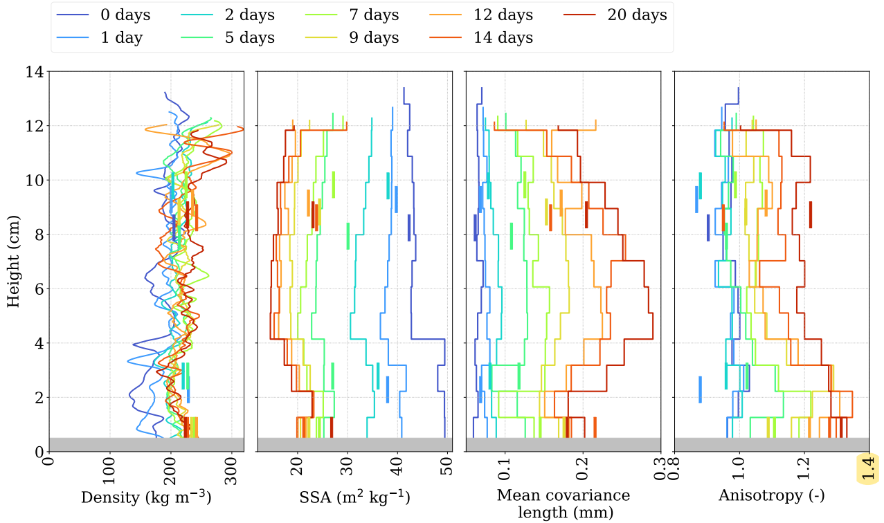
Figure 5. Vertical profiles of the microstructural properties of Experiment A. Properties computed from the large samples at 21\ \mu\text{m} are shown by step curves and those from the small samples at 8\ \mu\text{m} by vertical bars. The density of the samples at 21\ \mu\text{m} is computed on each slice with a running average (see Sec. 1.2). The grey area at the bottom represents the disturbed and unreliable area caused by the snow sampling.
