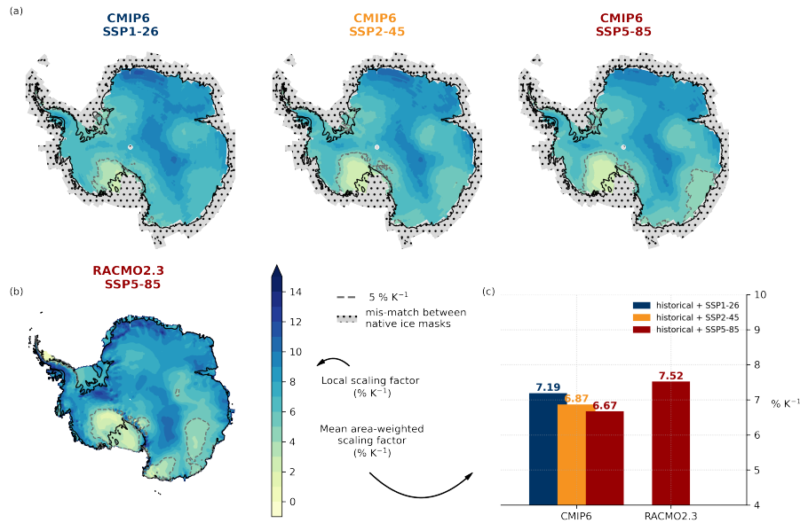
Figure 4. Differences in sensitivity factors across the ice sheet derived from 21st-century projections. Sensitivity factors across the ice sheet derived from 21st century projections. (a) Spatially-resolved sensitivities for the CMIP6 model mean for each SSP scenario. The point-wise temporal regression is based on the period 1950 to 2100 by combining the historical period with the SSP1-26, SSP2-45 and SSP5-85 future scenarios, respectively. (b) Spatially-resolved sensitivities for RACMO2.3 model data, which was forced by CESM2 with SSP5-85 forcing (1950-2100). Dashed lines in maps indicate the 5 % K -1 contour line, which refers to a commonly used sensitivity factor in ice-sheet modelling, such as in Garbe et al. (2020). Hatched regions shows a mis-match between native ice masks of the CMIP6 ensemble which is excluded from the analysis. (c) Comparison of area-weighted mean sensitivities, averaged over the same area of interpolated CMIP6 and RACMO2.3 data.
