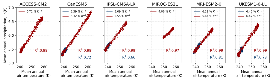
Figure 3. Continent-wide scaling factors for CMIP6 models simulating Antarctic climate change until 2300. Two different approaches for determining the sensitivity factor are used: (a) shows the results when estimating the sensitivity of Antarctic precipitation Red colors refer to temperature from anomalies wrt. shared-socioeconomic pathway SSP5-85 , blue colors refer to 1890-1980 as done in Frieler et al. (2015) shared-socioeconomic pathway SSP1-26 . (b) shows the results when using log-scaled precipitation with absolute temperature estimates in the regression analysis.
