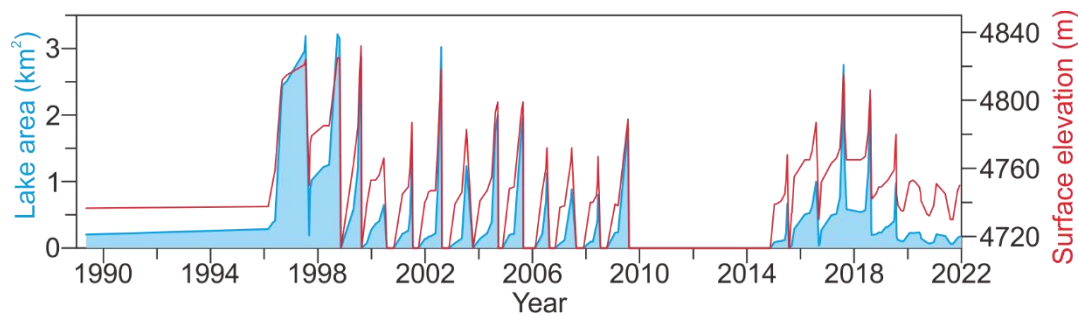
Figure 9: Evolution of ice-dammed lake surface elevation and area from 1989 to 2021.
