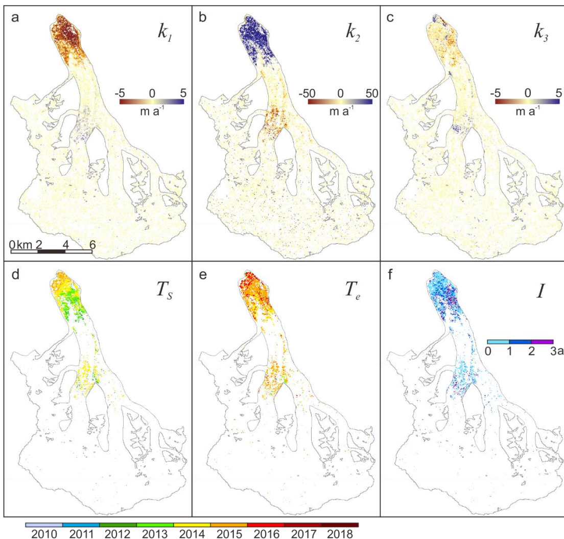
Figure 8: Parameter maps quantifying elevation changes of Kyagar Glacier. Elevation-change rates before, during, and after the surge of each pixel are labeled as k_1 , k_2 , and k_3 . T_s and T_e represent the dates of surge impact initiated and terminated on each pixel. I represents the duration of surge impact.
