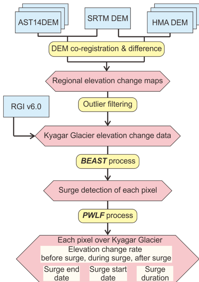
495 Figure 3: Workflow to quantify glacial behaviour using multi-temporal DEMs
