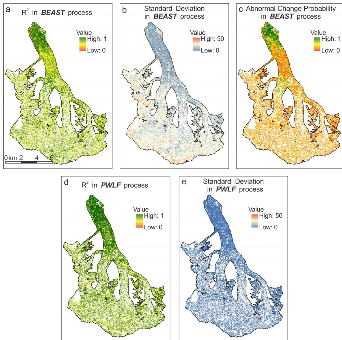
Figure 11: R^2 (a), standard deviation (b), and abnormal change probability (c) in BEAST process; R^2 (d) and standard deviation (e) in PWLF process.
