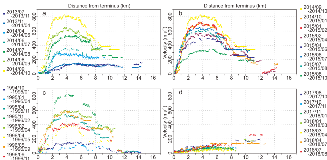
Figure 6: Near monthly velocity profiles along western branch centerline of Kyagar Glacier during two surging periods.
