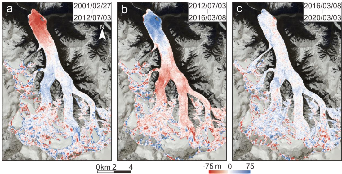
Figure 7: Surface elevation changes of Kyagar Glacier during three periods (a: 2001 - 2012, b: 2012 - 2016, c: 2016 – 2020).
