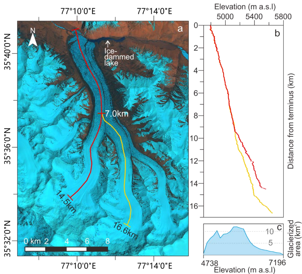
Figure 2: (a) Location of the ice-dammed lake and elevation profiles of the Kyagar Glacier. The background is a sharpened Landsat OLI image (band 6-5-4) acquired on 4 July 2015. (b) Elevation along two centerlines from the terminus; the western branch is shown in red and the central branch shown in yellow. (c) Hypsometry curve of Kyagar Glacier.
