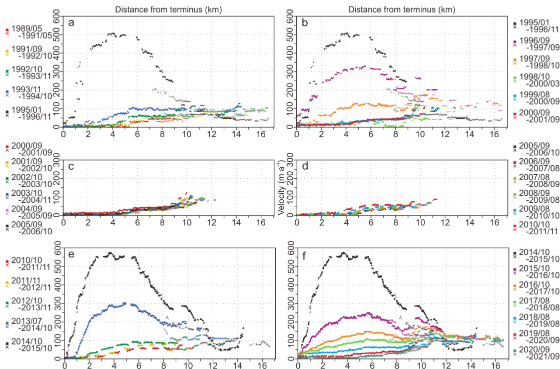
Figure 5: Annual velocity profiles along the western and central branches of Kyagar Glacier from 1989 to 2021. The centerline of the western branch is formed by square dots and the centerline of the central branch is formed by crosses.
