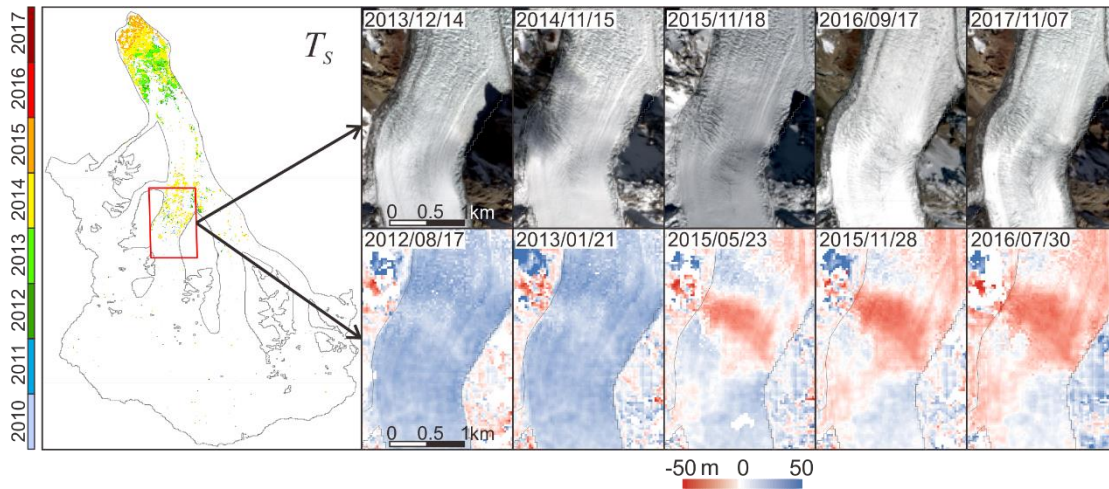
515 Figure 10: Details of Landsat 8 OLI images and elevation changes over reservoir zone. Elevation changes between HMA DEM and SRTM DEM are shown.
