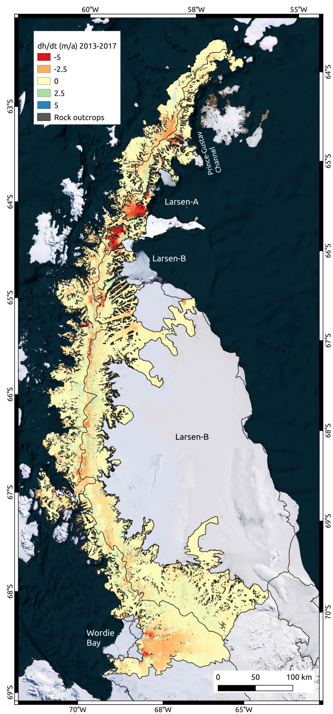
550 Figure 1. Surface elevation changes between austral-winter of 2013 and 2017 derived from TanDEM-X acquisitions for the 25g and 26g basin according to Zwally et al. (2012). Background: © Bing Satellite map by Microsoft; Black polygons: rock-outcrops according to Silva et al. (2020)
