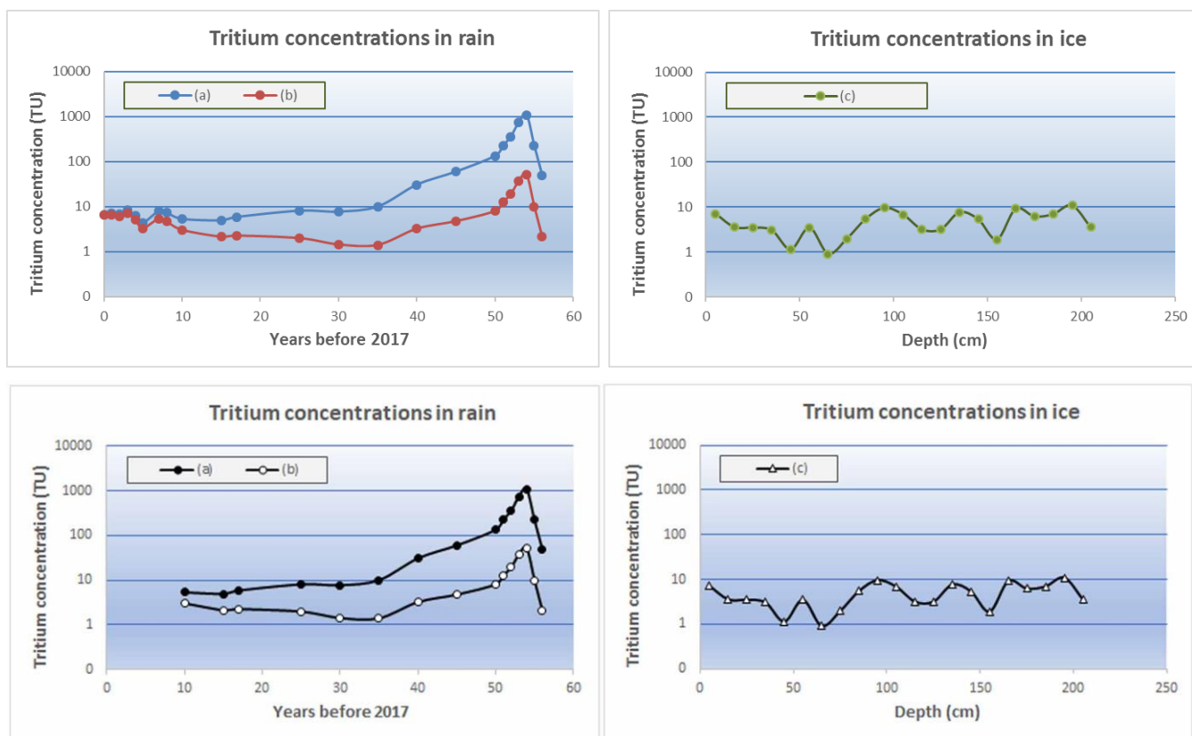
90 Figure 2. Tritium concentration: (a) Annual mean values of tritium in rain samples from various monitoring stations in Greece (GNIP, IAEA, see Fig.1 for the sites of the stations and Table S3 for the coordinates and altitude). (b) Annual mean tritium values of line (a) corrected for decay at the year of ice sampling (2017). (c) Tritium content in ice samples, of odd numbering, with depth, from the Christaki pothole.
