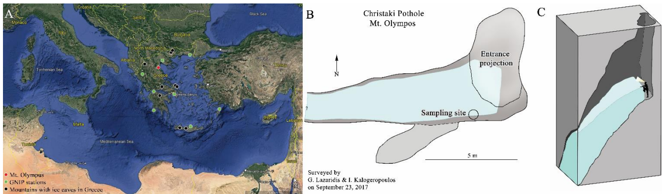
Figure 1. A. Location of Mt. Olympus and the sampled cave Christaki Pothole; other mountains of Greece with ice caves; tritium monitoring stations (GNIP). B. Ground-plan with the sampling site depicted and 3D representation of the cave.
