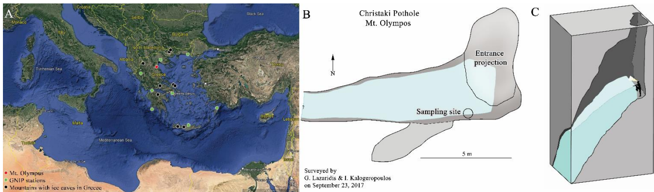
Figure 1. A. Location of Mt. Olympus and the sampled cave Christaki Pothole; other mountains of Greece with ice caves; tritium monitoring stations (GNIP); other mountains of Greece with ice caves (satellite image source from: Google Earth 2022). B. Ground-plan with the sampling site depicted and 3D representation of the cave.
