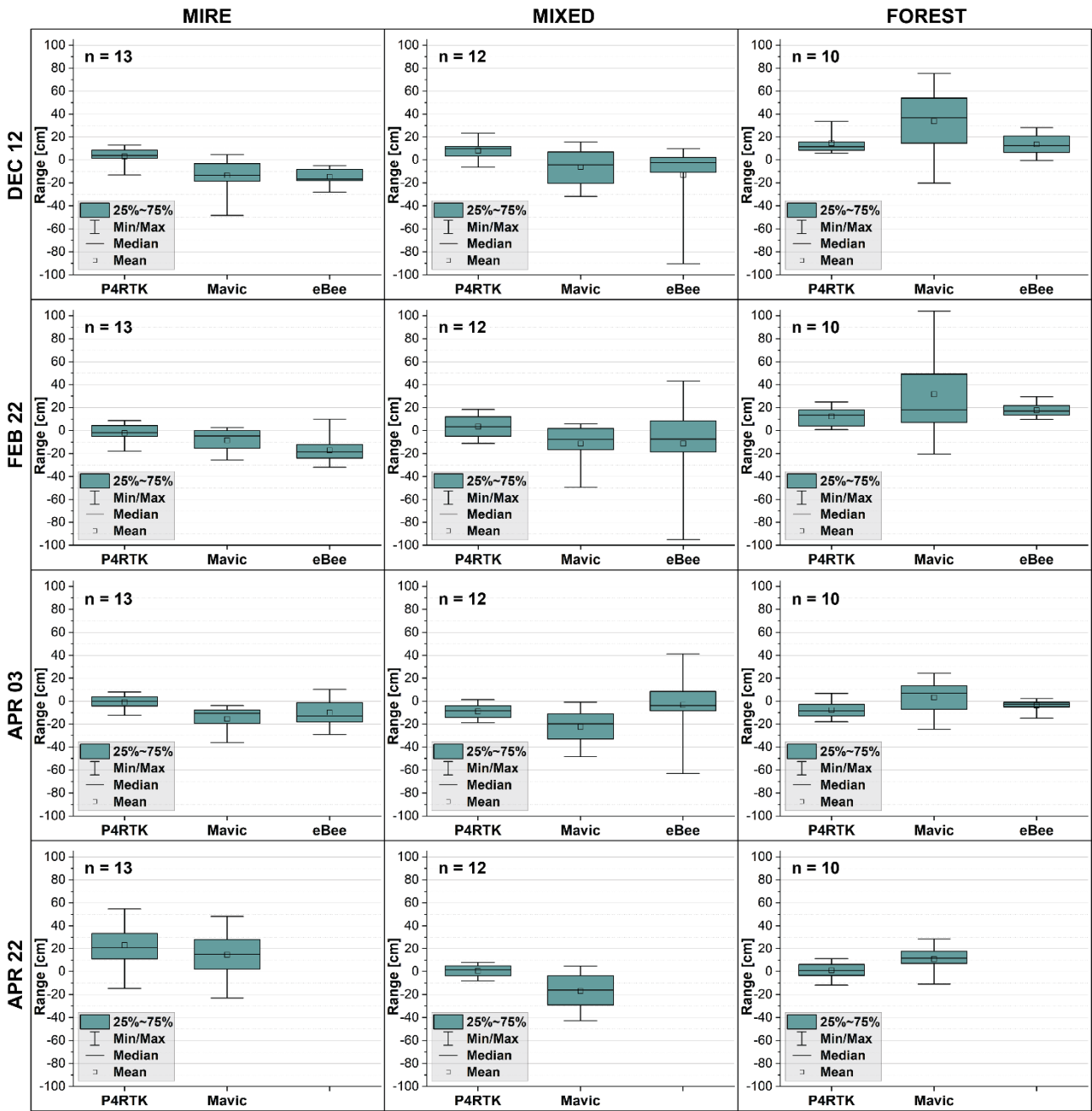
5 Figure S2: The difference between the snow depth DoDs and manual snow line measurements for each subplot and survey date, utilizing UAS-derived snow-free DSM.
