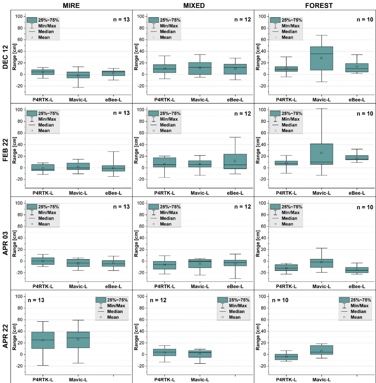
Figure S3: The difference between the snow depth DoDs and manual snow line measurements for each subplot and survey date, utilizing ALS-derived snow-free DSM.
