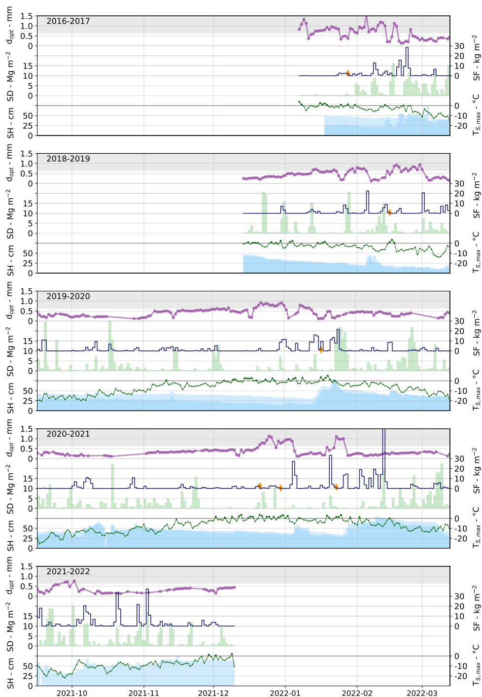
Figure 9. Timeseries of d_{opt} retrieved from Multiband acquisitions at D17 (purple), cumulative daily snowfall (SF, dark blue) cumulative daily snow transport (SD, green), maximum daily surface temperature ( T_{s,max} , dark green) and daily average surface height measured by two SR50 sensors during the first four seasons and only one during the latter (SH, light blue). Days in which rain occurred are marked by orange diamonds. Values of T_{s,max} \geq 0 are outlined by bigger points. The shaded gray area marks d_{opt} > 0.64 mm which is the threshold proposed by Vandecrux et al. (2022) to classify melt conditions.
