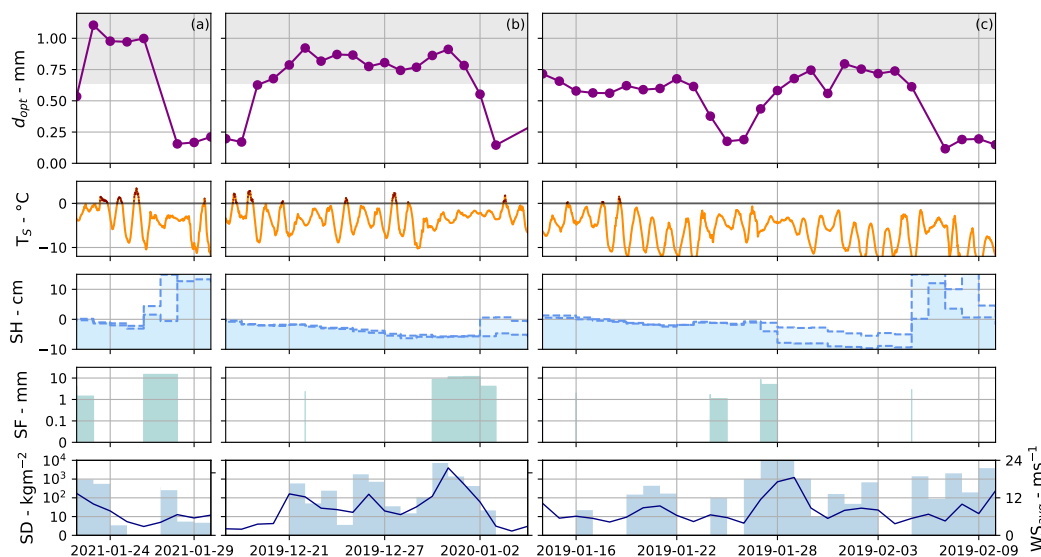
Figure 13. Three examples of timeseries of d_{opt} and meteorological parameters observed during periods with large grains ( d_{opt} \geq 0.64 mm). Shown are the surface temperature ( T_S ), the snow height (SH), the snowfall (SF), snow drift (SD) and wind speed ( WS_{avg} ) intensities. An episode of surface melt during a period of limited snowfall and snow drift (a). A melt event that concurred with snowfall and snow drift (b). An episode o of erosion of the snow surface to a layer with d_{opt} values of a previous melt event, without surface melt (c).
