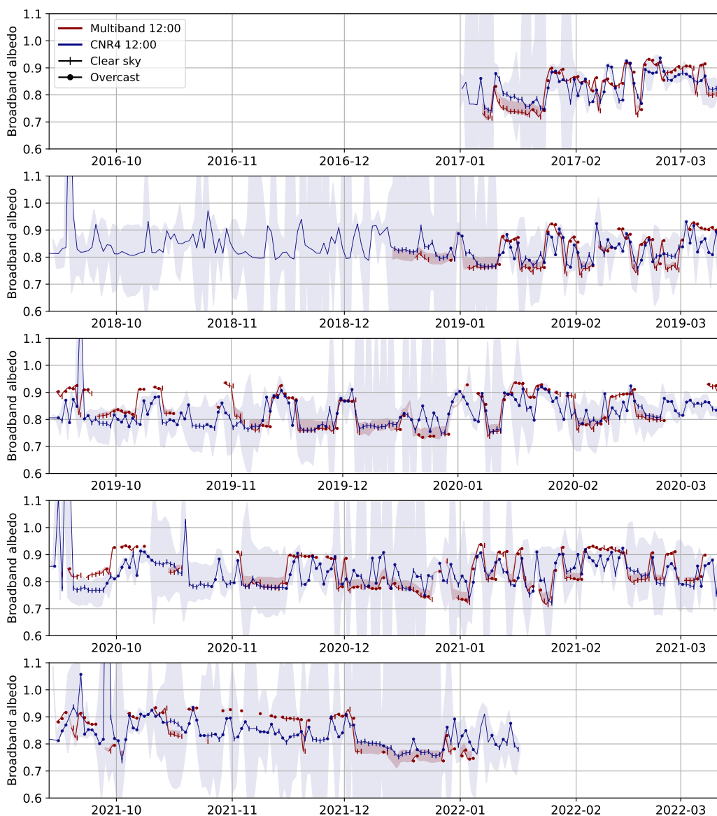
Figure 7. Comparison of the broadband albedo computed from the retrieved d_{opt} (red) and observed by the CNR4 sensor at D17 (blue) at solar noon (solid line). The 10 th and 90 th of the daily albedo measurements is also shown (shaded area).
