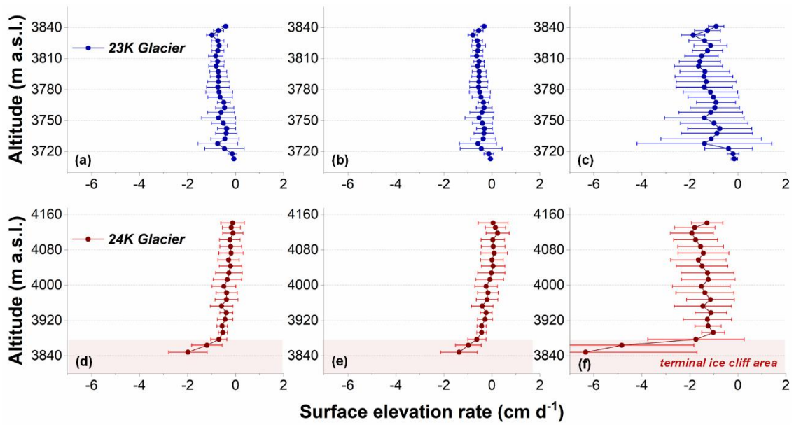
265 Figure 3: Annual average glacier surface elevation rates within 5-m (23K Glacier)/15-m (24K) elevation bands (dots) with the corresponding standard deviations (horizontal error bar) for August 2019-August 2020 (a, d), the cold period (b, e) and the warm period (c, f) across the monitoring area of the two glaciers. The red shadowed sections represent the terminal ice cliff at of the 24K Glacier.
