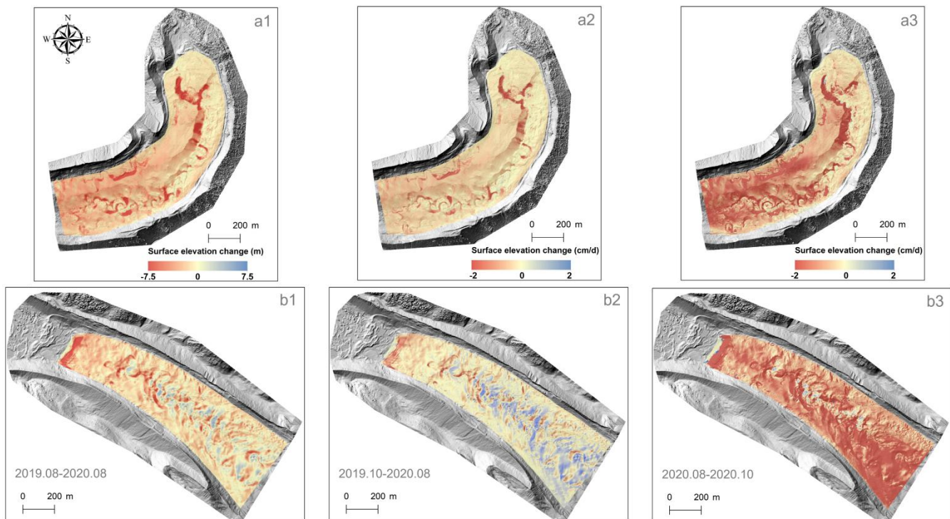
255 Figure 2: Annual surface elevation changes between UAV-derived DEMs for August 2019-August 2020 (a1, b1), the surface elevation change/thinning rates of the cold period (a2, b2) and the warm period (a3, b3) for the 23K Glacier (upper panels) and 24K Glacier (lower panels).
