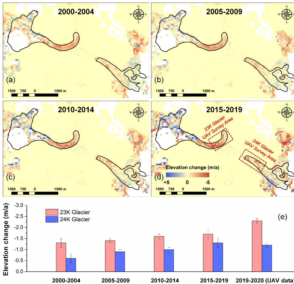
350 Figure 9: Annual surface elevation changes for 2000-2004 (a), 2005-2009 (b), 2010-2014 (c), 2015-2019(d) for the 23K Glacier and 24K Glacier (red dashed rectangular box represents the UAV aerial survey area). Annual surface elevation changes and their uncertainties for both UAV survey domains at different periods (e).
