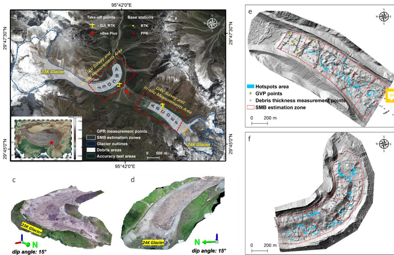
110 Figure 1: (a) Overview of the 23K Glacier and 24K Glacier basin including the UAV survey area, accuracy test areas, in-situ measurement locations (GVPs, GPR, debris thickness measurements), surface mass balance estimation zones (zones A-F) and glacier outlines (background image from Pléiades-1A false-color image from 2021-09-20). © CNES 2021, Distribution Airbus D&S. (b) Geographic location of the study area. (c-d) UAV-derived three-dimensional images for the two glaciers. (e-f) Spatial distribution of the surface mass balance estimation zones of the two glaciers (e: 24K Glacier; f: 23K Glacier), debris thickness measurement points (in June 2019), and distribution of ice cliffs & supraglacial ponds (based on 2020 orthomosaics).
