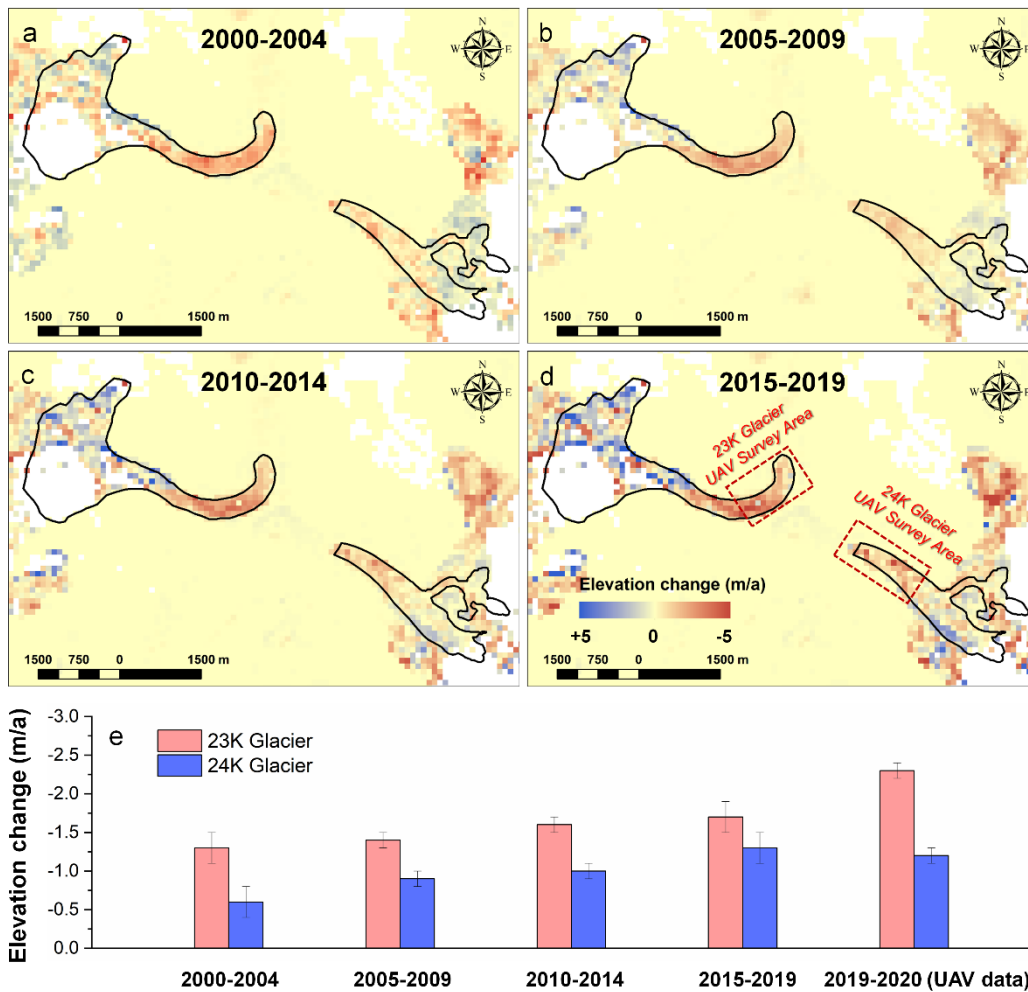
Figure 98: Annual surface elevation changes (Hugonnet et al., 2021) for 2000-2004 (a), 2005-2009 (b), 2010-2014 (c), and 2015-2019 (d) for the 23K Glacier and 24K Glacier (red dashed rectangular box represents the UAV aerial survey area). Annual surface elevation changes and their uncertainties for both UAV survey domains at different periods (e).
