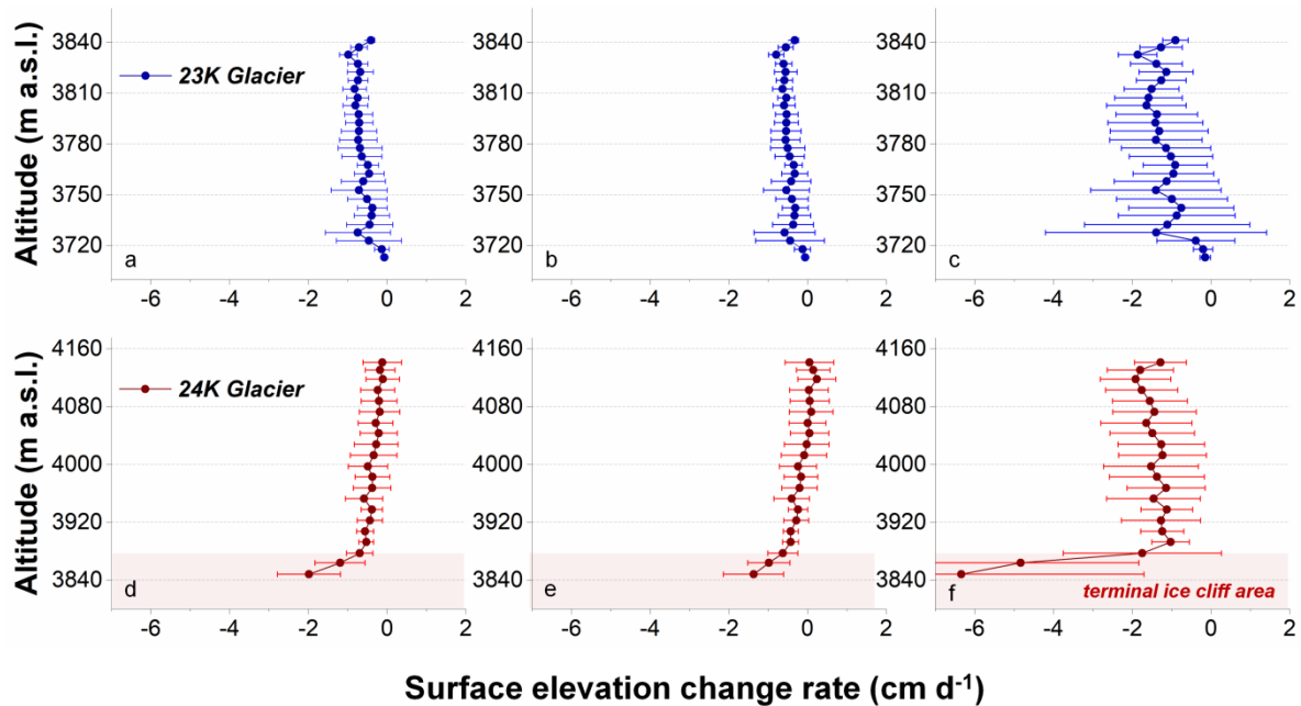
Figure 3: Annual average glacier surface elevation change rates within 5-m (23K Glacier)/15-m (24K Glacier) elevation bands (dots) with the corresponding standard deviations (horizontal error bar) for August 2019-August 2020 (a, d), the cold period (b, e) and the warm period (c, f) across the monitoring area of the two glaciers. The red shadowed sections represent the terminal ice cliff at on of the 24K Glacier. 270
