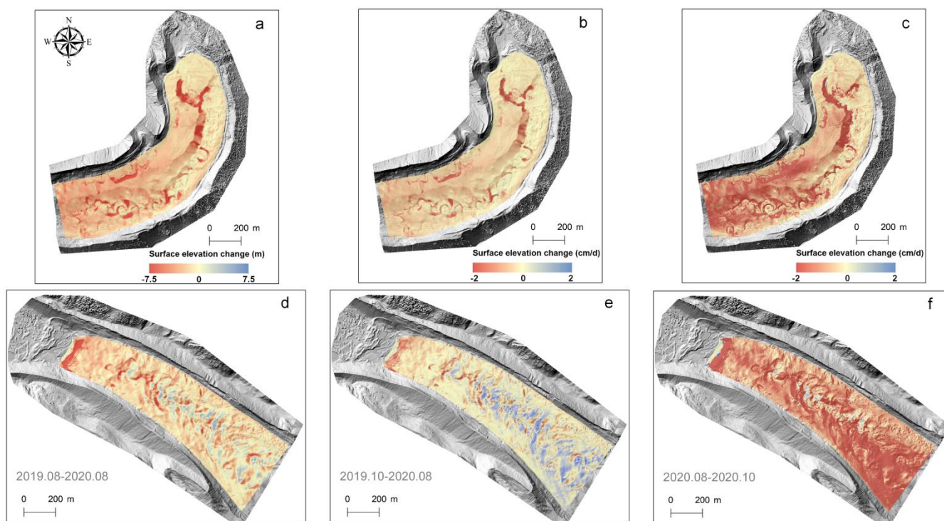
Figure 2. Annual surface elevation changes between UAV-derived DEMs for August 2019-August 2020 (a1, d1), and the surface elevation change/thinning rates for the cold period (b2, e2) and the warm period (c3, f3). Upper panels refer to 23K Glacier and bottom panels refer to 24K Glacier.
