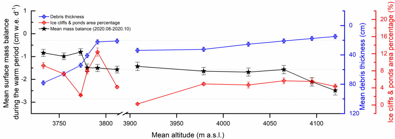
Figure 87: Daily surface mass balance during the warm period (black solid line), the mean debris thickness (blue solid line) and the mean percentage of the ice cliffs and supraglacial ponds area (red solid line) for the individual zones of the two glaciers.
