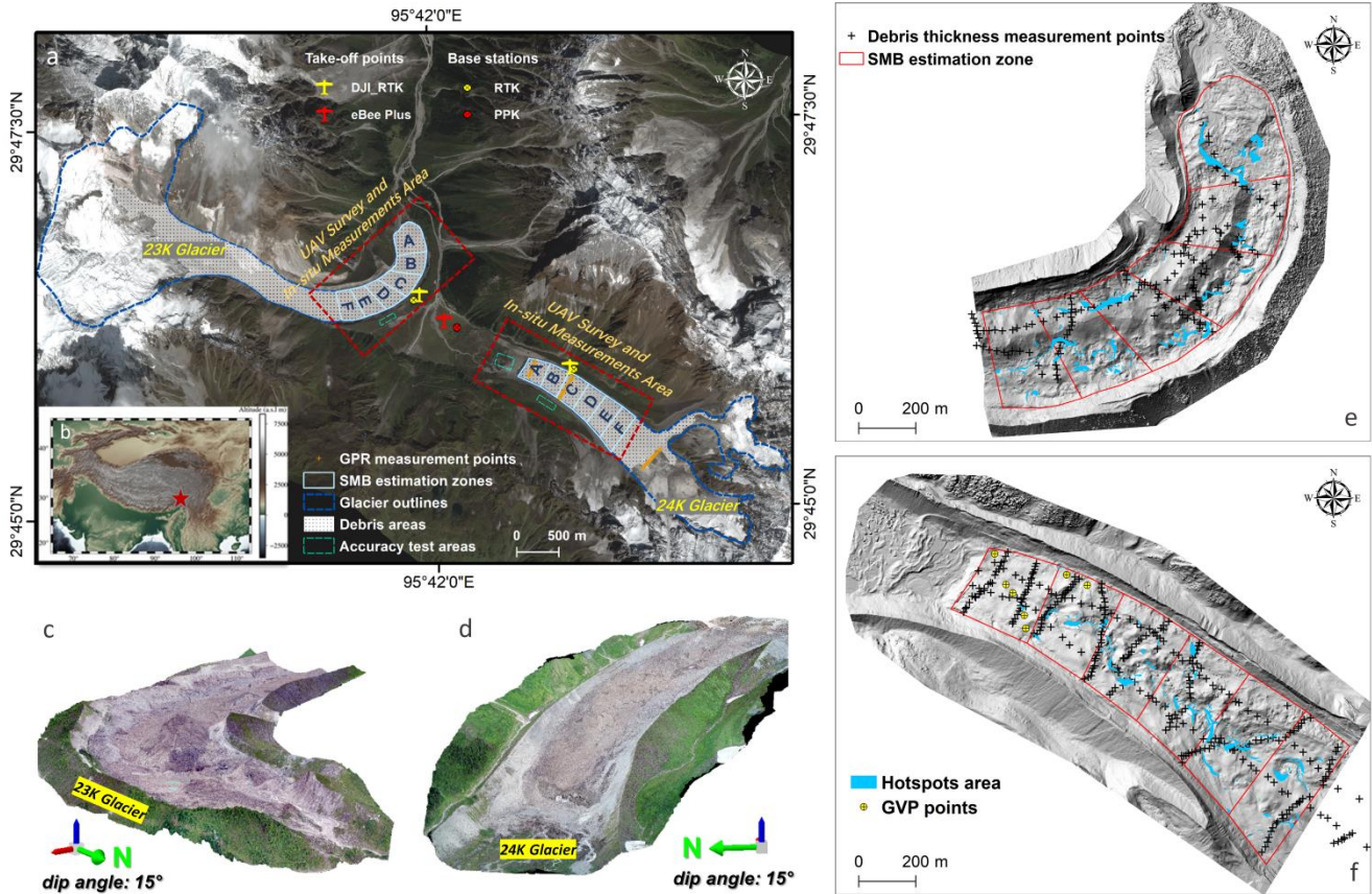
Figure 1: (a) Overview of the 23K Glacier and 24K Glacier basins including the UAV survey areas, accuracy test areas, in-situ measurement locations (ground validation points GVPs, ground penetrating radar GPR, debris thickness measurements), surface mass balance estimation zones (zones A-F) and glacier outlines (background image from Pléiades-1A false-color image from 2021-09-20). © CNES 2021, Distribution Airbus D&S. (b) Geographic location of the study area. (c-d) UAV-derived three-dimensional images for the of the two glaciers. (e-f) Spatial distribution of the surface mass balance estimation zones of the two glaciers (e: 24K Glacier; f: 23K Glacier), debris thickness measurement points (in June 2019), and distribution of ice cliffs and supraglacial ponds (based on 2020 orthomosaics).
