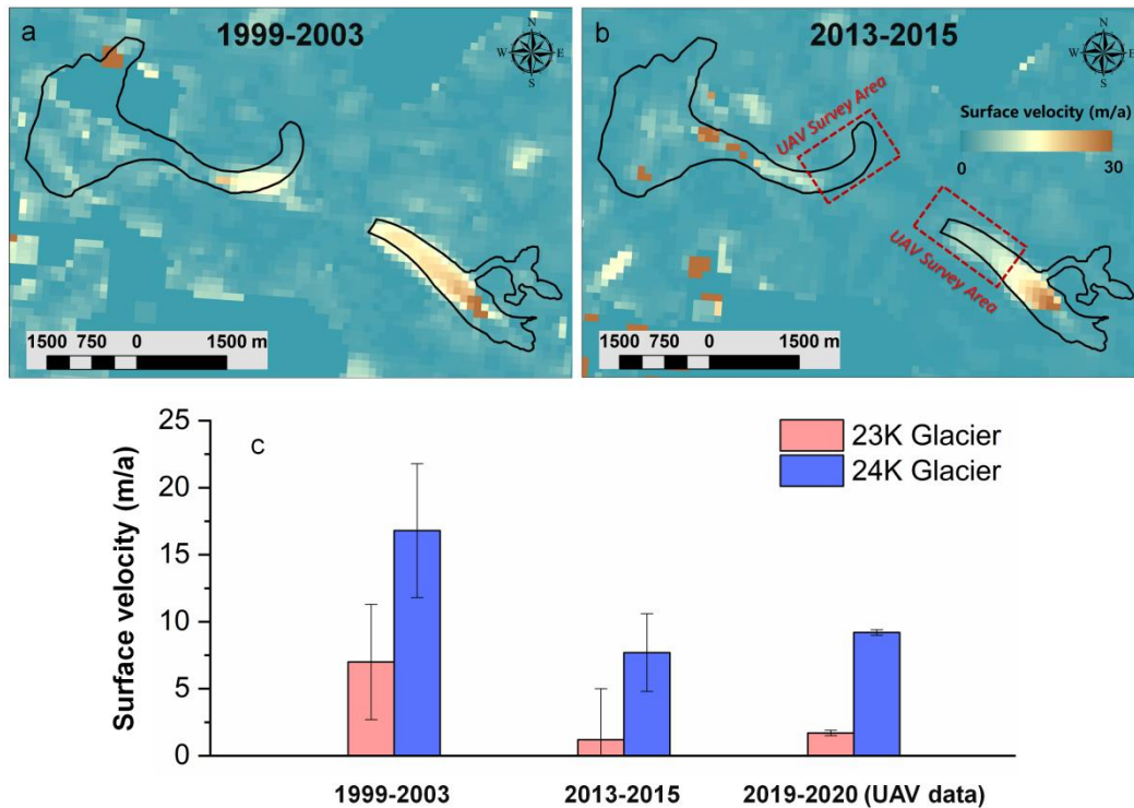
385 Figure 109. Annual surface velocities (Dehecq et al., 2015) for 1999-2003 (a), and 2013-2015 (b) for the 23K Glacier and 24K Glacier (red dashed rectangular boxes represents the UAV aerial survey areas). Annual surface velocities and their uncertainties for both UAV survey domains at different periods (c).
