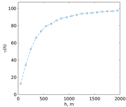
385 Figure 4: Semi-variance of terrain slope of the Tuolumne River Basin above Hetch Hetchy. The slope of the semivariance (not the terrain slope itself) shows a flattening around 500 m, or about the MODIS pixel size.
