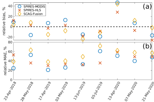
Figure 7: SWE errors by date for the three SWE reconstructions. The relative bias is shown in (a), the relative MAE in (b).
