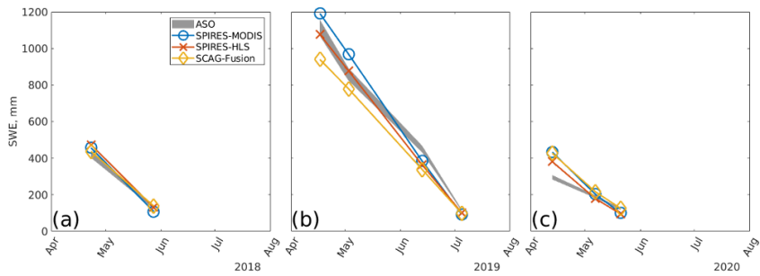
395 Figure 5: Basin-side SWE values by date for the three SWE reconstructions (a-c) compared to Airborne Snow Observatory estimates. Assumed uncertainty in the ASO measurements is \pm 4\% (Section 2.5) and is shaded in gray.
