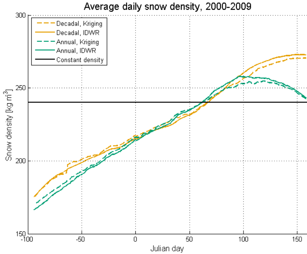
Figure 3: Average daily snow density between 2000-2009 for fourthree different snow density versions. The constant snow density used in SWE retrieval procedure is also shown.
