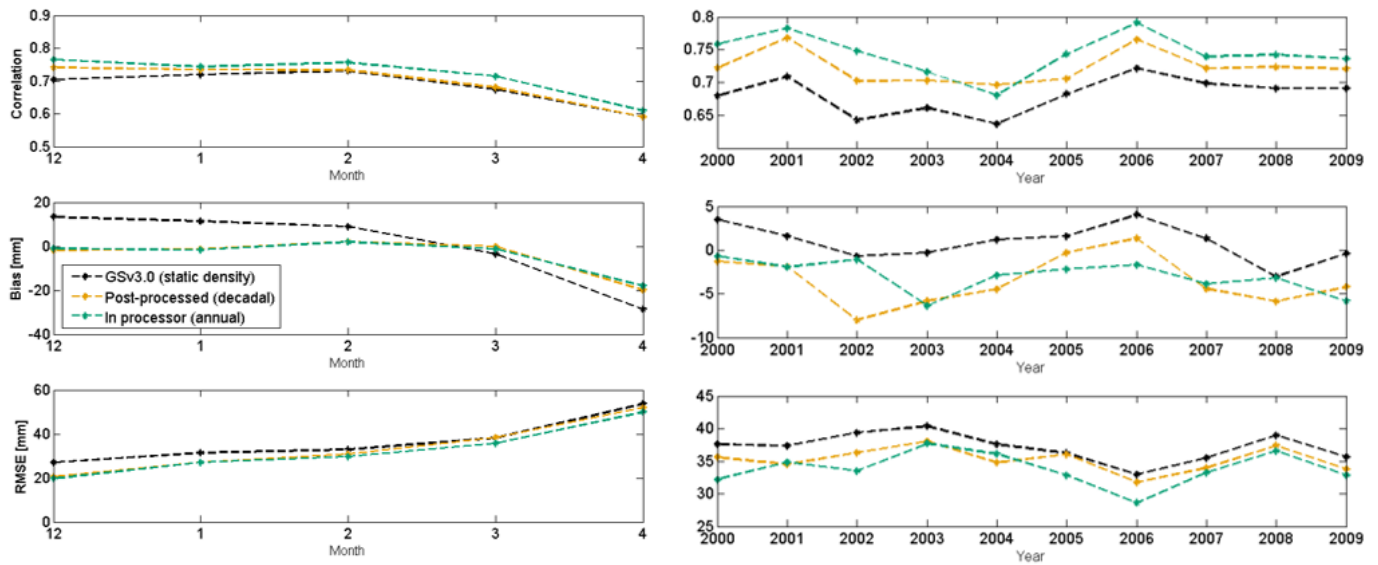
Figure 8: Correlation, bias and RMSE by month (left) and year (right) against validation data. Comparison of GSv3.0, decadal post-processed and IDWR densities in processor SWE value estimates, 2000-2009.
