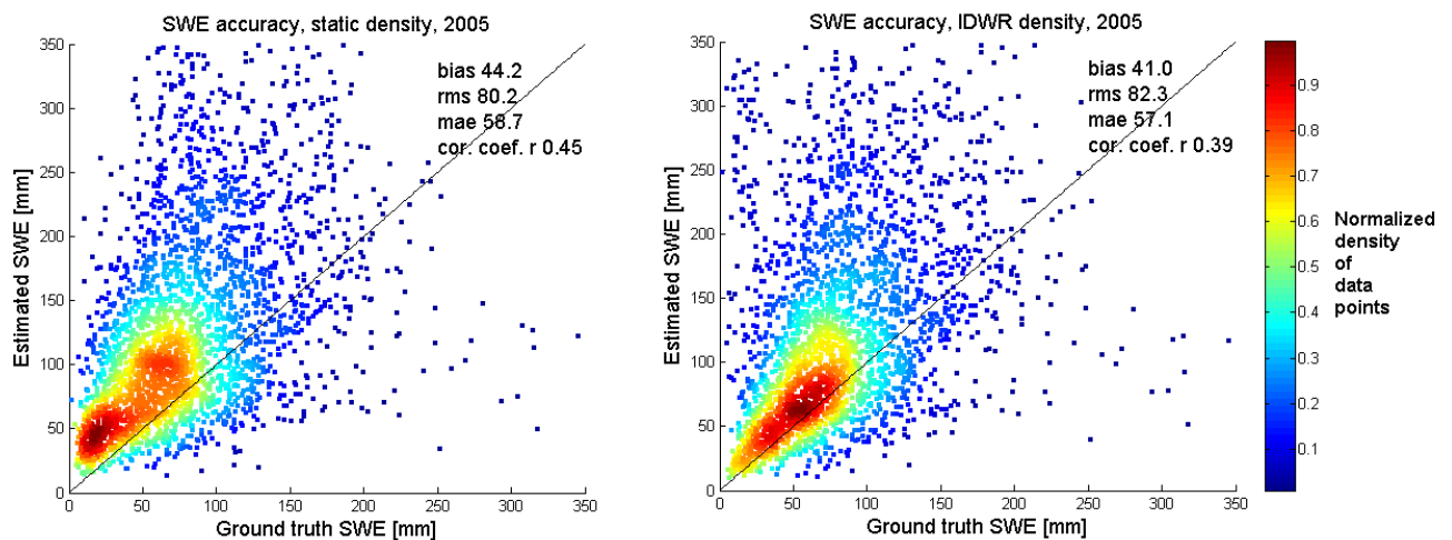
410 Figure 7: Density scatter plots showing the normalized density of scattered points and validation parameters for SWE retrievals without final assimilation with static density (left) and IDWR interpolated dynamic density (right) for 2005.
