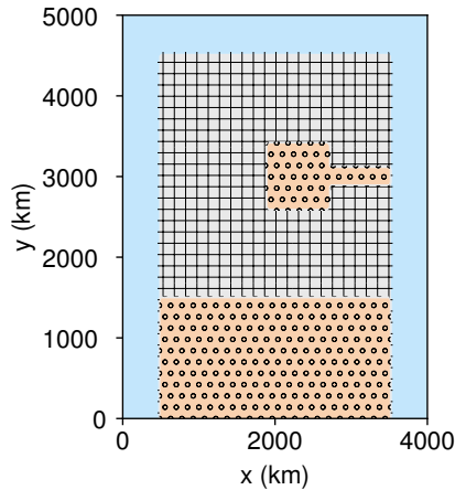
Figure 1. This map of the LISsq bed configuration shows the extent of the domain and the position of the Hudson Bay/Strait and Southern soft beds. Grey hatched regions are hard bedded, beige dotted regions are soft bedded, and blue represents water where ice is ablated.
