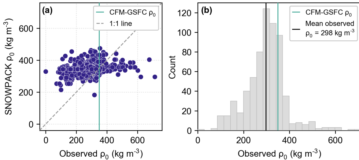
Figure A1. (a) Observed surface density ( \rho_0 ) from SUMup versus SNOWPACK. Since some observations begin farther below the surface, in this figure, observed \rho_0 is defined as the uppermost density measurement that is within 0.1 m from the surface. The SNOWPACK \rho_0 is calculated over the same vertical segment as the SUMup observation. The CFM-GSFC uses a prescribed surface density of 350 \text{ kg m}^{-3} (green vertical line), which falls near many of the observed surface densities. (b) Histogram of observed surface density with the mean represented by the black line. Also plotted is the CFM-GSFC surface density of 350 \text{ kg m}^{-3} .
