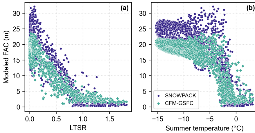
Figure 5. Modeled firm air content (FAC) in SNOWPACK (blue) and the CFM-GSFC (green) as a function of (a) the liquid-to-solid ratio (LTSR, Eq. 6), and (b) the summer 2-m air temperature, all calculated for 1980 through 1995.
