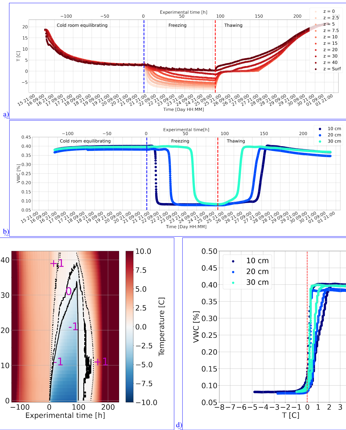
Figure 2. Temperature and volumetric water content monitoring of the experiment : a) Thermal-thermal monitoring, b) volumetric water content monitoring, c) reconstructed 2D temperature column, d) Soil-Freezing-Curves soil freezing curves. Depth of the sensors are in centimeters from the base of the sand layer. Blue dashed line represents the start of the freezing phase, while the red dashed line represents the end of the freezing phase and the beginning of thawing.
