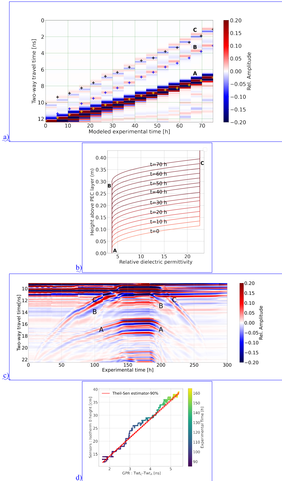
Figure 3. a) Modeled-Simulated radargram with b) permittivity distributions and shown in b) , c) experimental-Experimental radargram displayed with normalized amplitude. Labelled (A), (B) and (C) reflections correspond to the permafrost base, bottom and top of the transition zone. Dots-Crosses in (a) are computed TWT using permittivity distributions in (b) where B and C positions are indicated for the t=0t=65 h. TWT stands for Two-Way travel Time. ed ) TWT C and TWT A difference as a function of isotherm-0°C-C-isotherm height.
