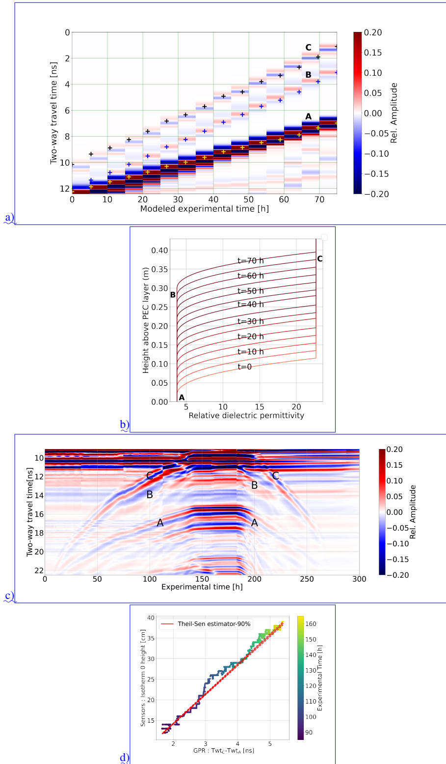
Figure 3. a) Modelled-Simulated radargram with b) permittivity distributions and shown in b) , c) experimental-Experimental radargram displayed with normalized amplitude. Labelled (A), (B) and (C) reflections correspond to the permafrost base, bottom and top of the transition zone. Dots-Crosses in (a) are computed TWT using permittivity distributions in (b) where B and C positions are indicated for the t=0t=65 h. TWT stands for Two-Way travel Time. ed ) TWT C and TWT A difference as a function of isotherm-0°C-C-isotherm height.
