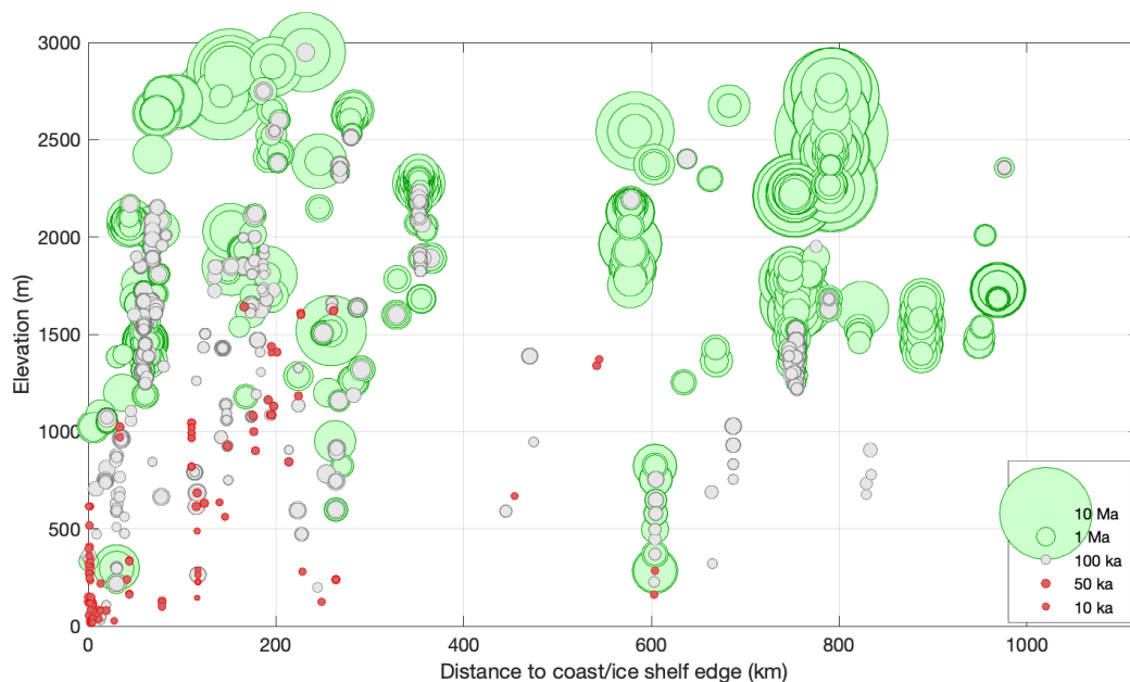
780 Figure 8: Geographic distribution of bedrock exposure ages in Antarctica compiled in the ICE-D:ANTARCTICA database. Each circle represents a bedrock sample with at least one cosmogenic-nuclide measurement, and the size of the circle indicates the apparent exposure age of the surface calculated from that measurement. The “apparent exposure age” is the exposure age of the surface given the assumption that the surface has been exposed continuously for a single period. As the majority of these samples have been repeatedly covered by ice, the apparent exposure age is a minimum limit on the duration of the exposure history recorded by a sample. Green denotes samples with apparent exposure ages > 1 Ma, and red denotes samples with apparent exposure ages < 785 50 ka. Samples that record multimillion-year exposure histories are common at elevations above approximately 1500 m, are ubiquitous at high-elevation, inland locations, and are rare at lower-elevation, coastal sites.
