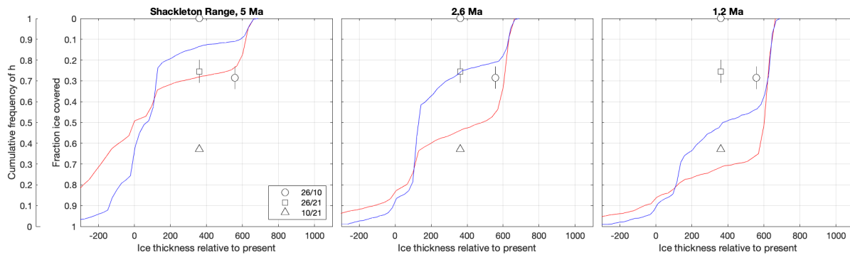
810 Figure 12: Ice cover frequency estimates for the Shackleton Range inferred from paired ^{26}\text{Al}/^{10}\text{Be} data and the inversion code of Spector et al. (2020), compared with sensitized and desensitized model CDFs for the same site. The model CDFs are referenced to the ice thickness in the final model time step and no model-data alignment has been attempted. The data are described in Fogwill et al. (2004), Hein et al. (2011, 2014), Sugden et al. (2014). Sample elevations relative to the present ice margin are taken directly from the source publications without additional examination.
