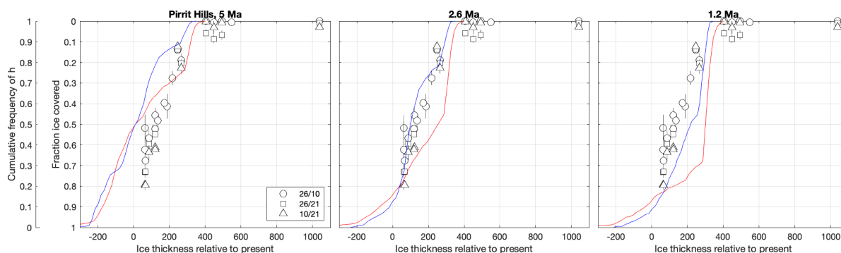
790 Figure 9: Ice cover frequency estimates derived from cosmogenic-nuclide data at the Pirrit Hills (Spector et al., 2020) compared with ice thickness CDFs for sensitized (red) and desensitized (blue) model simulations over different time periods. In this figure, model CDFs are vertically registered with data such that the “present ice thickness” is the ice thickness in the model grid cell containing the Pirrit Hills in the final time step of the model. The ice cover frequency estimates are computed from data in Spector et al. (2020) and the ICE-D: ANTARCTICA database, using the MATLAB code of Spector et al. (2020).
