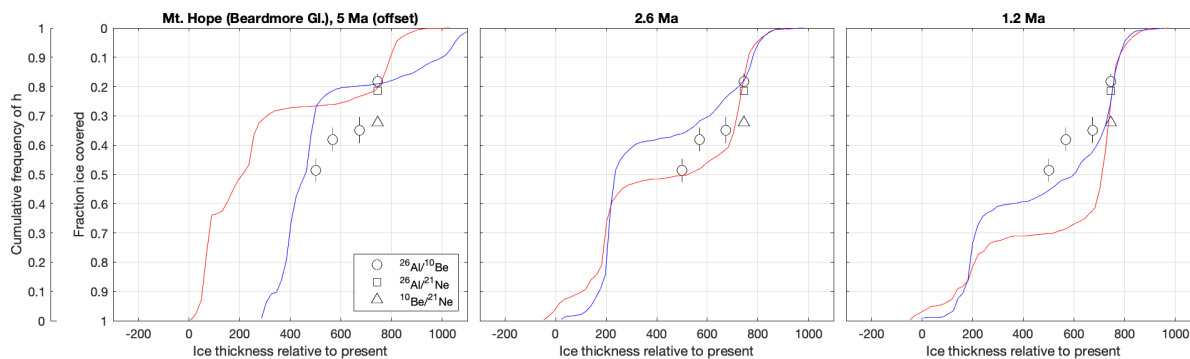
815 Figure 13: Ice cover frequency estimates for Mt. Hope, inferred from multiple-nuclide data and the inversion code of Spector et al. (2020), compared with sensitized and desensitized model CDFs for a site in the centre of the model Beardmore Glacier at a position near Mt. Hope (because of the coarse model resolution, the model Beardmore Glacier is not in exactly the same location as the real glacier, so we have chosen an equivalent site in the model). As in Figs. 10 and 11, model CDFs have been offset to align observational and model CDFs at the 80th percentile elevation. The data from Mt. Hope are unpublished measurements archived in the ICE-D:ANTARCTICA database.
