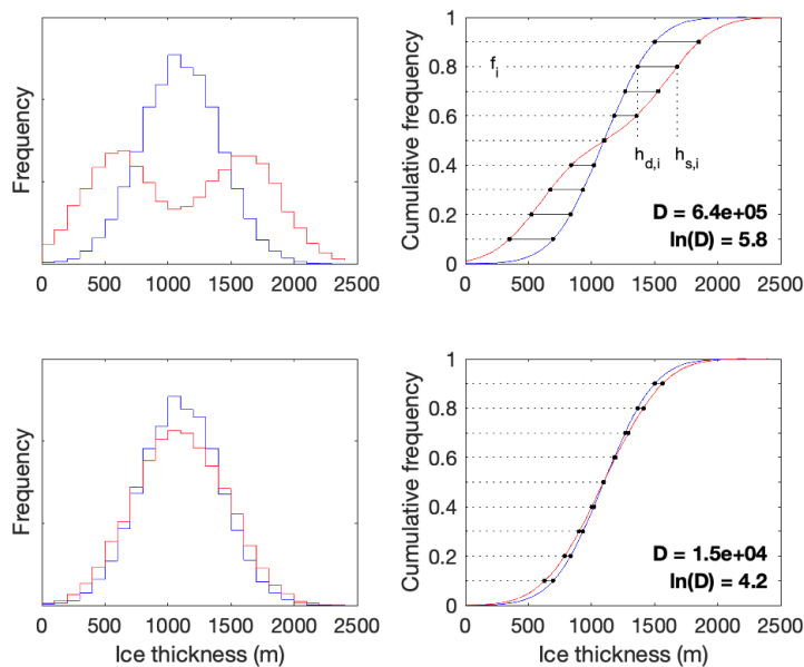
Figure 5: Method of quantifying difference between model ice thickness CDFs at a site. Red and blue curves are hypothetical output from desensitized (blue) and sensitized (red) ice sheet model runs, displayed as histograms (left) and CDFs (right). The difference between two CDFs is quantified by sampling the difference between the elevations of the two CDFs at evenly spaced values of cumulative frequency (the black line segments in right panels), and computing a total CDF difference metric ‘D’ (see text) as the sum of squares of the individual differences. As D ranges over several orders of magnitude, for convenience we plot \ln(D) in subsequent figures.
