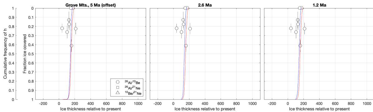
800 Figure 11: Ice cover frequency estimates for the Grove Mountains in East Antarctica inferred from paired ^{26}\text{Al}/^{10}\text{Be} data and the inversion code of Spector et al. (2020), compared with sensitized and desensitized model CDFs for the same site. As in Fig. 10, model CDFs have been offset in elevation to align them with the centre of the group of data points. Data are described in Huang et al. (2008), Lilly (2008), Li et al. (2009), Kong et al. (2010), Liu et al. (201), Lilly et al. (2010). Sample elevations relative to the present ice margin are taken directly from the source publications without additional examination.
