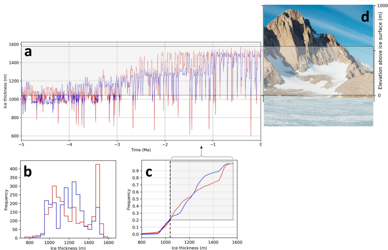
745 Figure 4: Example ice thickness change history at Mt. Tidd, one of the nunataks comprising the Pirrit Hills, in the middle of the West Antarctic Ice Sheet (location shown in Fig. 7e). (a) The sensitized model (red) displays larger variation in ice thickness and is more likely to occupy extreme values, whereas the desensitized model (blue) is more likely to occupy intermediate values. The resulting ice thickness histograms (b) and cumulative frequency distributions (CDFs) (c) are therefore distinct. (d) Photo of Mt. Tidd, aligned on the same yaxis as (a). Grey shading in (b,c,d) denotes the elevation range that is exposed above the present ice surface (so data can be collected) and where ice cover frequency reconstructions could distinguish between sensitized (red) and desensitized (blue) model behaviour. Dashed black line in (b) denotes the approximate modern ice thickness at this site. The dashed black line in (b) represents the modern ice thickness and is chosen to approximately align the range of ice thickness in the model 750 simulation with that inferred from geologic evidence.
