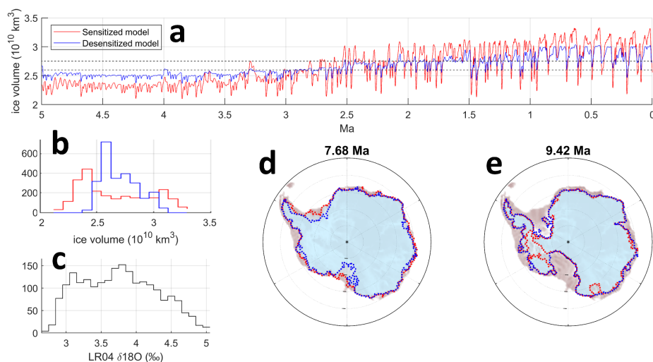
735 Figure 3: (a) Grounded ice volume throughout the Plio-Pleistocene produced by the sensitized (red) and desensitized (blue) simulations. Dashed lines represent the modern ice volume and an approximate WAIS collapse threshold, respectively. (b) Histogram of ice volume fluctuations shown in (a). (c) Histogram of the \delta^{18}\text{O} time series (Lisiecki and Raymo, 2005) used to force the model simulations. (d,e) Snapshots of sensitized (red) vs desensitized (blue) grounded ice configurations at two representative times; the sensitized ice sheet is bigger during glacials (d) and smaller during interglacials (e).
