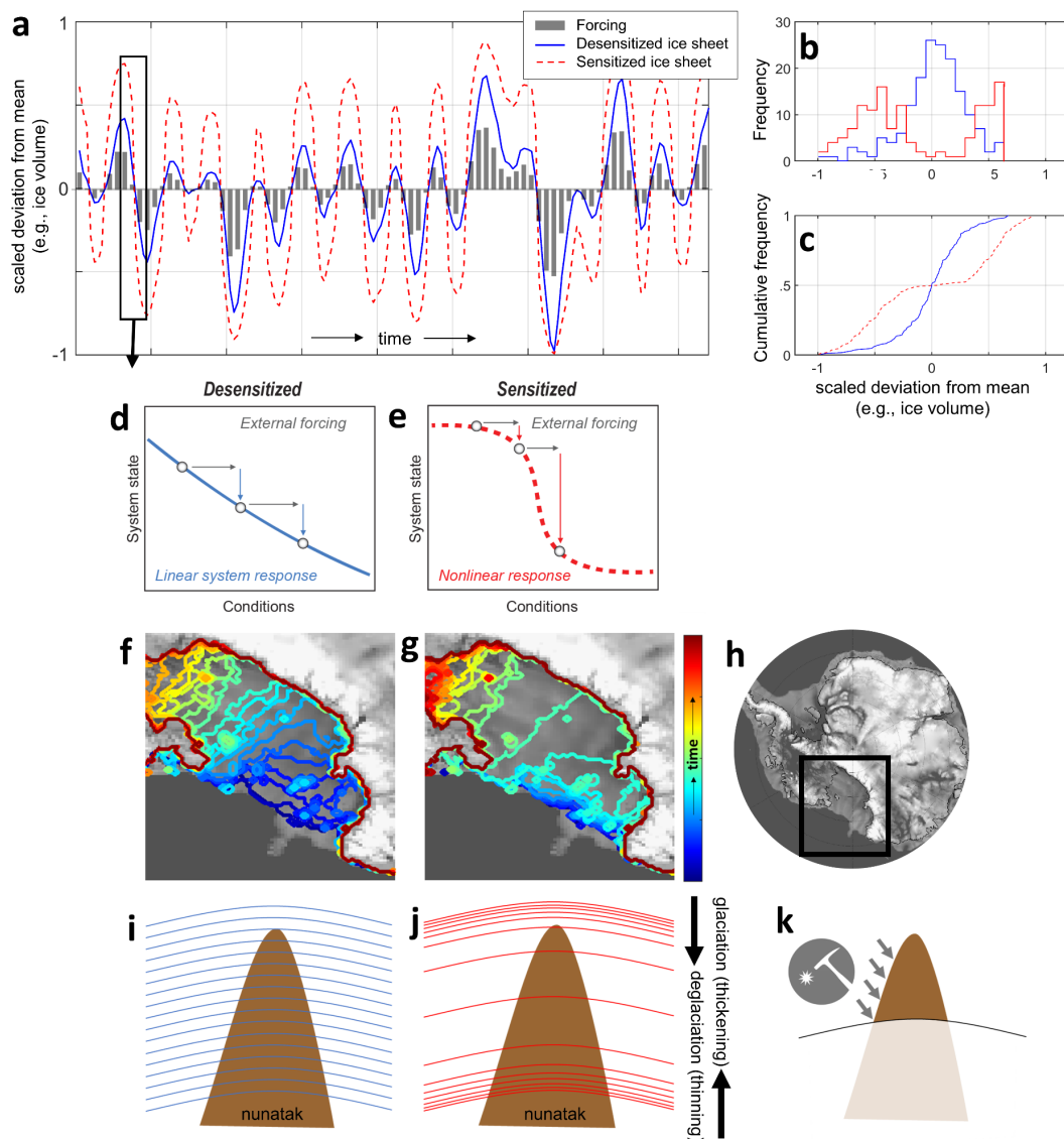
720 Figure 2: Conceptual illustration of sensitized versus desensitized ice sheet behaviour. (a) For a given forcing (black bars), a desensitized ice sheet responds linearly (blue line) while a sensitized ice sheet responds nonlinearly (dashed red). The y-axis is shown as scaled deviation from the mean, so that ice volumes are normalized between -1 and 1 in this hypothetical illustration. In this 725 example, the hypothetical dataset is non-linearized using a simple exponential transformation. (b) Frequency and (c) cumulative frequency distributions of ice volumes for the sensitized and desensitized models illustrated in (a). (d,e) Conceptual schematics of linear vs nonlinear responses to a given forcing (cf. Scheffer et al., 2009), leading to the differential ice sheet behaviour illustrated in (f,g). (f,g) Characteristic grounding-line behaviour in the Ross Sea, Antarctica; location shown as black box in (h). (f) Desensitized ice sheet behaviour is characterized by steady grounding line recession throughout a deglaciation, while (g) a sensitized ice sheet is 730 more susceptible to runaway positive feedback mechanisms that cause the grounding line to rapidly jump from maximum to minimum states. (h) Continental bed topography (Fretwell et al., 2013) with a modern grounding line shown for context. (i,j) Characteristic ice thinning patterns for desensitized (i) and sensitized (j) ice sheet behaviour; coloured lines denote hypothetical ice surfaces as the ice sheet deflates and regrows over a nunatak, where cosmogenic nuclide data could be sampled along the modern exposed surface (k).
