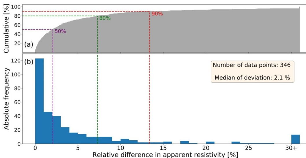
295 Figure 5: Histogram of the percentage deviation of the measured apparent resistivity for pairwise comparison between quadrupole measurements collected with the new textile electrodes and conventional steel pike electrodes: (a) cumulative distribution and (b) absolute frequency (b). The dashed lines show defined portions of all data pairs with the corresponding limit of deviation in apparent resistivity.
