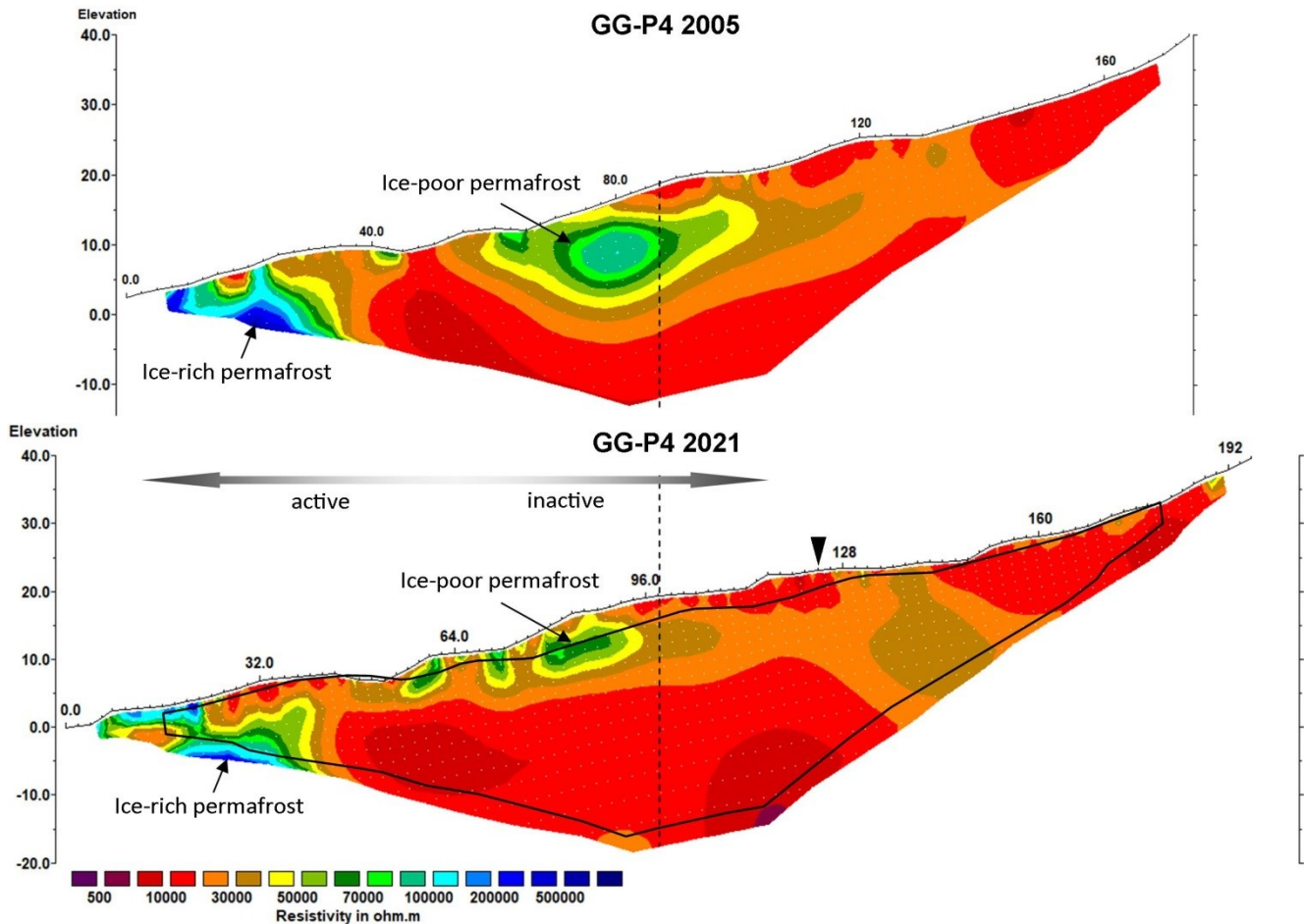
360 Figure 8: Tomograms of the historical (2005) and the repeated (2021) profile GG-P4 on the Gianda Grisca rock glacier. The dashed line indicates the common centre point. The point of intersection with tomogram GG-P1 is indicated by a black triangle. The black line displays the outline of the historical tomogram.
