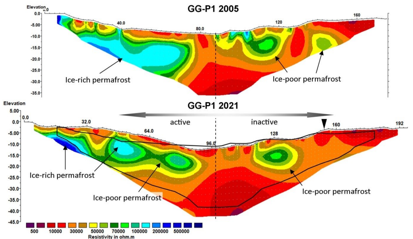
345 Figure 7: Tomograms of the historical (2005) and the repeated (2021) profile GG-P1 on the Gianda Grisca rock glacier. The dashed line indicates the common centre point. The point of intersection with tomogram GG-P4 is indicated by the black triangle. The black line indicates the outline of the historical tomogram.
