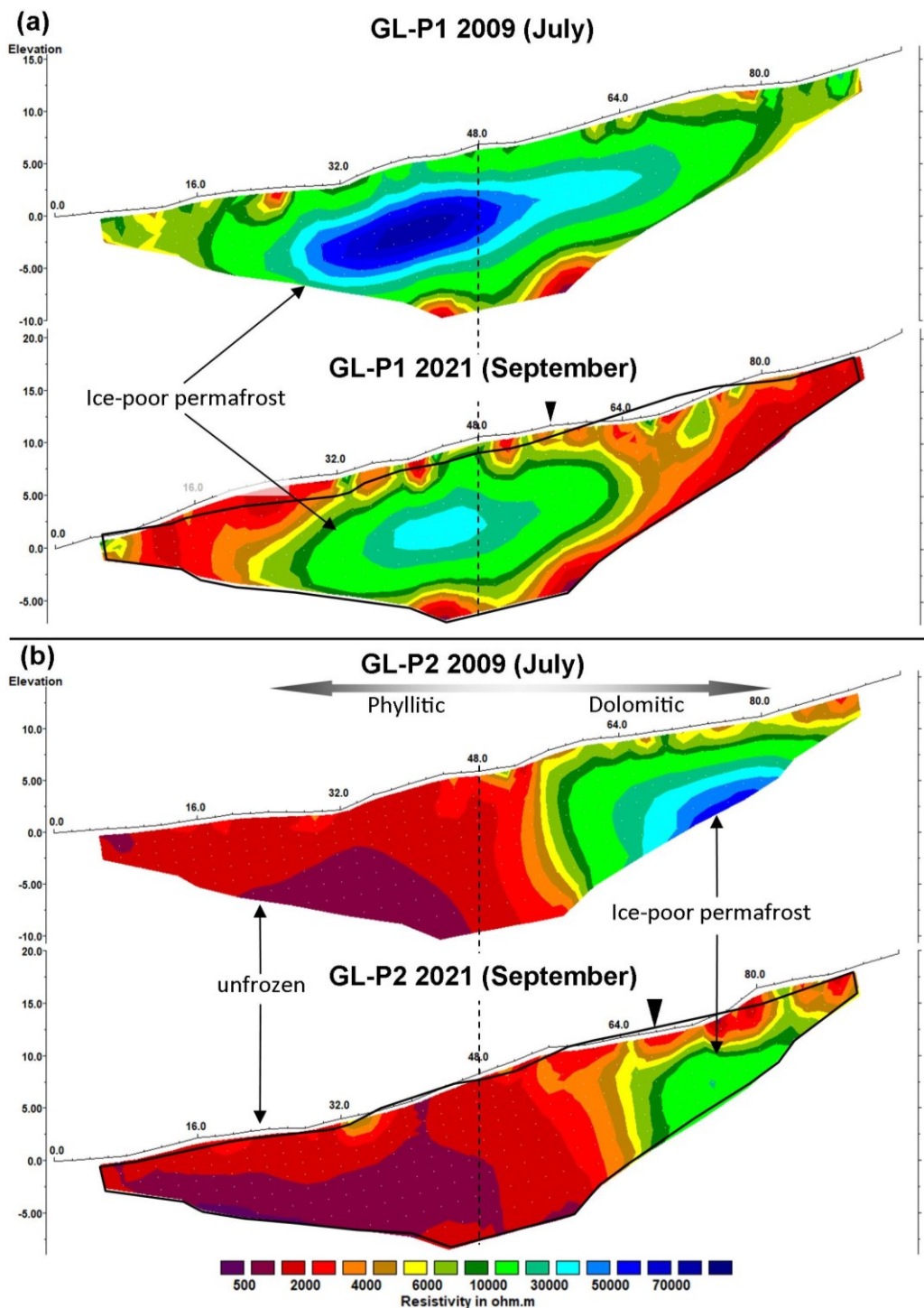
Figure 11: Tomograms of the historical (July 2009) and the repeated (September 2021) profiles GL-P1 and GL-P2 in the Glatzbach catchment. The dashed lines indicate the common centre points. The points of intersection of the two perpendicular profiles are indicated by black triangles. The black lines display the outlines of the historical tomograms.
