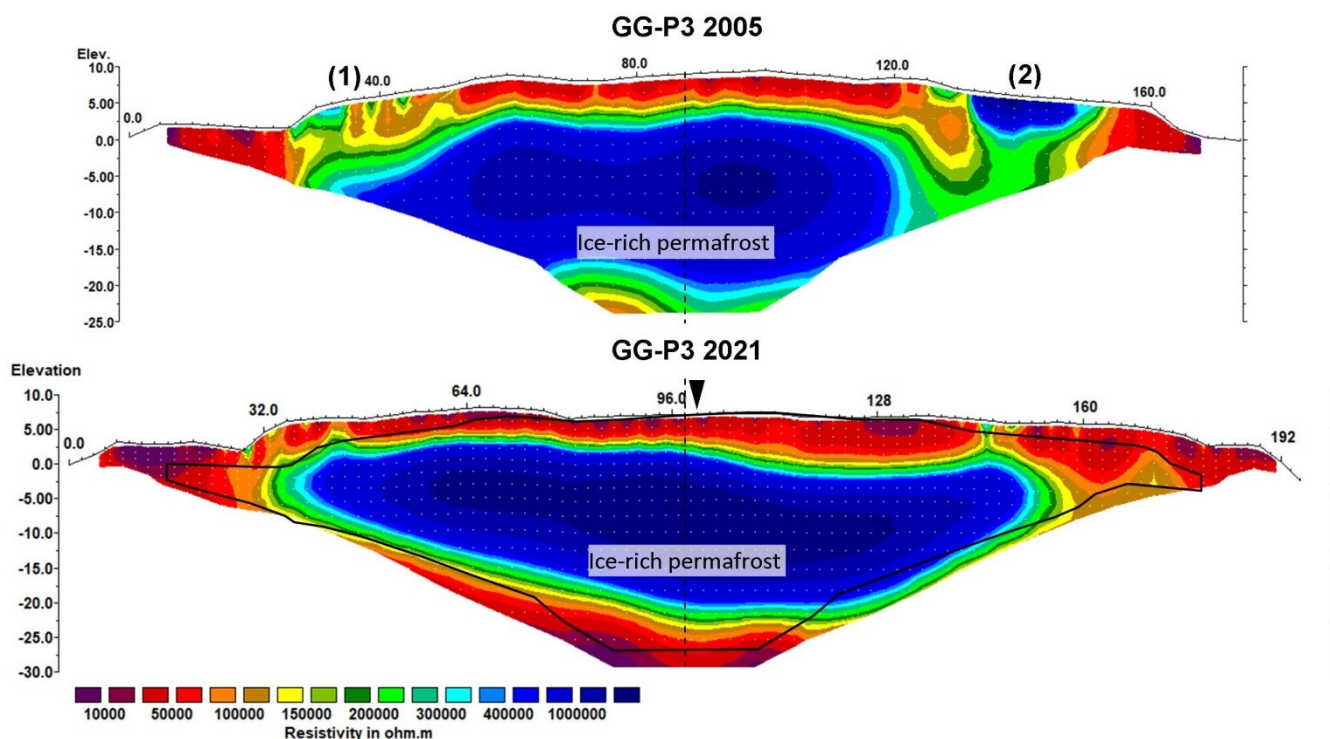
390 Figure 10: Tomograms of the historical (2005) and the repeated (2021) profile GG-P3 on the Gianda Grischa rock glacier. The dashed line indicates the common centre point. The point of intersection with tomogram GG-P2 is indicated by a black triangle. The black line displays the outline of the historical tomogram.
