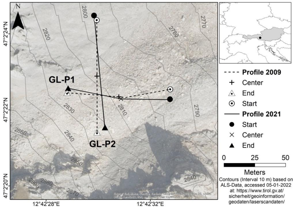
160 Figure 3: Location of the historical (2009, dashed lines) and the repeated (2021, solid lines) ERT profiles on the block field in the Glatzbach catchment, Tauern range.
