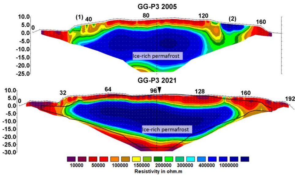
415 Figure 10: Tomograms of the historical (2005) and the repeated (2021) profile GG-P3 on the Gianda Grisca rock glacier. The dashed line indicates the common centre point. The point of intersection with tomogram GG-P2 is indicated by a black triangle. The black line displays the outline of the historical tomogram.
