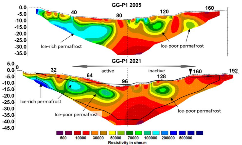
Figure 7: Tomograms of the historical (2005) and the repeated (2021) profile GG-P1 on the Gianda Grischa rock glacier. The dashed line indicates the common centre point. The point of intersection with tomogram GG-P4 is indicated by the black triangle. The black line indicates the outline of the historical tomogram.
