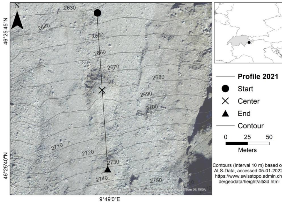
Figure 1: Location of the ERT profile on the protalus rock glacier in the Murtèl catchment, Upper Engadin. The repeated profile (2021) is based on the blocks marked in the field in 2011; therefore the location of the new and the historical profiles are identical.
