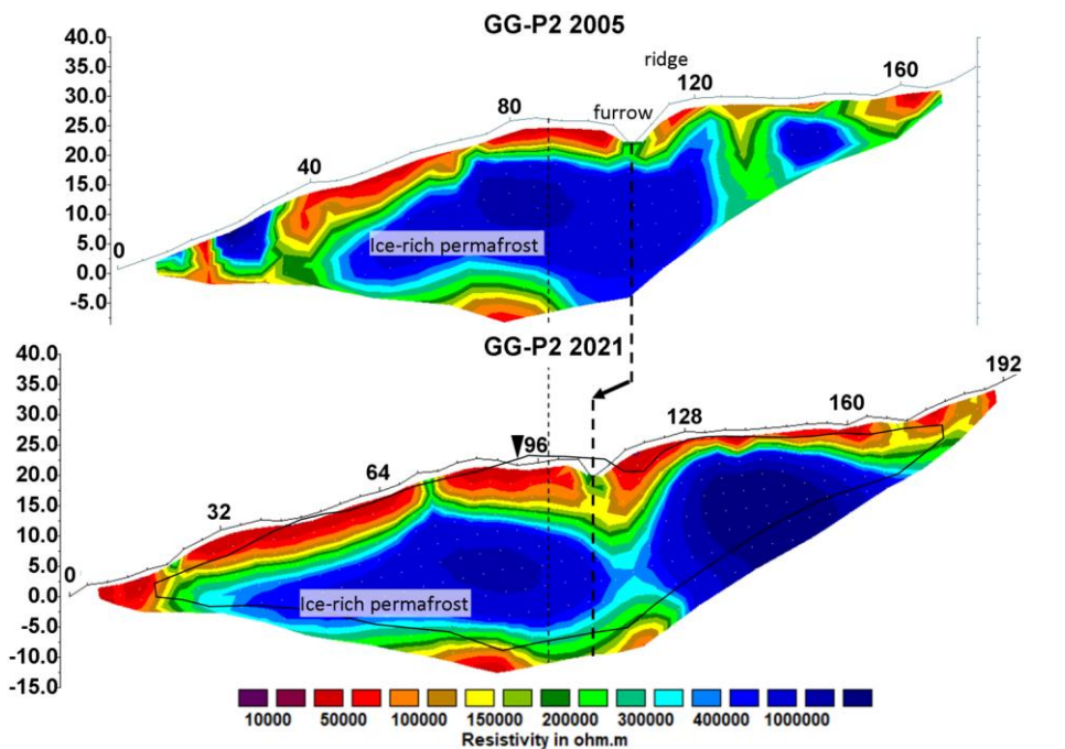
Figure 9: Tomograms of the historical (2005) and the repeated (2021) profile GG-P2 on the Gianda Grisca rock glacier. The thin black dashed line indicates the common centre point. The point of intersection with tomogram GG-P3 is given by a black triangle. The thick dashed line and the arrow highlight the observed down-gradient shift of furrow. The black line displays the outline of the historical tomogram.
