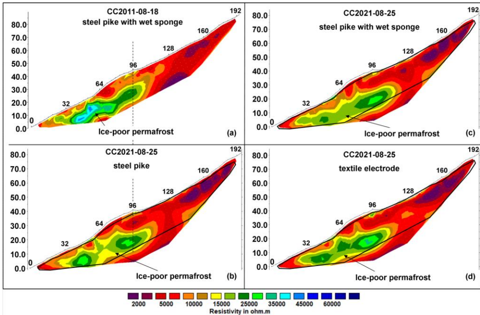
Figure 6: Tomograms of the historical (2011) and the repeated (2021) profiles in the Corvatsch catchment: (a) historical profile; (b) repeated profile measured with steel pikes; (c) repeated profile measured with steel pikes and wet sponges; (d) repeated profile measured with textile electrodes. The black lines in (b) to (d) indicate the outline of the historical tomogram. The vertical axes display the relative elevation in meters.
