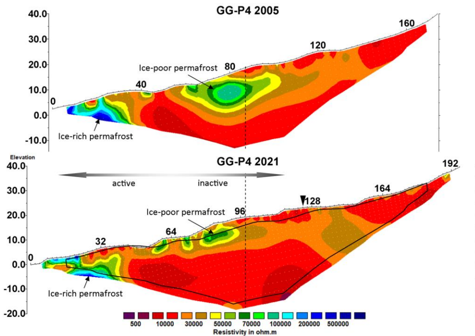
385 Figure 8: Tomograms of the historical (2005) and the repeated (2021) profile GG-P4 on the Gianda Grisca rock glacier. The dashed line indicates the common centre point. The point of intersection with tomogram GG-P1 is indicated by a black triangle. The black line displays the outline of the historical tomogram.
