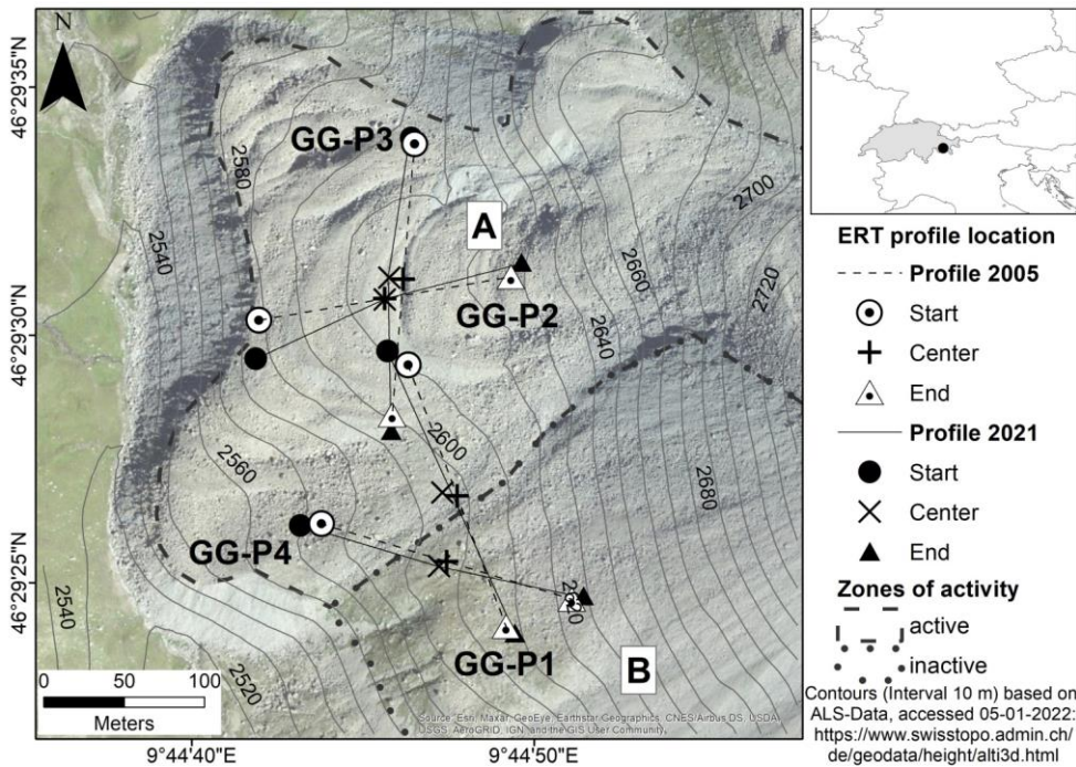
Figure 2: Location of the historical (2005, dashed line) and the repeated (2021, solid line) ERT profiles on the Gianda Grisca rock glacier, Upper Engadin. The status of activity (A = active; B = inactive) is based on this study and Frauenfelder et al. (2008). The area around A is characterized by furrows and ridges and hosts profiles P2 and P3.
