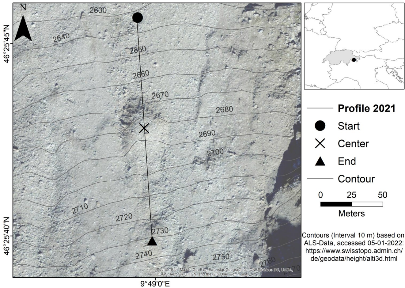
Figure 1: Location of the ERT profile on the protaustalus derived rock glacier in the Murtèl catchment, Upper Engadin. The repeated profile (2021) is based on the blocks marked in the field in 2011; therefore the location of the new and the historical profiles are identical.
