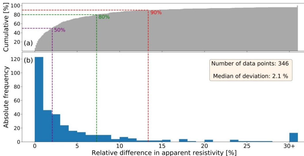
330 Figure 5: Histogram of the percentage deviation of the measured apparent resistivity for pairwise comparison between quadrupole measurements collected with the new textile electrodes and conventional steel pike electrodes: (a) cumulative distribution and (b)
