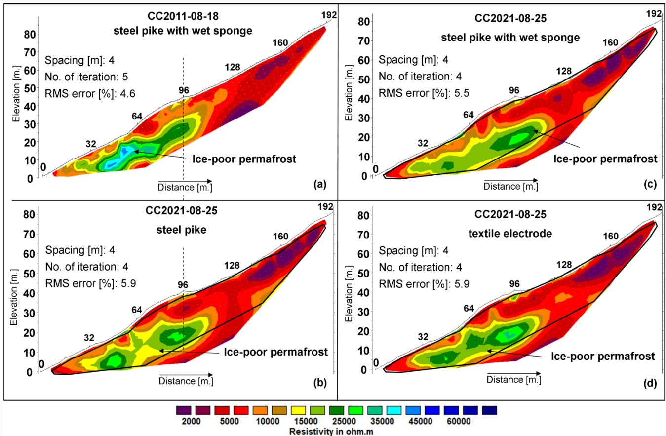
355 Figure 6: Tomograms of the historical (2011) and the repeated (2021) profiles in the Corvatsch catchment: (a) historical profile; (b) repeated profile measured with steel pikes; (c) repeated profile measured with steel pikes and wet sponges; (d) repeated profile measured with textile electrodes. The black lines in (b) to (d) indicate the outline of the historical tomogram. The vertical axes display the relative elevation in meters.,
