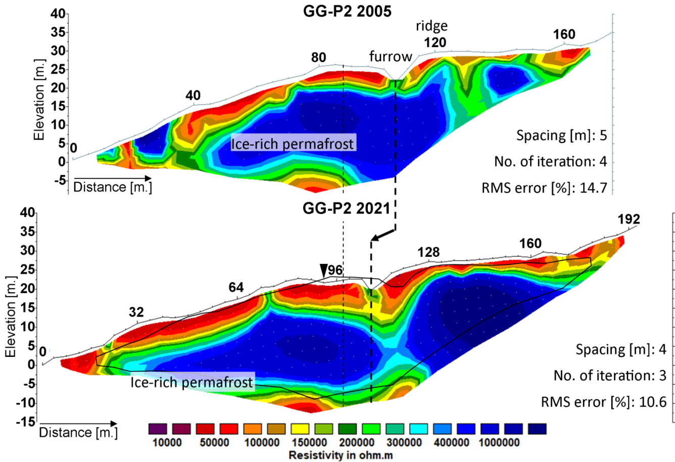
410 Figure 9: Tomograms of the historical (2005) and the repeated (2021) profile GG-P2 on the Gianda Grischa rock Rock glacier/Glacier. The thin black dashed line indicates the common centre point. The point of intersection with tomogram GG-P3 is given by a black triangle. The thick dashed line and the arrow highlight the observed down-gradient shift of furrow. The black line displays the outline of the historical tomogram.
