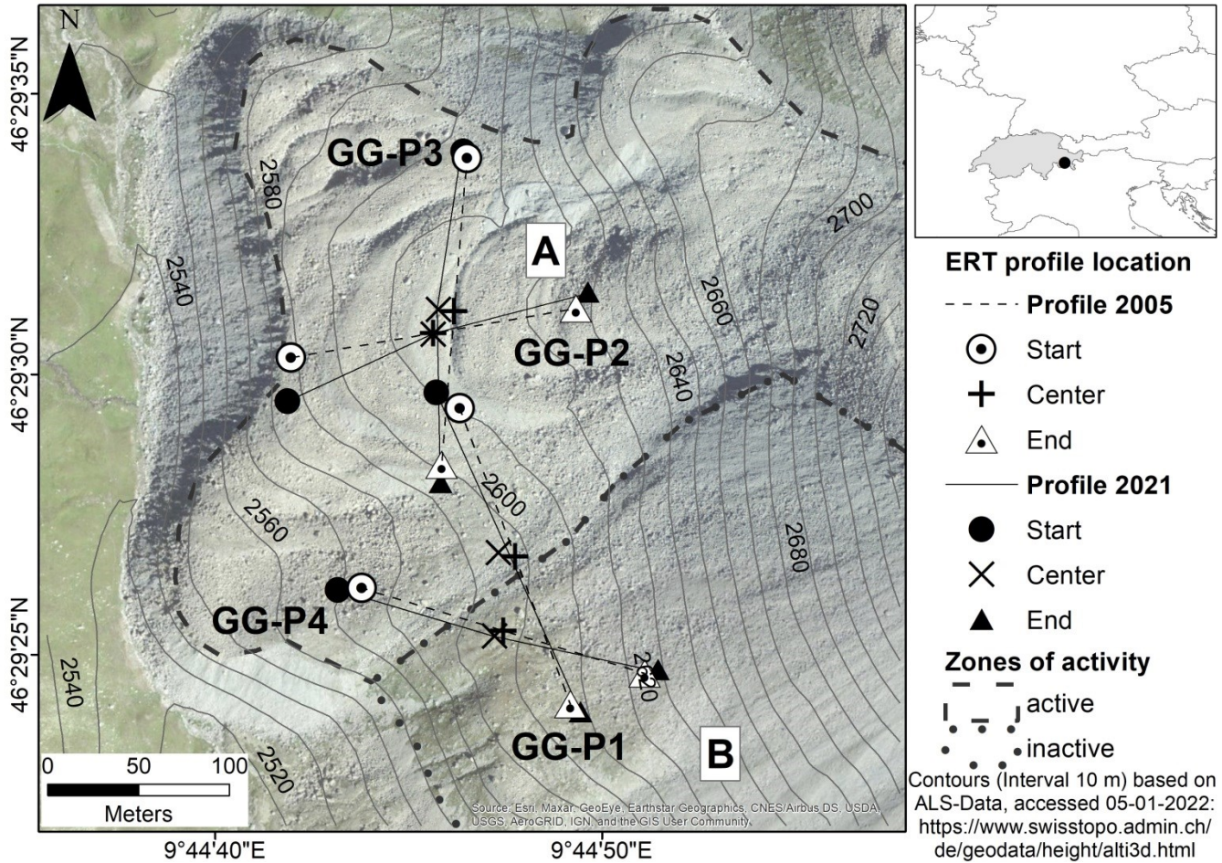
Figure 2: Location of the historical (2005, dashed line) and the repeated (2021, solid line) ERT profiles on the Gianda Grischa Rock glacier, Upper Engadin. The status of activity (A = active; B = inactive) is based on this study and Frauenfelder et al. (2008). The area around A is characterized by furrows and ridges and hosts profiles P2 and P3.
