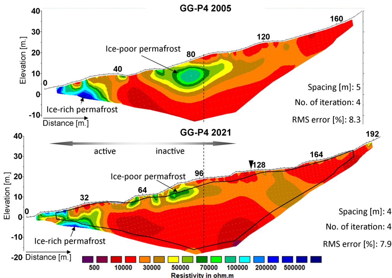
395 Figure 8: Tomograms of the historical (2005) and the repeated (2021) profile GG-P4 on the Gianda Grisca rock-Glacier rock-glacier . The dashed line indicates the common centre point. The point of intersection with tomogram GG-P1 is indicated by a black triangle. The black line displays the outline of the historical tomogram.
