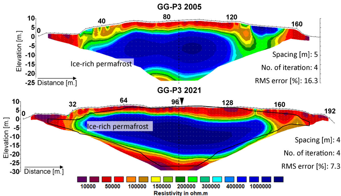
Figure 10: Tomograms of the historical (2005) and the repeated (2021) profile GG-P3 on the Gianda Grisca Rock glacier Glacier. The dashed line indicates the common centre point. The point of intersection with tomogram GG-P2 is indicated by a black triangle. The black line displays the outline of the historical tomogram.
