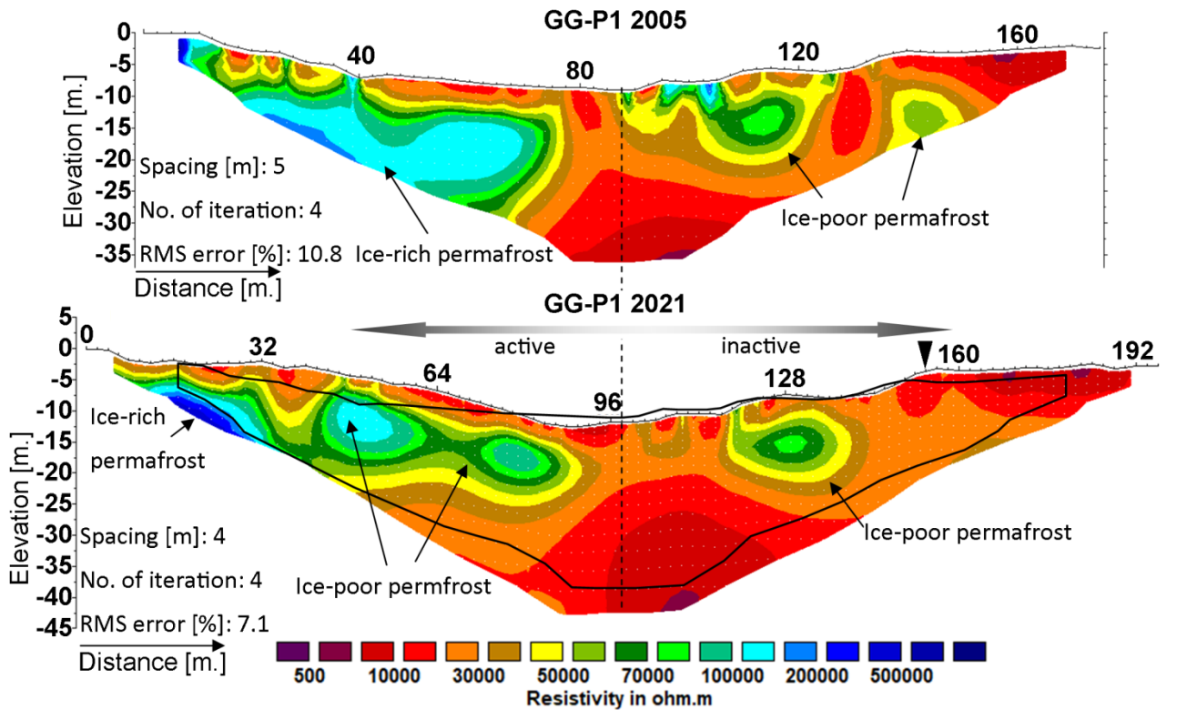
Figure 7: Tomograms of the historical (2005) and the repeated (2021) profile GG-P1 on the Gianda Grisca R ock g lacier. The dashed line indicates the common centre point. The point of intersection with tomogram GG-P4 is indicated by the black triangle. The black line indicates the outline of the historical tomogram.
