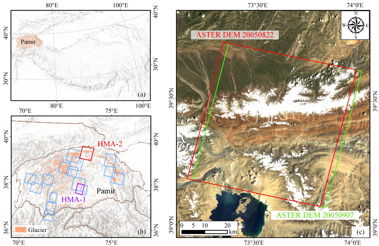
Figure 9. The study area located on HMA. (a) and (b) The footprints (blue) of the 22 DEM pairs, where pairs HMA-1 and HMA-2 listed in Table 4 are highlighted in purple and red, respectively. The glacierized areas are from the RGI 6.0 inventory. (c) The coverage of the two DEM images in HMA-2 (red: ASTER DEM 20050822; green: ASTER DEM 20050907). The background image was acquired by Landsat 5 in 2008.
