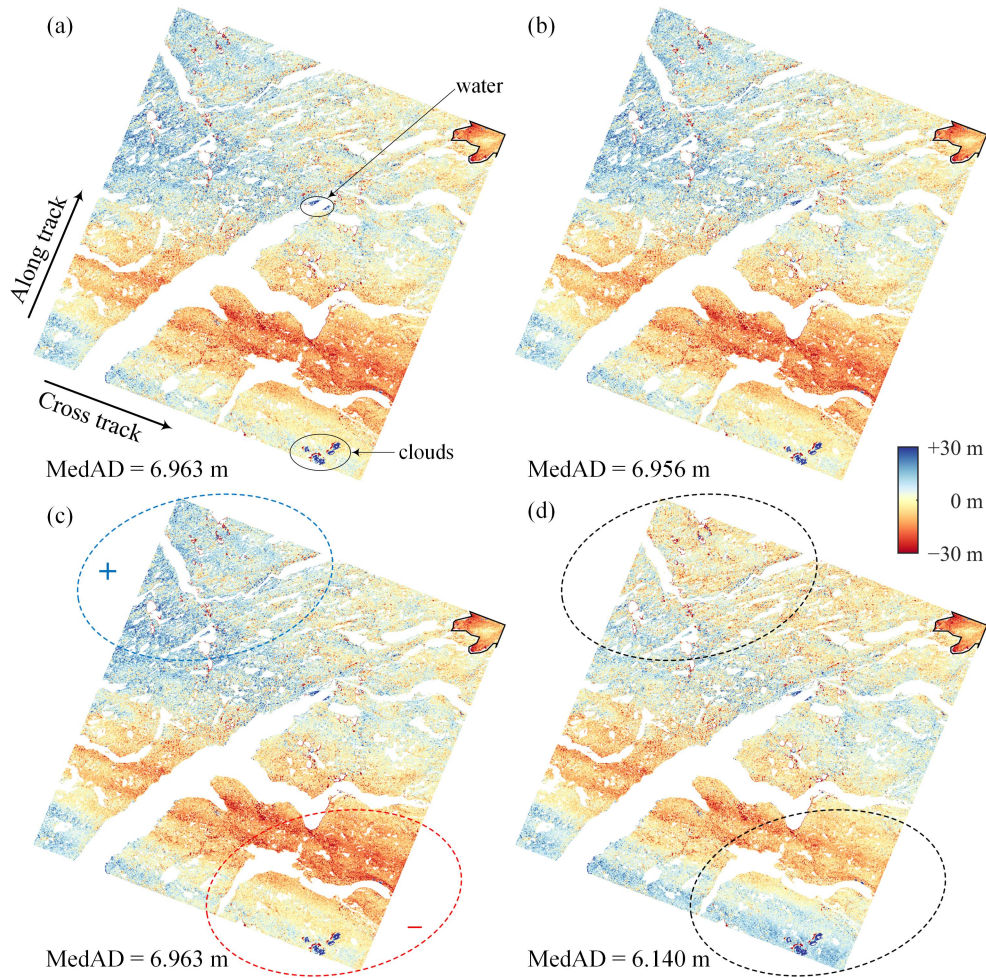
245 Figure 5. Co-registration results of the different methods for DEM pair GrIS-1: the standard (a), simplified (b), and linear (c) versions of the NK method, and the RT method (d).
