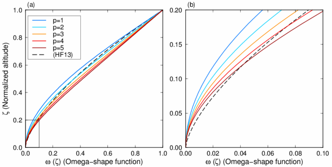
Fig. 2: (a) Normalized vertical velocity profiles adopted from Equation [43] with different p parameters. The dashed black line (HF13) indicates the vertical velocity profile used in Fischer et al. (2013) with m = 0.5 . (b) Enlarged view near the bottom of the ice column (see black rectangle in (a)).
