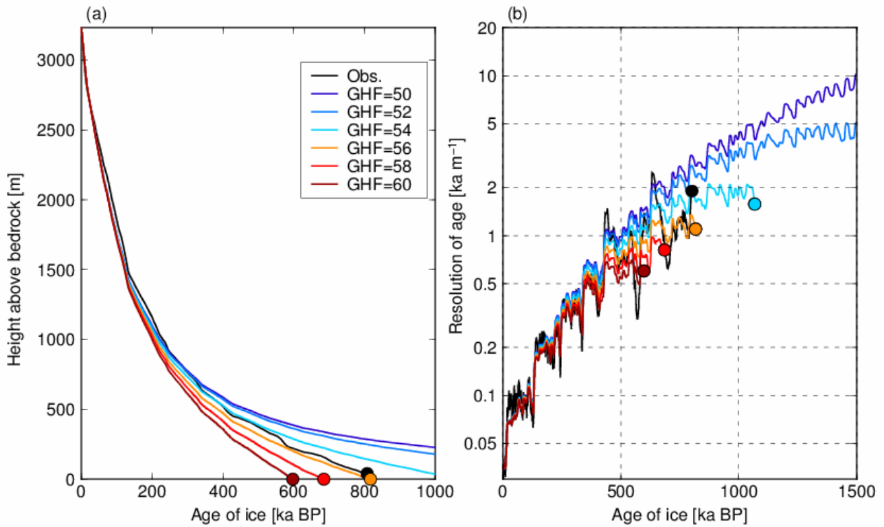
964 Fig. 108: Same as Fig. 6, but results under the EDC configuration (Table 1). The AICC2012 965 chronology (Veres et al., 2013) is used in this figure for the observed depth–age profile. 966
