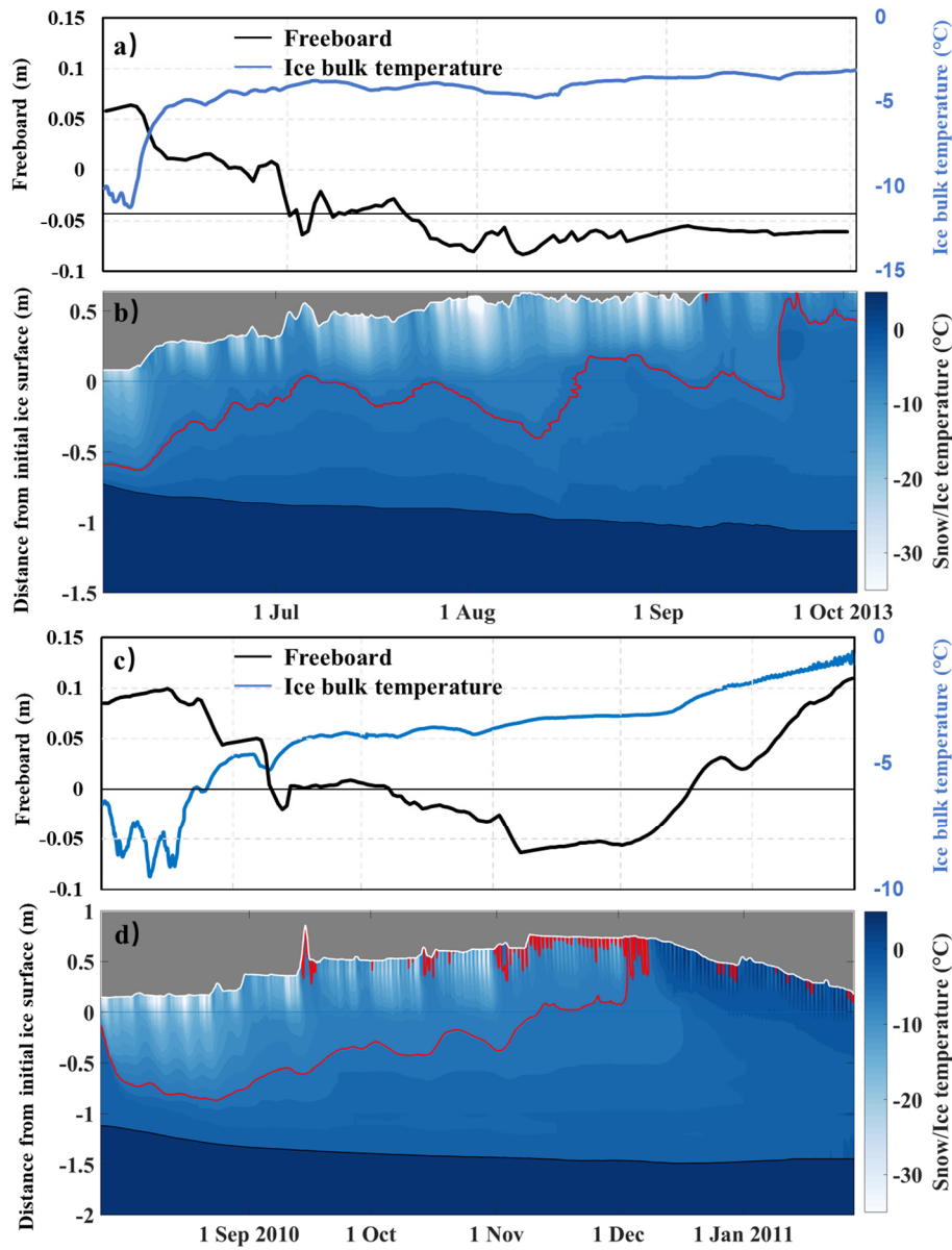
535 Figure 9. Estimated sea ice freeboard and ice bulk temperature, and temperature contours in the snow and sea ice measured by (a and b) ZS2013b and (c and d) ZS2010. The white, red, and black lines in panels (b) and (d) represent the snow surface, the -5^{\circ}\text{C} isotherm, and the ice bottom, respectively. The y-axis zero value denotes the initial snow-ice interface.
