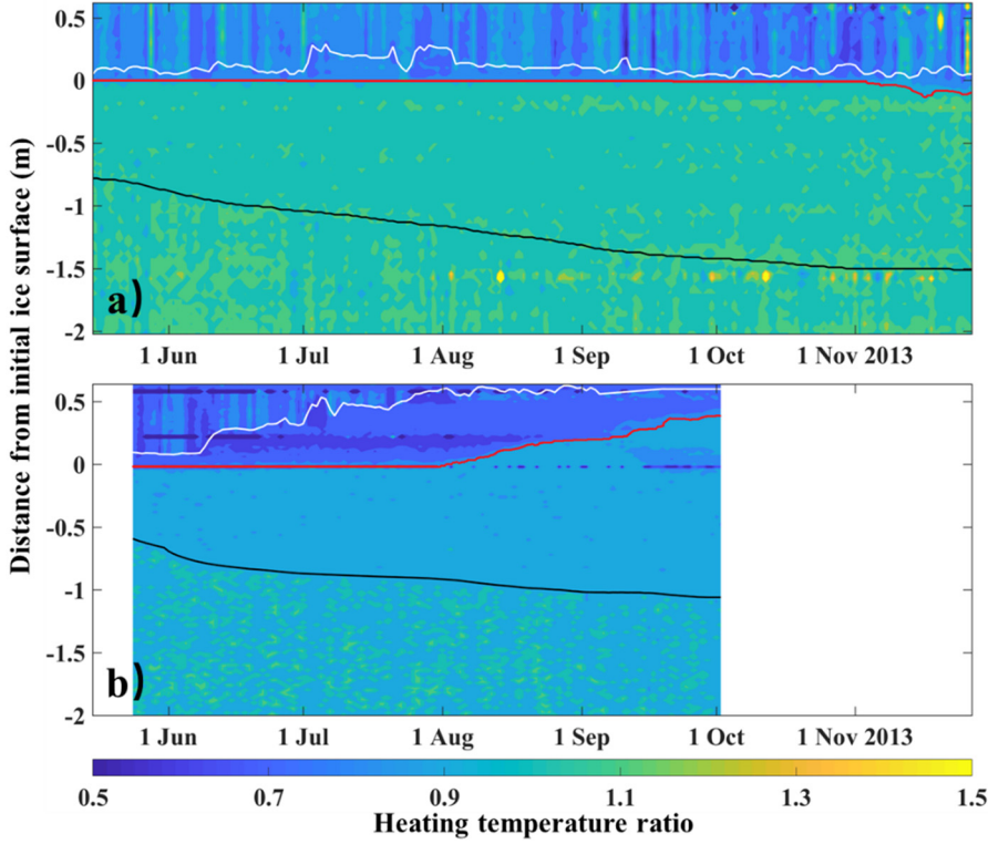
160 Figure 2. Profiles of the pulsed heating (HT) ratio after 30 and 120 s observed by the (a) ZS2013a and (b) ZS2013b SIMBAs, with the white, red, and black lines denoting the snow surface, snow-ice interface, and ice bottom, respectively. The zero y-value refers to the initial snow- ice interface at the buoy deployment.
