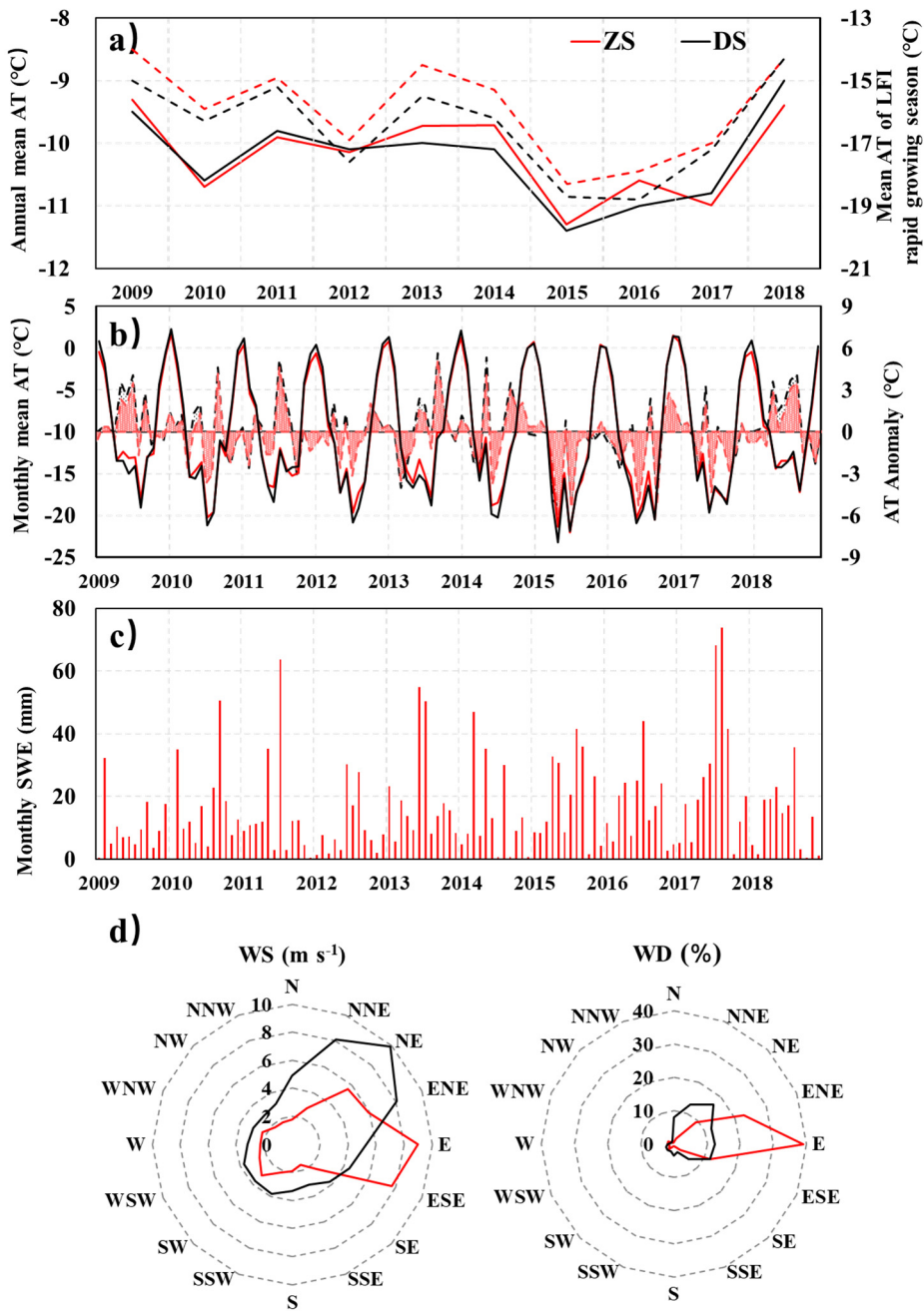
240 Figure 3. Atmospheric parameters measured at ZS (red) and DS (black) from 2009 to 2018: (a) annual mean air temperature (AT; solid line, left axis) and mean AT of the LFI rapid growing season (dashed line, right axis), (b) monthly mean AT (solid line, left axis) and AT anomaly (shaded area, right axis), (c) monthly accumulative SWE of SP obtained from the Russian Progress II Station, and (d) wind speed (WS) and wind direction (WD) frequency distribution.
