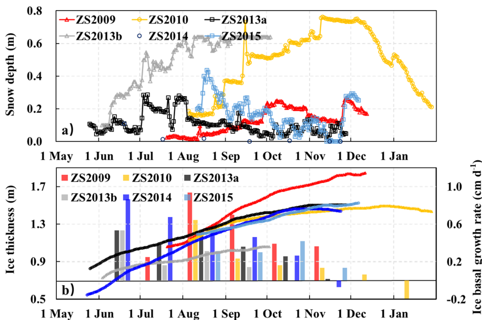
260 Figure 4. Seasonal evolution of (a) the snow depth and (b) the ice thickness (lines, left axis) off ZS derived from CRREL-IMB and SIMBA observations, with the bars in panel (b) denoting the monthly ice basal growth rates (right axis). The snow depth of ZS2014 was obtained from in-situ measurements and showed as blue circles.
