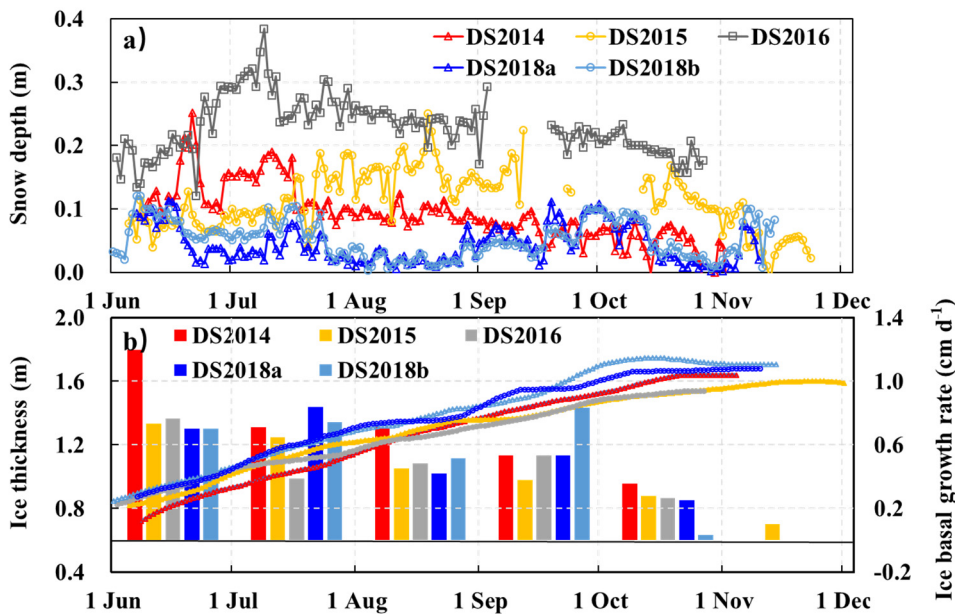
310 Figure 5. Same as Figure 4, but for DS.
