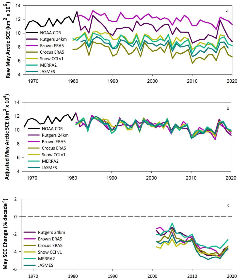
Figure 1. Raw time series of May Arctic snow extent (a), adjusted time series (b), and rate of change since 1981 of adjusted time series (c).
