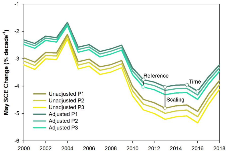
270 Figure 4. Change in Arctic SCE ( \% \text{ decade}^{-1} ) for May since 1981 relative to three reference periods (P1, P2, P3, see Table 2) and scaled versus unscaled datasets since 1981 through the year noted on the x-axis. The impact of year-to-year increases in time series length, reference period differences, and changes due to dataset adjustments are noted.
