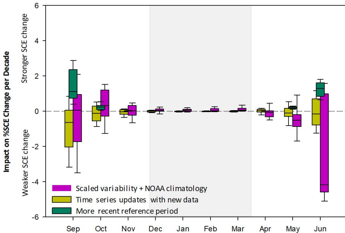
290 Figure 5. Sensitivity of Arctic snow cover extent rate of change calculations (expressed as % decade -1 ) to changes in the available time series length, selection of reference period, and the adjustment process. Values above zero indicate a stronger SCE rate of change; values below zero indicate a weaker SCE rate of change.
