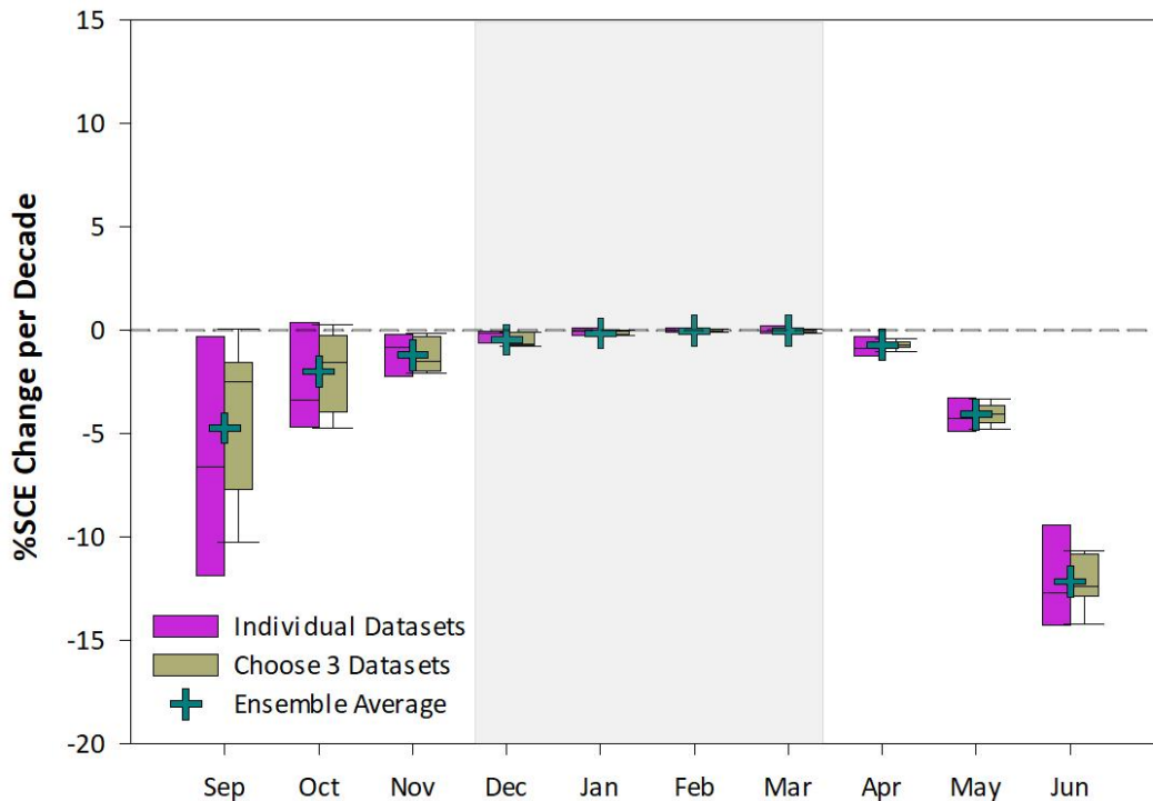
305 Figure 6. The impact of dataset averaging (new product set) on rates of change in Arctic SCE.
