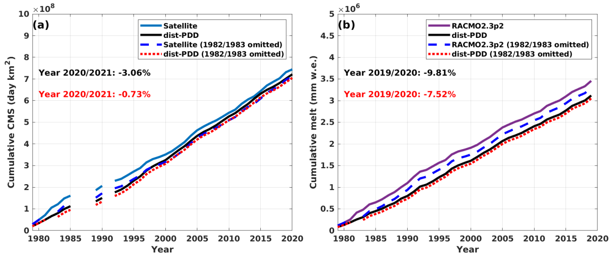
Figure E2. (a) cumulative CMS for satellite estimates and dist-PDD/ dist-PDD (1982/1983 omitted) outputs from 1979/1980 to 2020/2021 (with 1986/1987 to 1988/1989 and 1991/1992 omitted. (b) cumulative annual melt amount for RACMO2.3p2 simulations and dist-PDD/ dist-PDD (1982/1983 omitted) outputs from 1979/1980 to 2019/2020.
