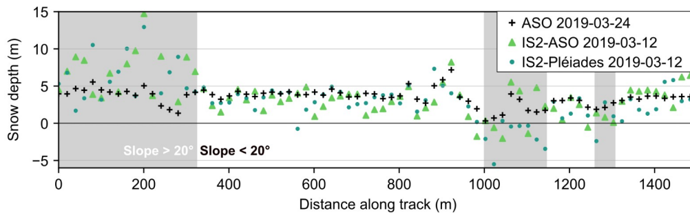
Figure 4. Transect of the snow depths on 12 March 2019 derived from ICESat-2 – ASO DTM (green triangles), ICESat-2 – Pléiades DSM (green circles) and on 24 March 2019 by ASO (black cross). Slopes steeper than 20^\circ are shaded as an indication of areas prone to larger errors. This transect is the northernmost of the first beam available on that date (Figure 3a).
