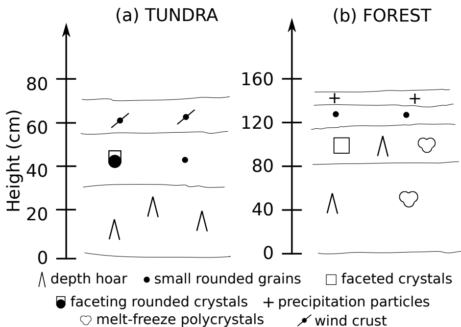
Figure 5. Simplified stratigraphies from February 2014 representing typical snow conditions at sites (a) TUNDRA (25 February) and (b) FOREST (24-28 February). Note that the y-scales are different for the two sites.
