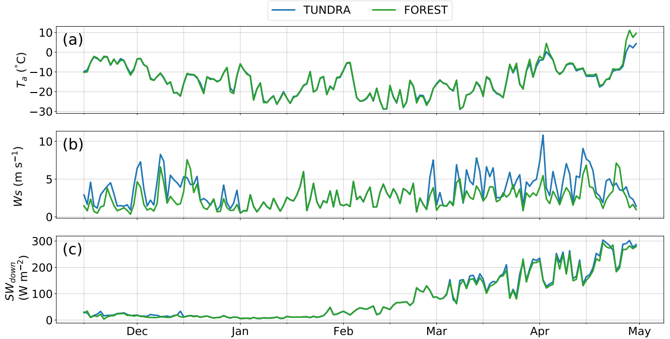
Figure 2. Daily mean (a) air temperature T_a , (b) wind speed W_s and (c) downwelling shortwave radiation SW_{down} measured at the two sites TUNDRA and FOREST for winter 2018-19. Labeled tick marks on the x-axis indicate the start of each month.
