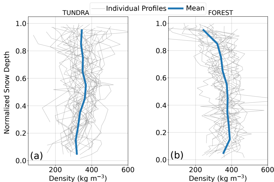
Figure 6. Snow density profiles from 29 snow pits in tundra environments near TUNDRA in tundra environments near TUNDRA and 18 snow pits in forested environments near FOREST in forested environments near FOREST collected between January and March from the years 2012 to 2019. For better comparability, snow heights were normalized. The means of all profiles are also shown.
