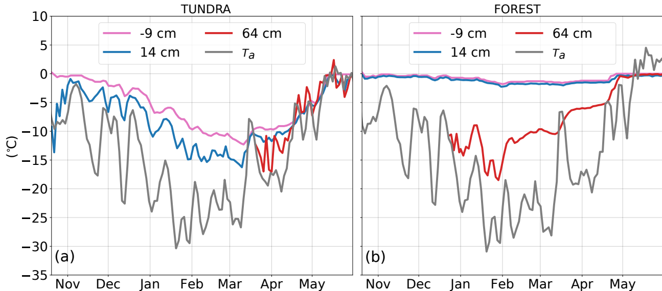
Figure 8. Snow (blue and red lines ), ground (pink curve ) and air temperatures (grey curve ) at the (a) TUNDRA and (b) FOREST for winter 2018-19. Heights at which measurements were taken are relative to the surface of the ground surface . Air temperature T_a was measured at 2.3 m above ground. The values correspond to measurements collected once every two days other day at 5 AM.
