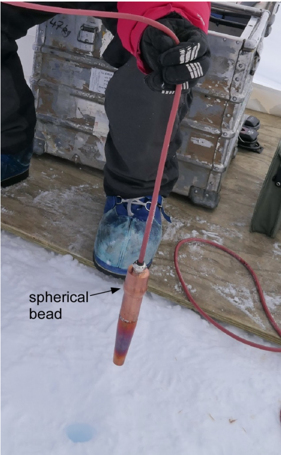
Figure 2: Heated copper "plumb bob" for melting and glazing first 6 m of firm hole.
