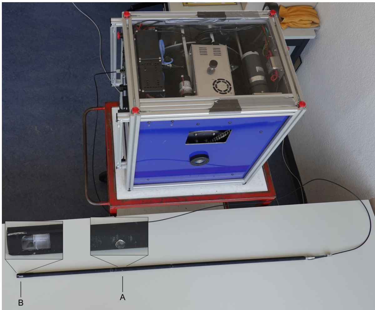
Figure 11: Logger and 3.5 mm fiberoptic cable winch. A: emitting 405-nm LED. B: Receiving window and mirror.
