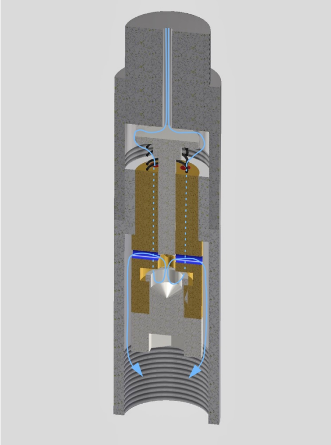
135 Figure 6: Cross section through mechanical flow controller. The direction of flow is from top to bottom. The fluid flows through the red holes below the deflection disk into the space below the pin and exits through the blue holes.
