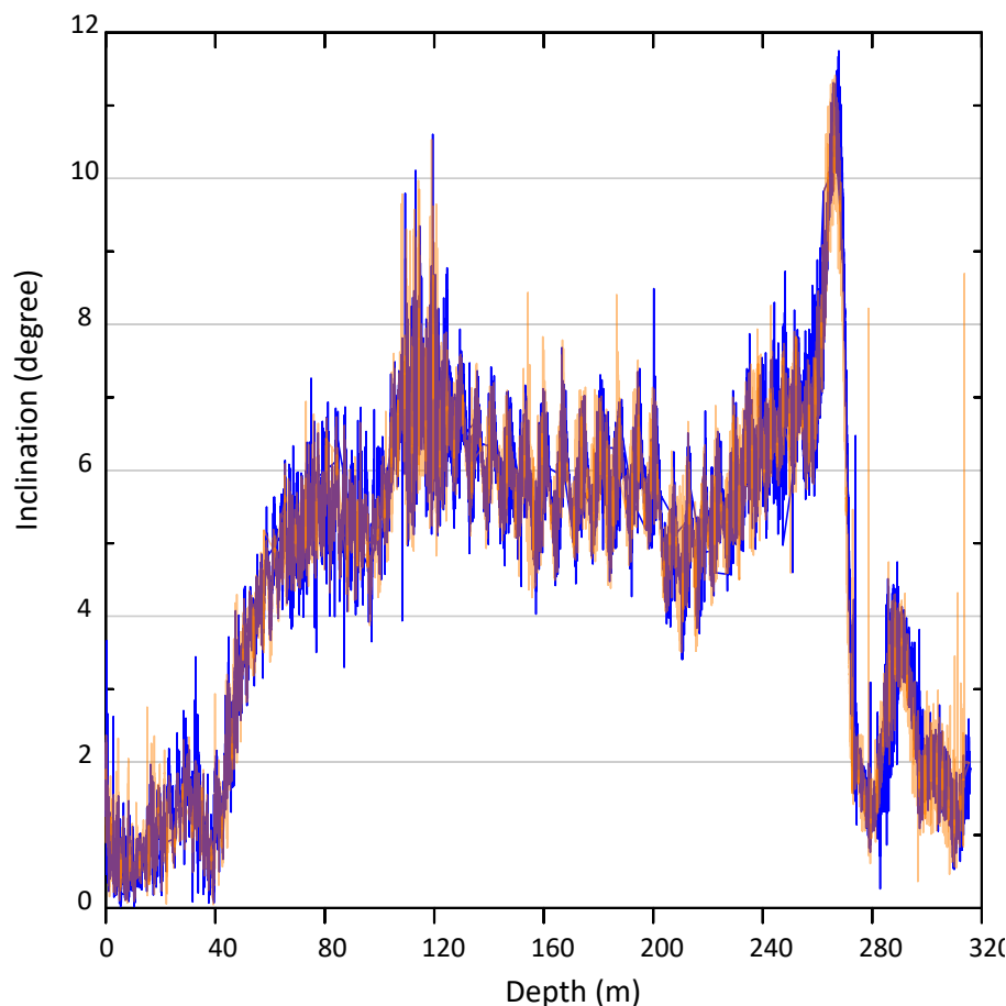
Figure 15: LDC 21/22 hole inclination (324 m hole). Blue: downward logging; orange: upward logging. The noise of the order of 1 degree on the submeter scale is caused by the acceleration (shaking) when lowering and raising the logger.
