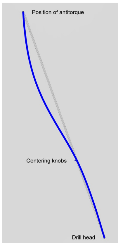
Figure 12: Bending of drill by gravity (exaggerated). Finite element simulation with actual material properties and tests with the drill itself led to an optimal position of the centering knobs at about one third from the lower end.
