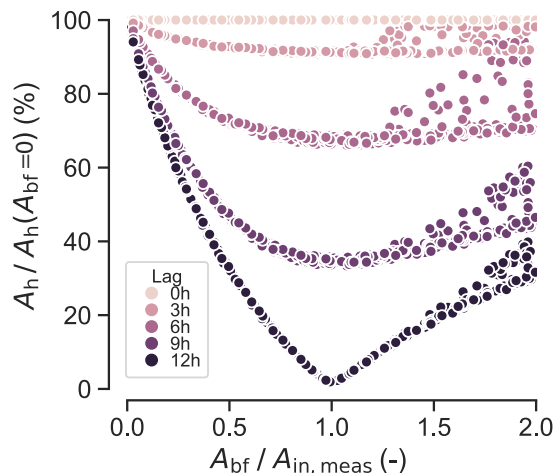
Figure 9. Sim E1d: Hydraulic head oscillation amplitude A_h , as a percent of the amplitude without baseflow ( A_h(A_{bf}=0) ), versus the ratio between baseflow amplitude ( A_{bf} ) relative to the measured surface meltwater input amplitude ( A_{in,meas} ), for different surface input–baseflow phase lags. Baseflows with larger amplitudes of oscillations (x-axis), or that are more out of phase with the surface melt (darker colors), generally produce smaller-amplitude head oscillations.
