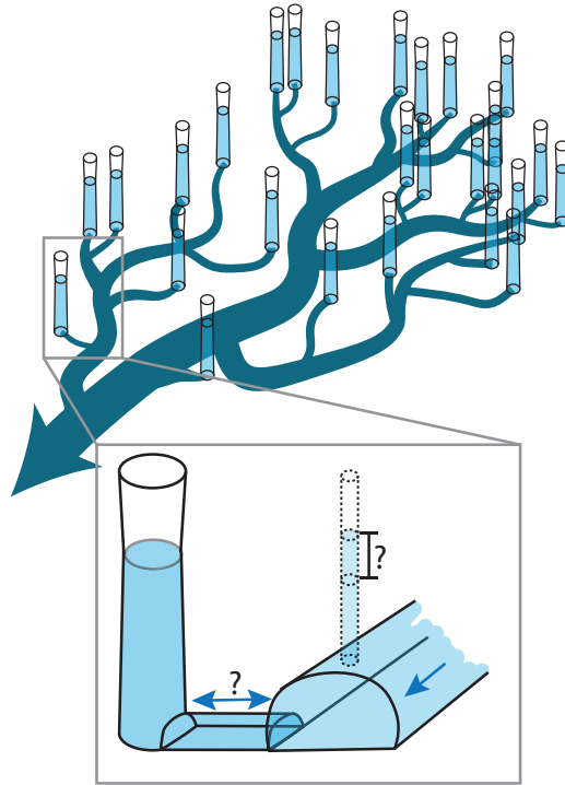
Figure 10. Subglacial network connectivity illustrated by a dendritic subglacial channel system (dark blue), initiated by moulin forming tributaries that connect to higher-order channels.
