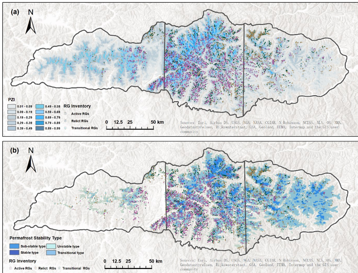
Figure 8: Spatial distribution of rock glaciers vs. (a) Gruber's (2012) Permafrost Zonation Index (PZI) in Guokalariju and (b) Map of the thermal stability of permafrost in Guokalariju (Ran et al. , 2020).
