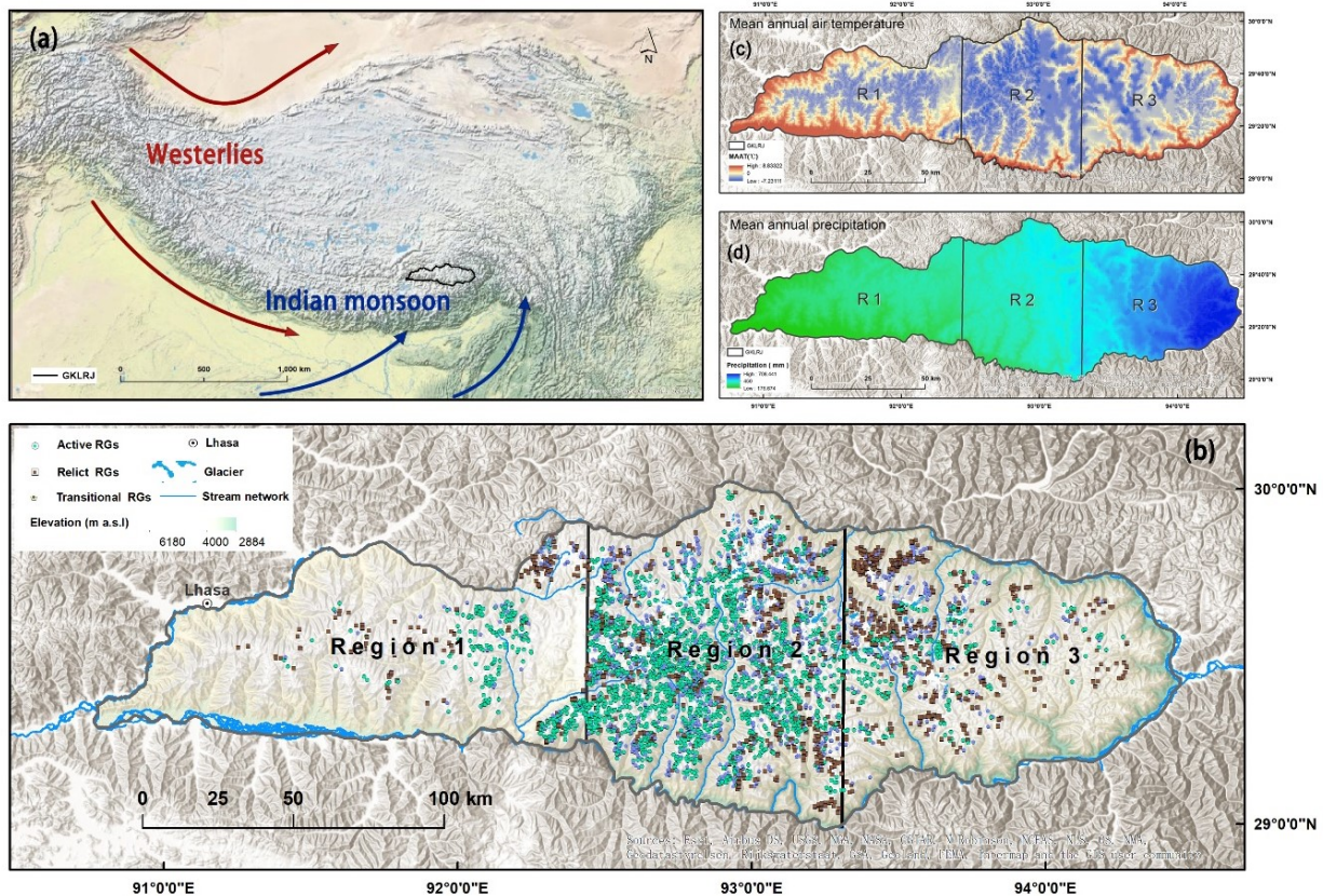
Figure 1: (a) The location of Guokalariju on the TP; (b) The three sub-regions and the spatial distribution of streams. Rock glaciers are categorized as green (active rock glaciers), purple (transitional rock glaciers), and brown (relict rock glaciers), and glaciers are shown in light blue and white; (c) Mean annual air temperature map for the Guokalariju (Du and Yi, 2019); (d) Mean annual precipitation map for the Guokalariju (Du and Yi, 2019). Maps were created using ArcGIS® software by Esri.
