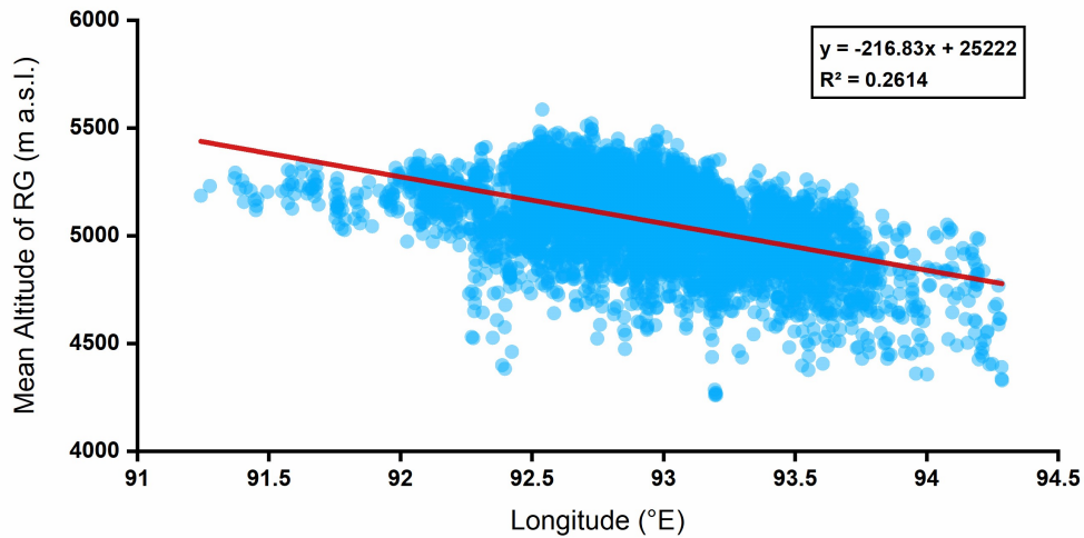
230 Figure 5: Scatterplots and fitted curves of the mean altitudinal distribution of rock glaciers versus longitude.
