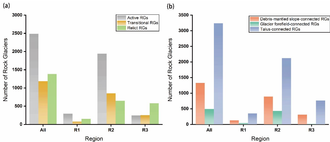
200 Figure 3: The number of rock glaciers categorized by different(a) activity types and (b) upper slope connection types in the entire study region and its sub-regions.
