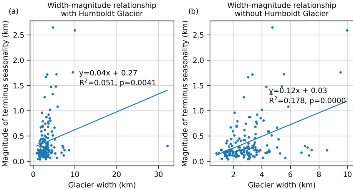
Figure S6. Relationship between glacier width and the magnitude of terminus-position seasonality, (a) with and (b) without Humboldt Glacier, a major width outlier.
