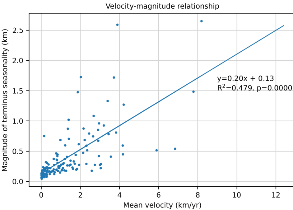
Figure S7. Relationship between glacier velocity and the magnitude of terminus-position seasonality.
