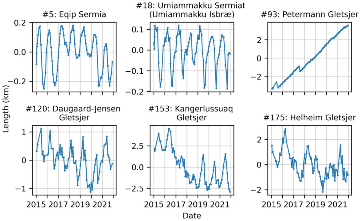
Figure S3. Length time series for selected glaciers digitized at monthly resolution. One glacier from each ice-sheet region is represented. All lengths are given in kilometers on the y-axis.
