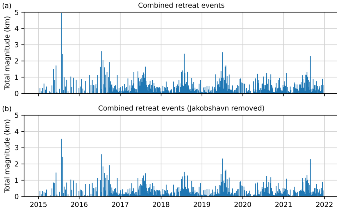
Figure S5. Timing and magnitude of retreat events combined across the 20 six-day glaciers, both (a) with and (b) without Sermeq Kujalleq (Jakobshavn Isbræ, no. 3). If multiple retreat events occur at different glaciers on a single day, their retreat magnitudes are added together. In (b), Jakobshavn is removed to show that it is not solely driving the seasonality in retreat events.
