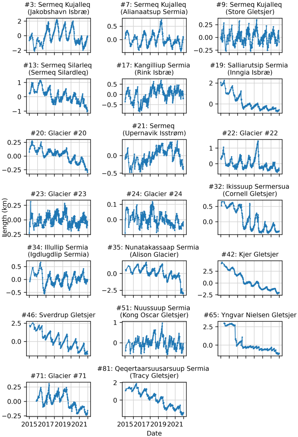
Figure S2. Length time series for the 20 glaciers digitized at six-day resolution. All lengths are given in kilometers on the y-axis.
