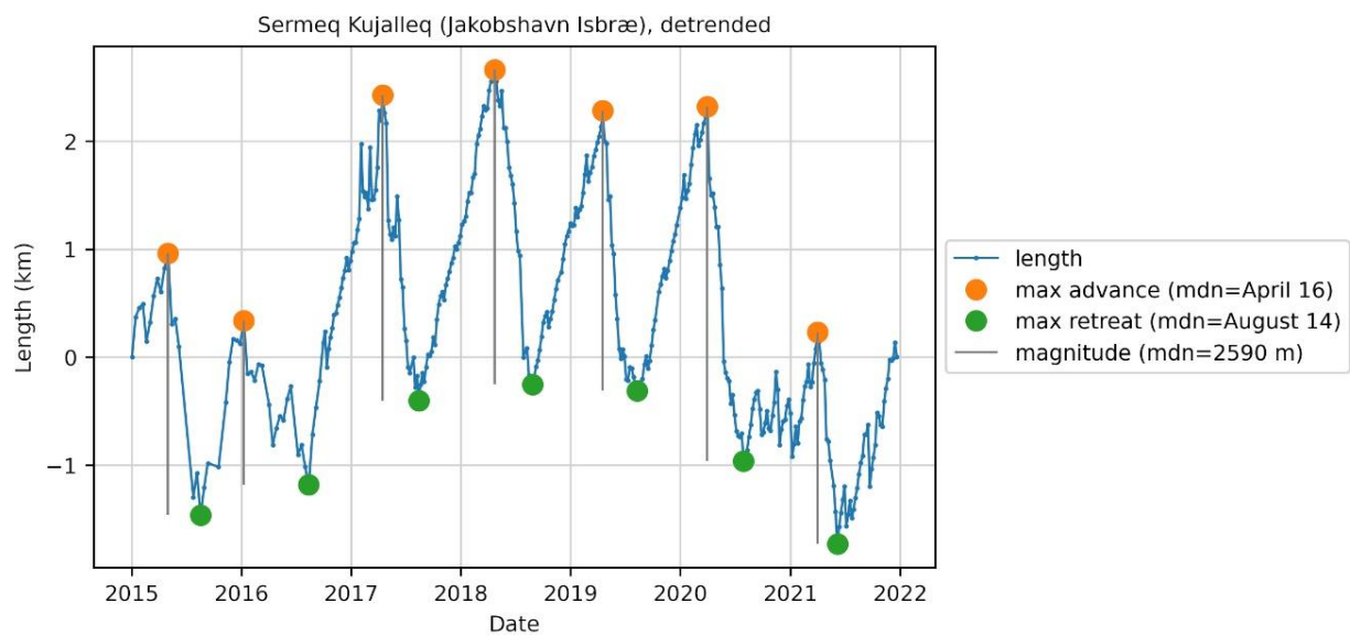
Figure S1. Illustration of the process of determining the annual dates of greatest advance (orange dots) and greatest retreat (green dots) and the annual magnitude of retreat (gray vertical line), demonstrated for Sermeq Kujalleq (Jakobshavn Isbræ, no. 3). The dates of greatest advance and retreat are identified in the original time series, then the time series is detrended and the dates are plotted on the detrended time series. The detrended length at the date of greatest retreat is subtracted from the detrended length at the date of greatest advance to calculate an annual magnitude of retreat. The median dates of greatest advance and retreat and the median magnitude of retreat are reported in the legend.
