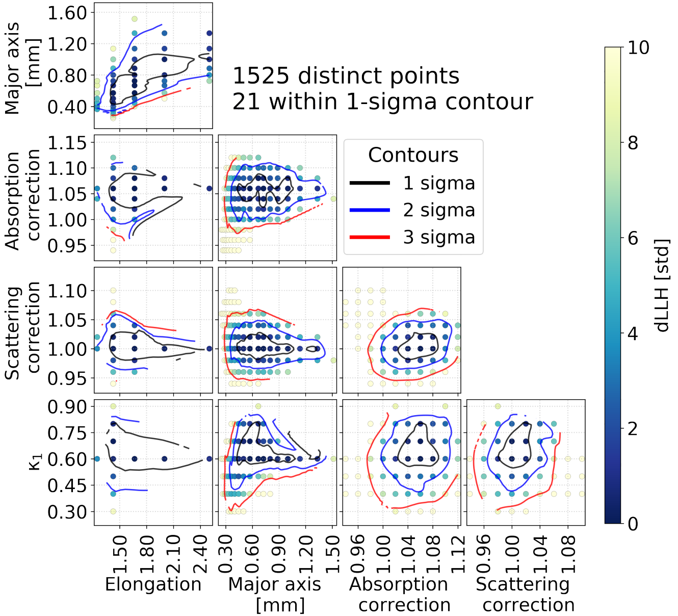
Figure 12. Log-likelihood (LLH) space, where each point quantifies the agreement of a simulation data with a set of assumed parameter values against data, for one ice layer and a subset of parameters. Each panel shows a marginalized 2D space, each point being a simulated ice realization, color coded by its LLH distance from the best fit. In this example, the absorption anisotropy ( \kappa_1 ) is a free parameter (corresponding to the final model).
