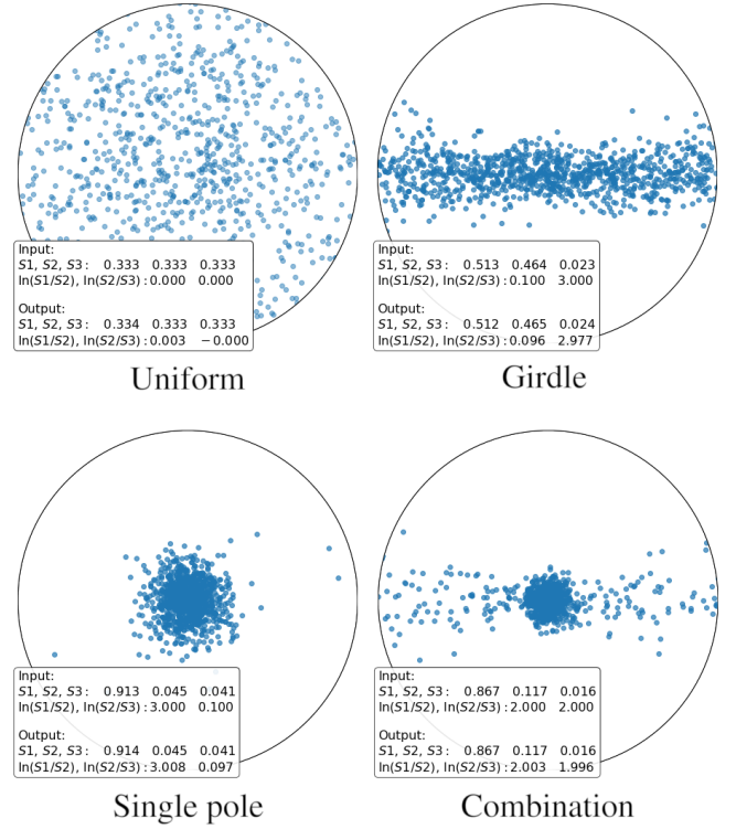
Figure A2. Example c-axis distributions in Schmidt equal-area projection generated using the described method.
