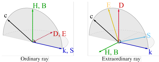
Figure 7. Orientation of all electromagnetic vectors for the ordinary and extraordinary ray with respect to the crystal axis ( c -axis). See text for detailed explanation of this figure.
