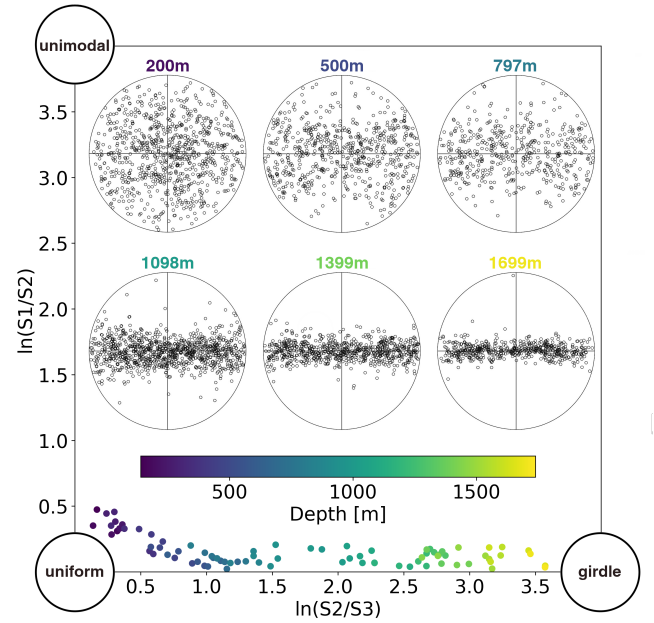
Figure A1. Fabric versus depth trajectory as measured in the SPC14 ice core. Individual c-axis distributions at example depths are shown superimposed in the Schmidt equal-area projection. The ice features a prominent girdle fabric at the overlapping depths instrumented by IceCube starting at \sim 1450 m. Adapted from Voigt (2017).
