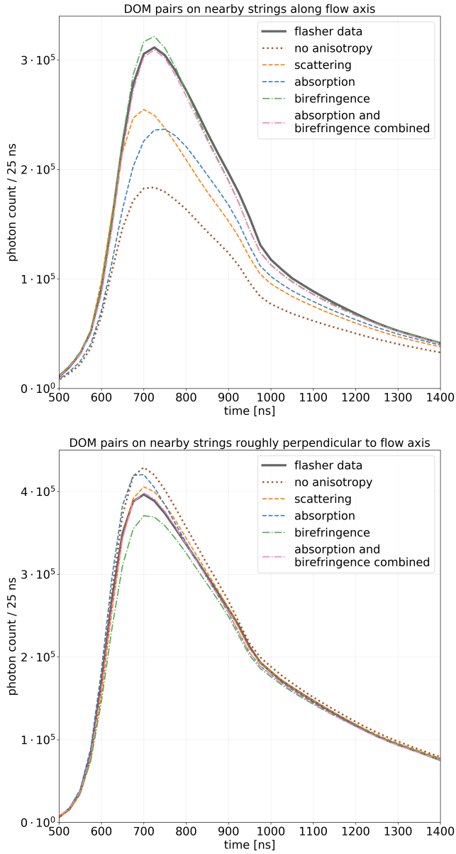
Figure 6. Comparison of fit quality achieved with different models for the ice optical anisotropy. Shown are photon arrival time distributions (summed counts in 25 ns time bins) for all nearest-pair emitters and receivers, roughly aligned along and perpendicular the ice flow. As more emitter-receiver pairs are included in the perpendicular case compared to the case along the ice flow, the total photon counts are not directly comparable between the two plots, and should instead be compared to the curve titled "flasher data" within each plot. While the array geometry is well aligned with the flow axis, the nearest inter-module propagation direction perpendicular to the flow is roughly 30^\circ off. The "absorption" and "scattering" models represent an ad-hoc, directional modifications to Mie scattering and absorption, but are unable to describe timing and intensity simultaneously. "Birefringence" refers to the microstructure based effect introduced in this paper. A combination of the "absorption" and "birefringence" model yields the closest match to data to date.
