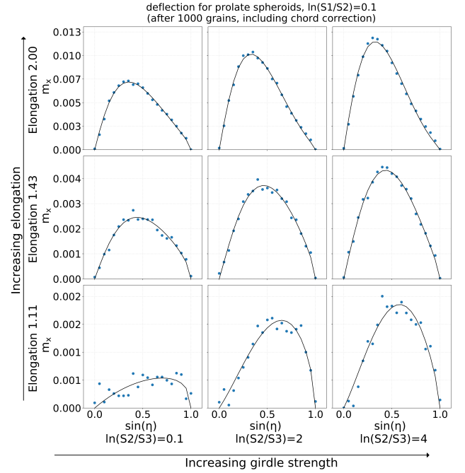
Figure 11. Deflection m_x as described in the text as a function of opening angle to the flow for a number of crystal configurations. The black curves were fitted through the blue, simulated points using the functional form introduced in Equation 17. Note the different ordinate scales per row.
