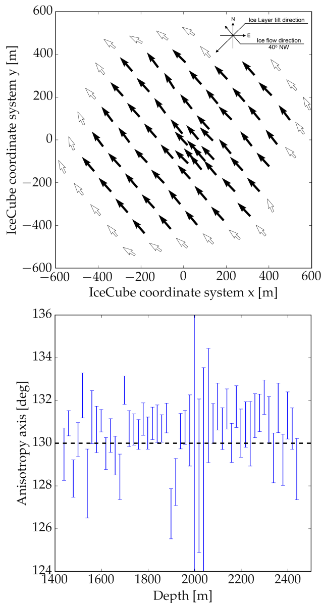
Figure 5. Measured anisotropy axes as a function of lateral position averaging over all depth (top) and as a function of depth averaging over all strings (bottom). Strings on the perimeter of the detector have been excluded, as the lack of symmetric neighbors leads to potentially biased results. The sensitivity is greatly reduced in the region of strongest scattering around 2000 m. The dashed line indicates the anisotropy angle averaged over all strings.
