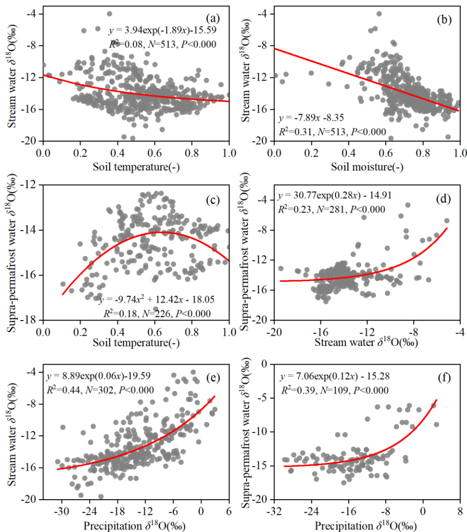
265 Figure 5. Correlation analysis between stable isotopes and influencing factors. (a) and (b) correlations between stream water \delta^{18}\text{O} with: soil temperature and moisture, respectively; (c) and (d) correlations between supra-permafrost water \delta^{18}\text{O} with: soil temperature and stream water \delta^{18}\text{O} , respectively; (e) and (f) correlations between precipitation \delta^{18}\text{O} with: stream and supra-permafrost water \delta^{18}\text{O} , respectively; Red line is the fitted line; Soil moisture and temperature data used in correlation analysis were normalized. “-” presents dimensionless. The soil moisture and temperature data were the daily average value of all the sensor data in the soil layer.
