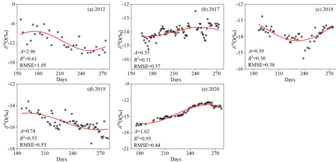
320 Figure 9. Fitted sine-wave regression models to \delta^{18}\text{O} in supra-permafrost water in Xiaoliuyu catchment during 2012, 2017–2020. A is the amplitude and RMSE is root mean square error for the modelled isotopic signature.
