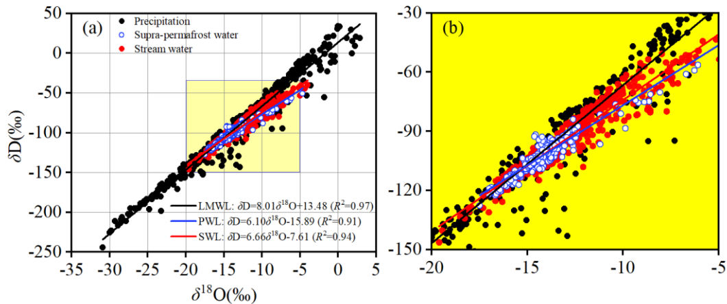
220 Figure 3. Relationships between \delta^{18}\text{O} and \delta\text{D} of precipitation, stream water, and supra-permafrost water. (a) all isotope data; (b) the data, constrained by yellow square.
