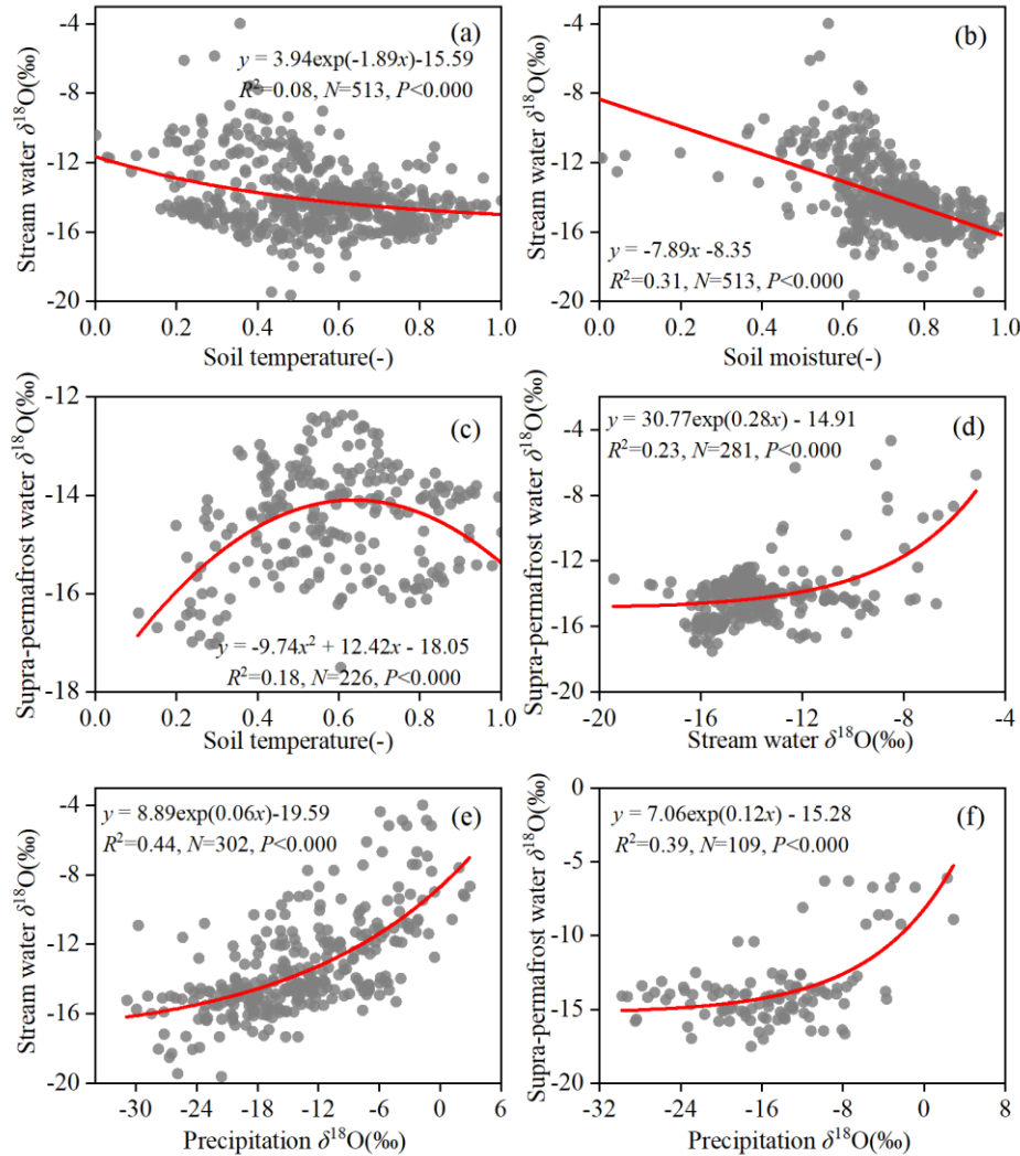
255 Figure 5. Correlation analysis between stable isotopes and influencing factors. (a) and (b) correlations between stream water \delta^{18}\text{O} with: soil temperature and moisture, respectively; (c) and (d) correlations between supra-permafrost water \delta^{18}\text{O} with: soil temperature and stream water \delta^{18}\text{O} , respectively; (e) and (f) correlations between precipitation \delta^{18}\text{O} with: stream and supra-permafrost water \delta^{18}\text{O} , respectively; Red line is the fitted line; Soil moisture and temperature data used in correlation analysis were normalized. “-” presents dimensionless.
