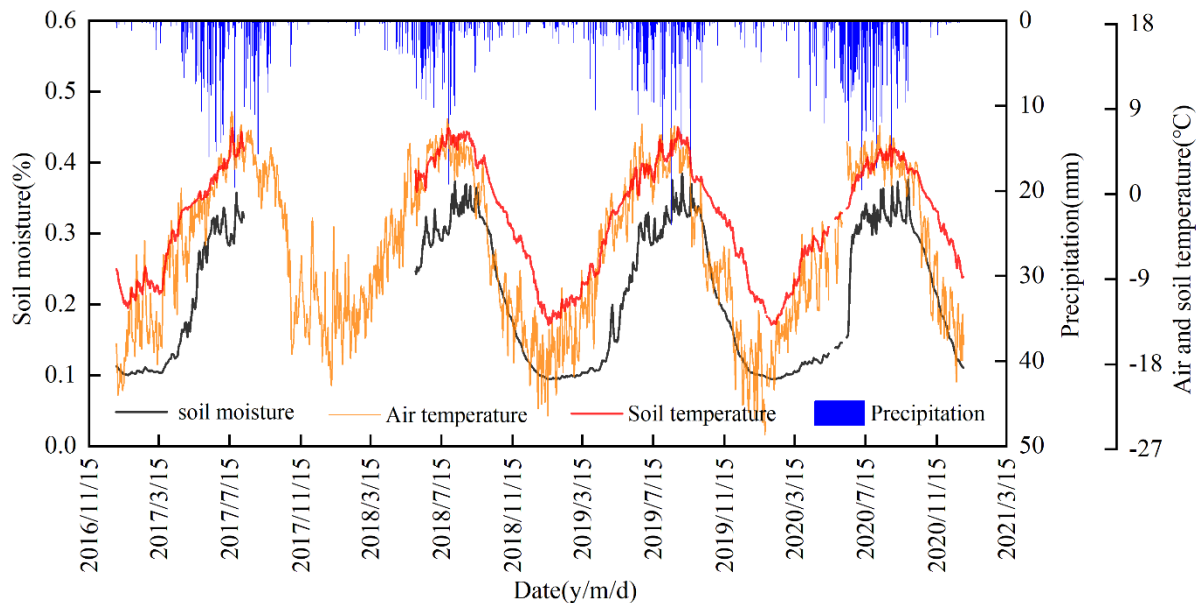
100 Figure 2. Temporal variation of soil moisture, soil temperature, air temperature, and precipitation from 2017 to 2020.
