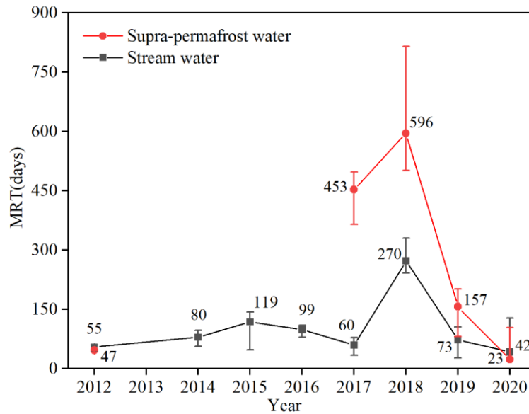
340 Figure 11. Inter-annual variation of stream water MRT during 2012, 2014–2020, and supra-permafrost water MRT during 2012, 2017–2020.
