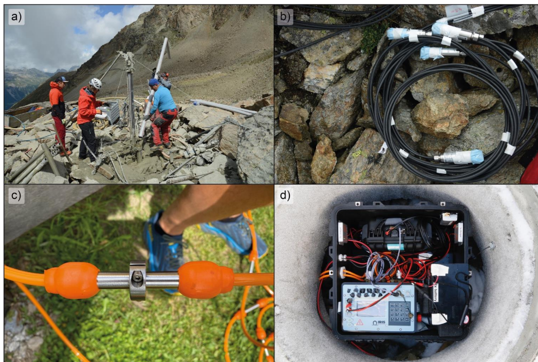
Figure 2: a) Drill and protective PVC pipe used to drill boreholes B3, B4 and B5 on Schafberg rock glacier in August 2020; b) Piezometers and temperature sensors ready to be installed in B5; c) Stainless steel ring mounted on cross-borehole ERT electrode to improve ground contact; d) Cross-borehole ERT logging system for B3 and B4 in a concrete chamber (ERT instruments in Fig. 1c).
