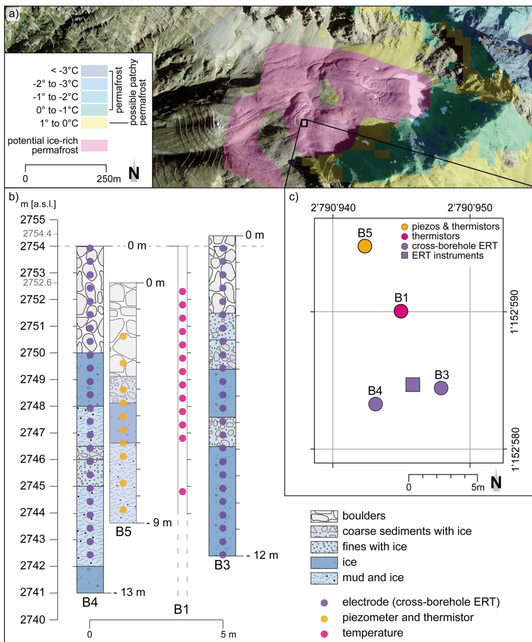
Figure 1: a) Permafrost distribution at the Schafberg study site (Permafrost and ground ice distribution map of Switzerland, Kenner et al. 2019). Aerial photograph: swisstopo; b) Borehole stratigraphy in B3, B4 and B5 (drilled in 2020) and positions of the ERT electrodes (purple dots) and borehole piezometers/temperature sensors (yellow dots (B5) and pink dots (B1)). No stratigraphy is shown for B1 (drilled in 1990); b) Positions of the boreholes and instruments relative to each other and their position on the Schafberg rock glacier (1a, black rectangle).
