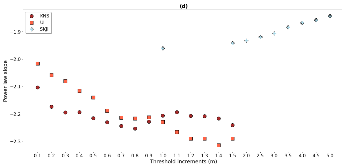
Figure 5. Iceberg frequency for each threshold increment tested. a) SKJI's increments were every 0.5 m above sea level between 0 and 5 m above sea level. Increments of 0.1 m between 0 and 1.5 m above sea level were ran for both b) UI, c) KNS. d) shows how the \alpha value for each glacier changes, depending on which threshold increment is chosen to detect their respective icebergs. Note the log-scale on the y-axis in subplot: a, b and c, and normalised y-axis and the x-axis for SKJI (a) is on a different scale to that of UI (b) and KNS (c).
