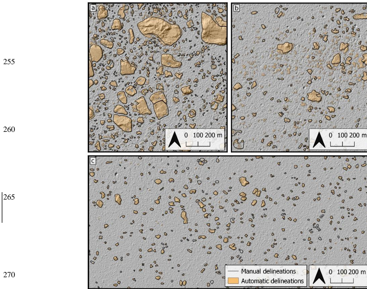
Figure 4. Manual (black lines) and automated (orange) delineation of the iceberg subset for a) SKJI (2011-09-10), b) UI (2012-07-04) and c) KNS (2013-08-21) overlaving the hillshaded ArcticDEM v3 strip data for each glacier.
