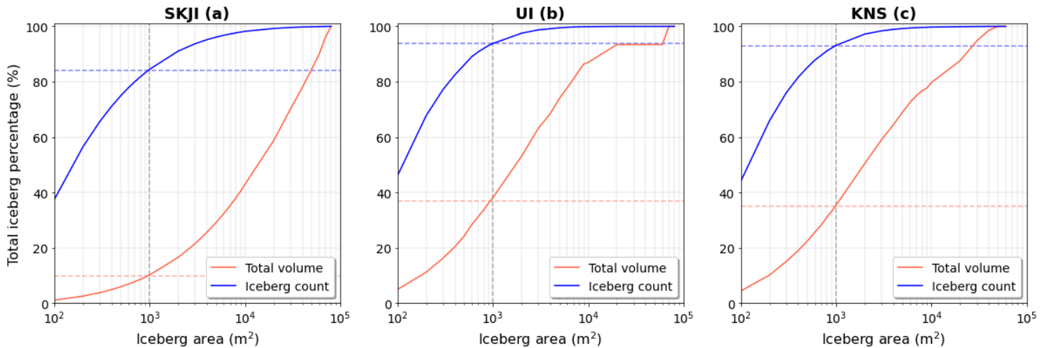
495 Figure 9. Cumulative iceberg volume (orange line) and count (blue line) plotted as percentage with their respective surface area. The small iceberg threshold ( \leq 1,000 \text{ m}^2 ) is defined by a dashed grey line. The total volume made up by small icebergs is represented by the orange dashed line and the total number is the dashed blue line. 84% of all the icebergs at SKJI are small, however they only account for 10% of the total volume, whereas they account for 94% of the total count at UI and 37% total volume. 93% of the icebergs are small at KNS and account for 35% of the total volume.
