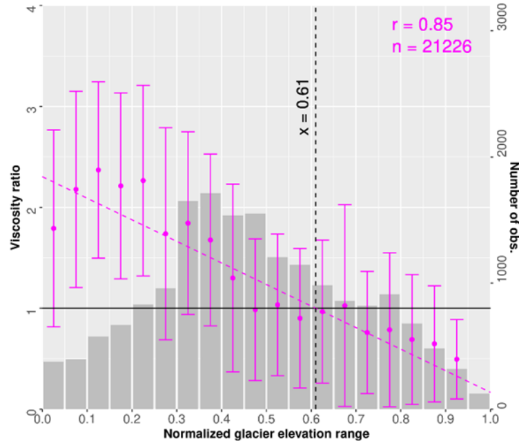
390 Figure 55: Elevation-dependent viscosity ratio of H_{SIA1970}^{in-situ} and H_{SIA1970}^{retreat\ 02} reconstruction at locations of in-situ observations. Elevations have been normalized for each glacier with 0.0 being the minimum and 1.0 the maximum glacier height. Magenta points denote mean viscosity ratio values aggregated within 0.05 normalized elevation bins on glacierized areas. The number of observations of each bin is shown as gray bars. The respective linear regression of the elevation-derived viscosity ratio is shown as dotted line. Ratios of elevation bins with less than 100 observations are excluded from the analysis. Vertical error bars indicate the respective mean ratio \pm one standard deviation. The elevation threshold ( h_{\eta}^{thres} ) is indicated as vertical black dotted line at 0.61 normalized glacier elevation. 395
