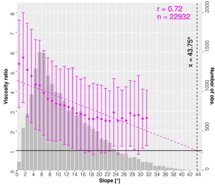
365 Figure 4: Slope-dependent viscosity ratio of H_{SIA1970}^{in-situ} and H_{SIA1970}^{retreat\ 01} at locations of in-situ observations. Magenta points denote mean viscosity ratio values aggregated within 2^\circ slope bins on glacierized areas. The number of observations of each slope bin is shown as gray bars. The respective linear regression of the slope-derived viscosity ratio is shown as dotted line. Ratios of elevation bins with less than 100 observations are excluded from the analysis. Vertical error bars indicate the respective mean ratio \pm one standard deviation. The slope threshold ( \alpha_\eta^{thres} ) is indicated as vertical black dotted line at 43.75^\circ .
