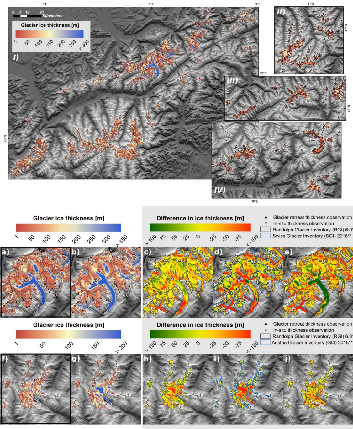
520 Figure 6: Reconstructed ice thickness ( H_{SIA2003}^{in-situ \& retreat} ) of glaciers in the European Alps ('2003'): I) Mont Blanc Group, Pennine & Bernese Alps, II) Ötztal & Stubai Alps, III) Zillertal Alps, Venediger & Glockner Group, IV) Silvretta Alps and comparison of estimated ice thickness distribution of Aletsch (CH) (a-e) and Pasterze Glacier (AT) (f-j) by this study and previously published reference ice thickness maps. Panel (a,f) and (b,g) show the distributed glacier thickness as estimated by the H_{SIA2003}^{in-situ \& retreat} (a,f) and H_{SIA2003}^{retreat} reconstructions, respectively (b,g), while panels (c-e & h-j) indicate vertical differences in reconstructed ice thickness
