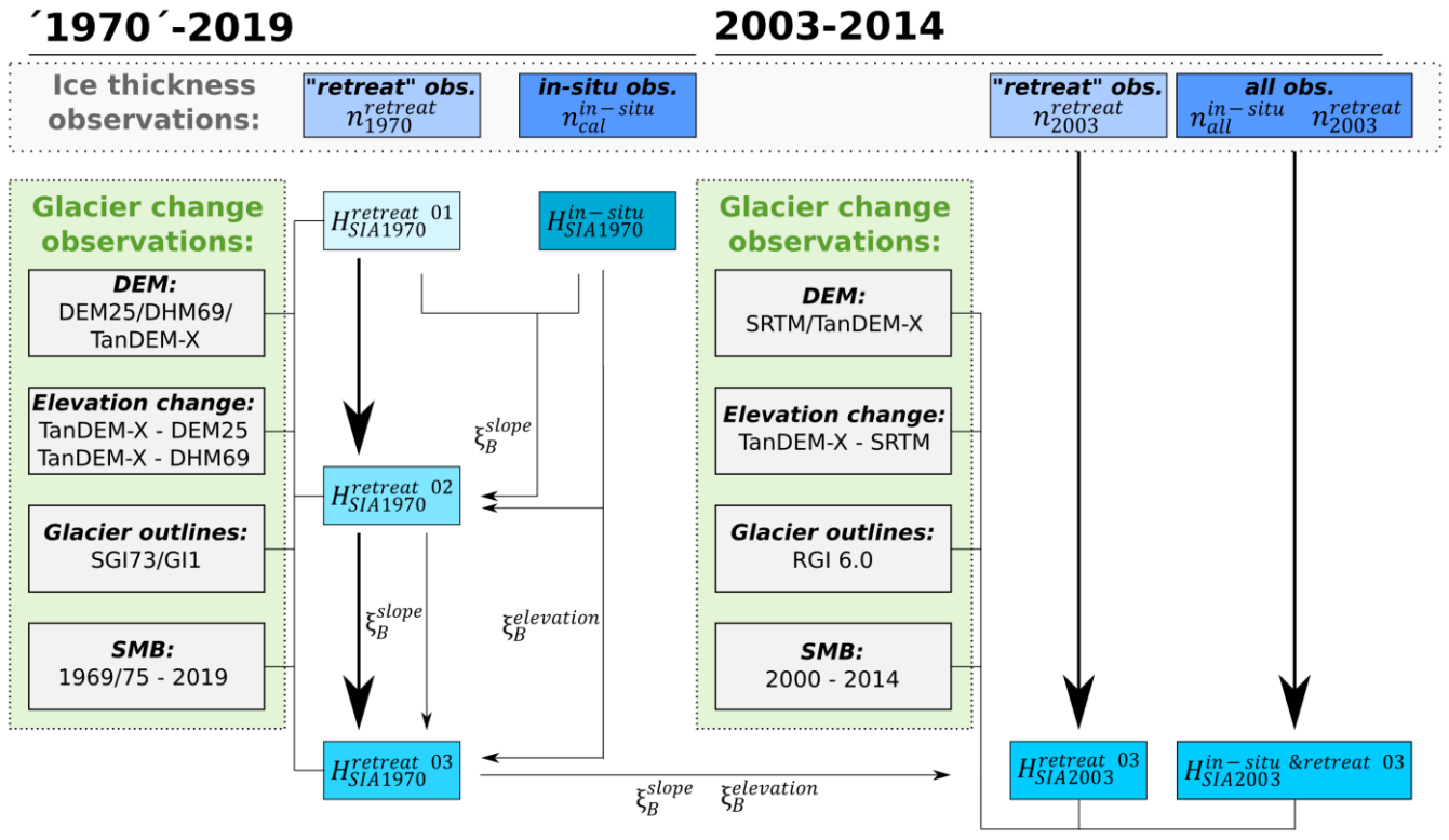
305 Figure 1: Visualization of experimental setup and input datasets: Over the period '1970'-2019, surface slope- and elevation-based scaling factors ( \xi_{\eta}^{slope} & \xi_{\eta}^{elevation} ) are calibrated by comparing the ice thickness distribution ( H_{SIA1970} ) derived from in-situ thickness observations ( H_{SIA1970}^{in-situ} ) and retreat thickness observations at the glacier margins ( H_{SIA1970}^{retreat} ). By iterating H_{SIA1970}^{retreat} ( H_{SIA1970}^{retreat\ 01} - H_{SIA1970}^{retreat\ 03} ), \xi_{\eta}^{slope} and \xi_{\eta}^{elevation} are calibrated. Eventually, the calibrated scaling factors ( \xi_{\eta}^{slope} & \xi_{\eta}^{elevation} ) are transferred to the period 2003-2014 to estimate the total alpine-wide glacier volume from different samples of ice thickness observations ( H_{SIA2003}^{in-situ \& retreat\ 03} & H_{SIA2003}^{retreat\ 03} ).
