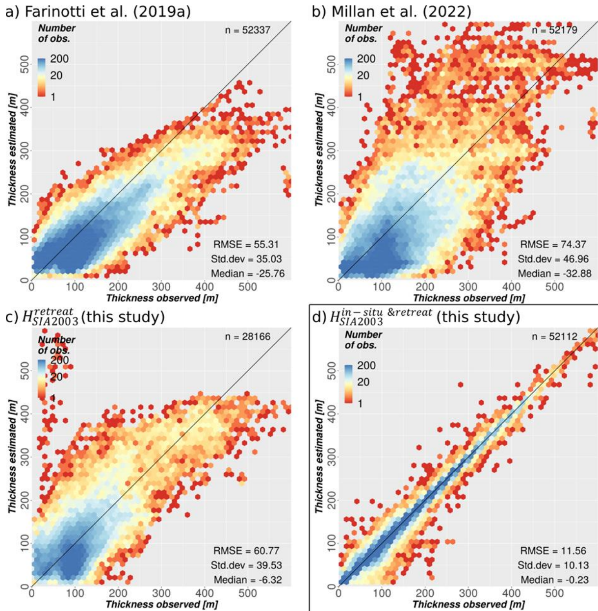
540 Figure 8: Difference between in-situ observed and estimated (2000) local ice thickness, root-mean-square-error (RMSE), standard deviation (Std.dev) and median difference (Median; all in metres) are stated in the lower right corner of each panel: Panel a) & b) refer to published ice thickness maps by Farinotti et al. (2019a) and Millan et al. (2022). Differences between estimated and observed ice thickness are derived from all available in-situ measurements (GlaThiDa; Grab et al. 2021). Deviations in ice thickness of the 545 H_{SIA2003}^{retreat} reconstruction of this study are shown in c). Note that in-situ observations from glaciers used to derive the viscosity scaling factors (section 2.5) are excluded from the comparison. Panel d) indicates the ice thickness distribution based on all available in-situ and retreat observations as well as the viscosity scaling factors ( H_{SIA2003}^{in-situ \& retreat} ). Note the logarithmic scaling of the thickness observations distribution. Darkblue areas indicate hexbins with more than 200 thickness measurement locations.
