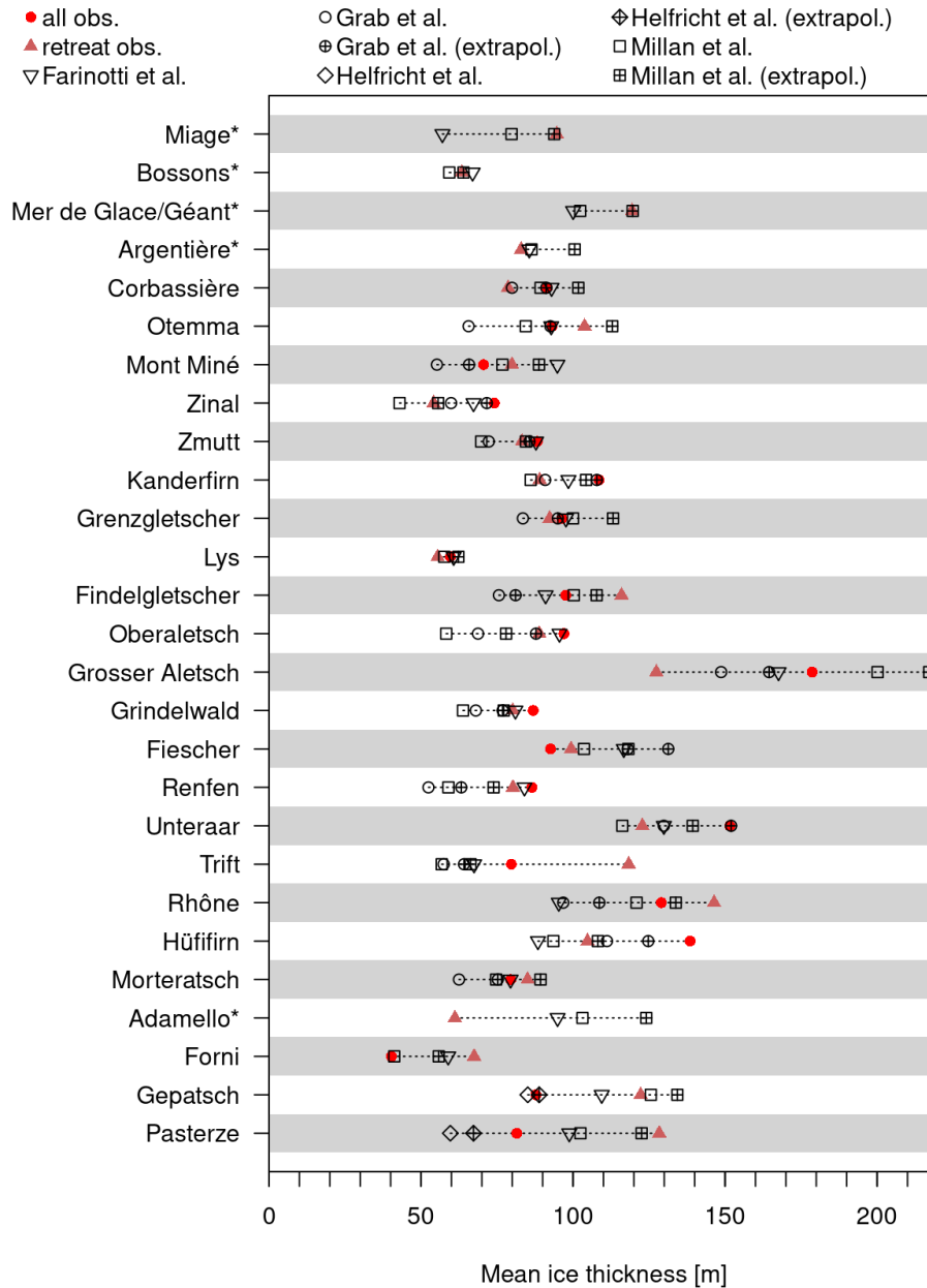
530 Figure 7: Mean ice thickness of large Alpine glaciers (> 10 km 2 ) estimated by this study and previous reconstructions (Farinotti et al., 2019a; Helfricht et al., 2019; Grab et al., 2021; Millan et al., 2022). Red dots and brown triangles indicate the mean H_{SIA2003}^{in-situ \& \text{retreat}} and H_{SIA2003}^{retreat} glacier thickness of this study. The reconstructions by (Helfricht et al., 2019), (Grab et al., 2021) and (Millan et al., 2022) refer to the years 2006, 2016 and 2017-18, respectively. Therefore, hollow symbols represent the original mean value derived from the published ice thickness maps while filled symbols show the mean glacier thickness temporally extrapolated to the year 2000. *For glaciers without in-situ observations, only the H_{SIA2003}^{retreat} reconstruction is shown. 535
