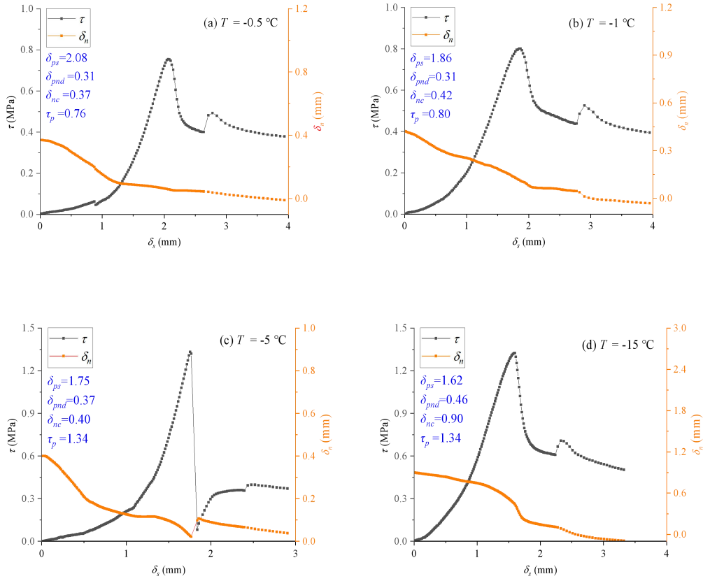
Figure 9. Shear strength and normal displacement versus the shear displacement for the profile of No. 4 in the temperature group. \delta_{ps} and \delta_{pnd} are the shear displacement and normal shear dilatancy at the point of peak shear strength, \tau_p and \delta_{nc} is the initial compression deformation.
