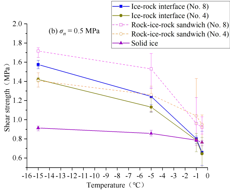
Figure 21. Influence of freezing temperature on the direct shear strength of ice and ice-filled joints. Experimental condition: v = 0.2 \text{ mm/min} .
