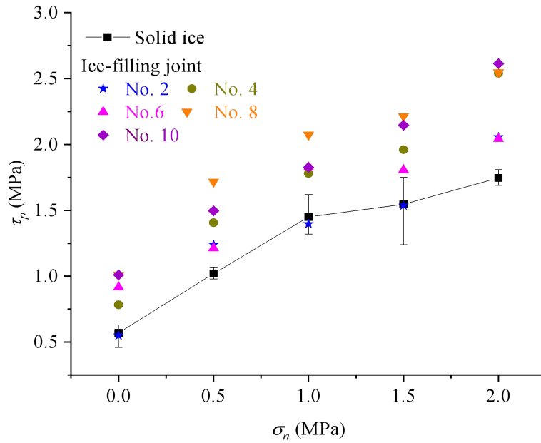
Figure 23. Shear failure characteristics of ice-rock interfaces under different normal stress. Experimental condition: v = 0.2\text{mm/min} , d = 2\text{ mm} , T = -15\text{ }^{\circ}\text{C} .
