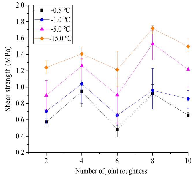
Figure 5. Shear strength against joint roughness at different freezing temperatures. Experimental condition: \nu = 0.2
