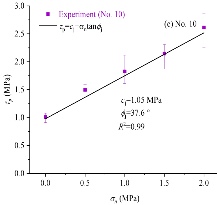
Figure 17. Effect of normal stress on the peak shear strength of ice-filled joints. Experimental condition: T = -15^\circ\text{C} , v = 0.2 mm/min and d = 2 mm.
