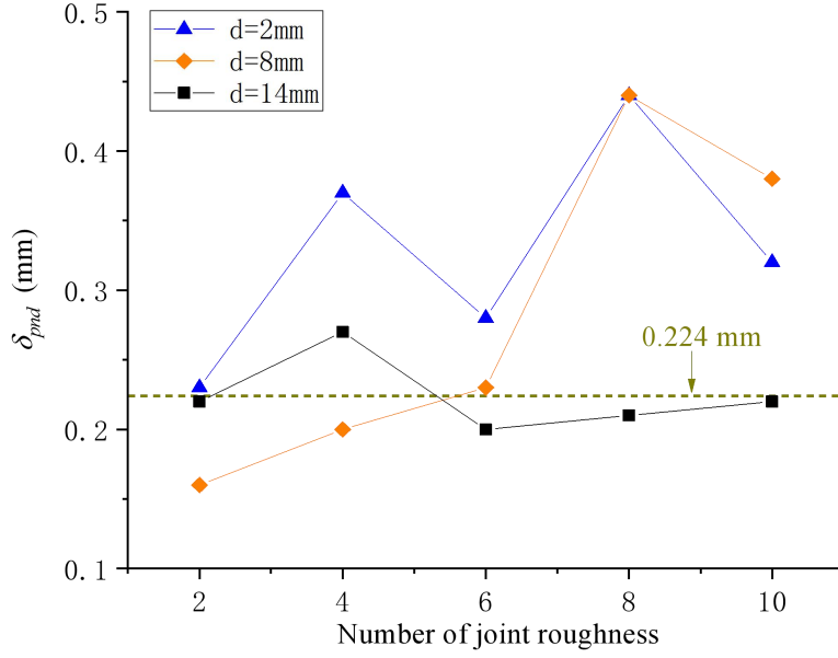
Figure 16. Effect of joint opening on the shearing dilatancy. Experimental condition: T = -5\text{ }^{\circ}\text{C} , v = 0.2\text{ mm/min} and \sigma_n = 0.5\text{ MPa} .
