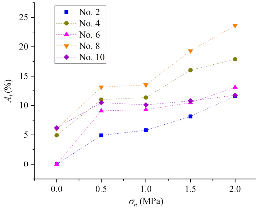
Figure 19. Aggregation area of rupture ice increases with increasing normal stress. Experimental condition: T = -15\text{ }^{\circ}\text{C} , d = 2\text{ mm} and v = 0.2\text{ mm/min} .
