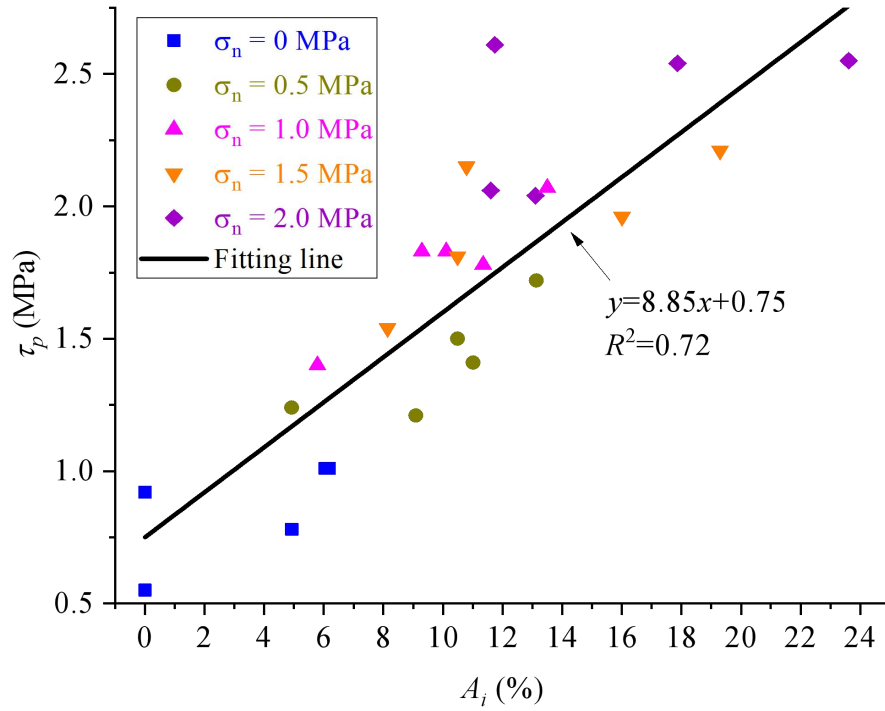
Figure 20. Peak shear strength linearly increases with increasing aggregation areas of rupture ice. Experimental condition: T = -15\text{ }^{\circ}\text{C} , d = 2\text{ mm} and v = 0.2\text{ mm/min} .
