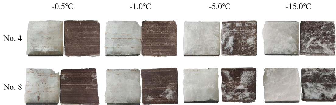
Figure 22. Shear failure characteristics of ice-rock interfaces under different temperatures. Experimental condition: v = 0.2 \text{ mm/min} , \sigma_n = 0.5 \text{ MPa} .
