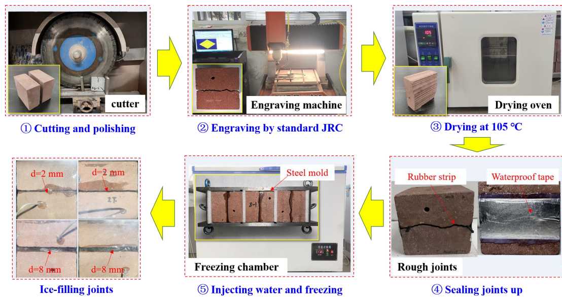
Figure 1. Preparation of ice-filled joints. The preparation steps are as follows: ① Cutting and polishing, ② Engraving by standard, ③ Drying at 105 °C, ④ Sealing joints up, ⑤ Injecting water and freezing.
