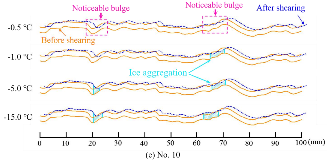
Figure 7. Shear aggregation areas of ice along the profile of roughness. Experimental condition: v = 0.2 mm/min, d = 2 mm, \sigma_n = 0.5 MPa. Some blue profiles (dotted curves) are located under the orange profiles (solid curves) after shearing, which means the width of joints becomes smaller. Generally, the reduction of joint width occurs before some bulges and the rupture ice will aggregate before these bulges. The bulges causing the reduction of joint width and aggregation of ice are called noticeable bulges. The noticeable bulges have larger inclination angles and they are far away from the joint edges.
