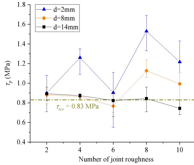
351 352 Figure 14. Effect of joint opening on the peak shear strength. Experimental condition: T = -5\text{ }^{\circ}\text{C} , v = 0.2\text{ mm/min} 353 and \sigma_n = 0.5\text{ MPa} .
