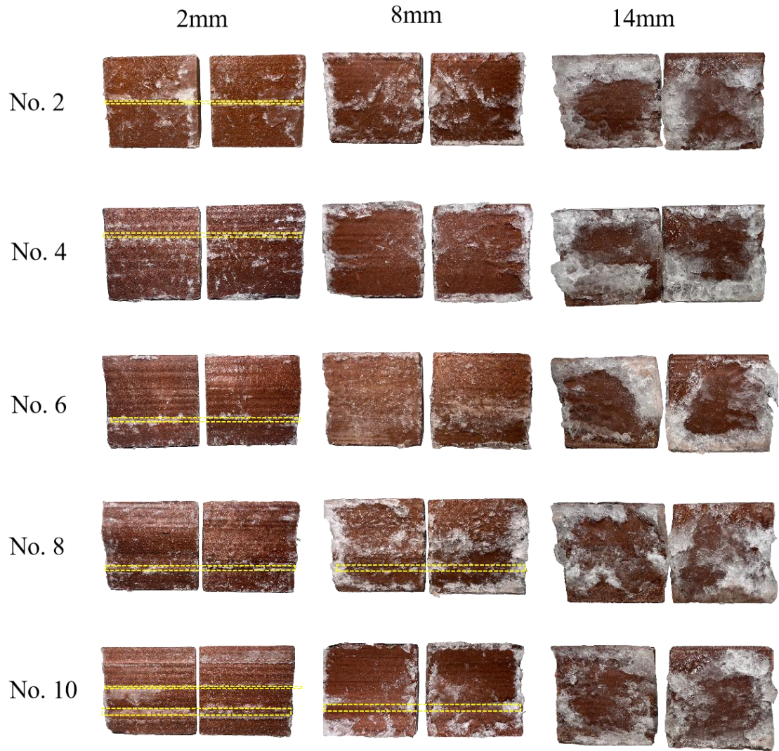
Figure 13. The shear rupture characteristics of ice-filled joints with different openings. Experimental condition: T = -5\text{ }^{\circ}\text{C} , d = 2\text{ mm} and \sigma_n = 0.5\text{ MPa} . The yellow lines show the main aggregation of rupture ice. Ice after rupture will aggregate in roughness bulges perpendicular to the shear direction. The aggregation phenomenon disappears
