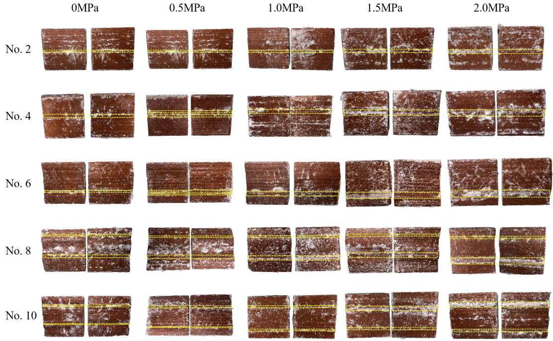
Figure 18. Aggregation of rupture ice under different normal stresses. Experimental condition: T = -15\text{ }^{\circ}\text{C} , d = 2 mm and v = 0.2\text{ mm/min} . The yellow lines show the main aggregation of rupture ice.
