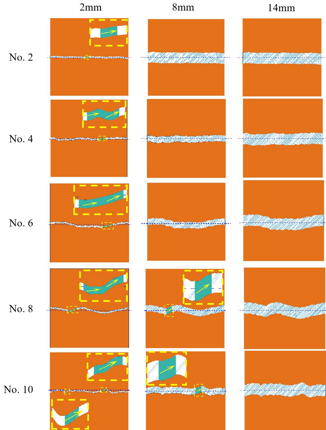
Figure 15. Influence of joint roughness on the shearing slip path. Experimental condition: T = -5\text{ }^{\circ}\text{C} , \nu = 0.2 mm/min and \sigma_n = 0.5\text{ MPa} .
