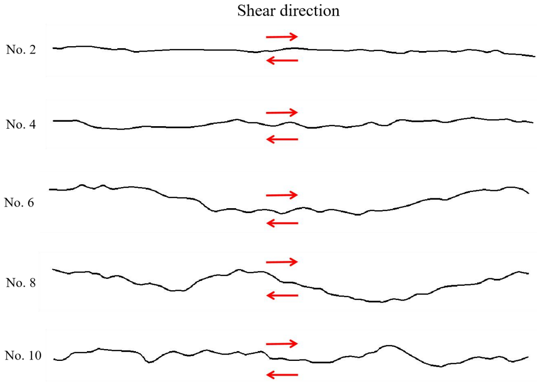
Figure 2. The shear directions for different joint profiles.
