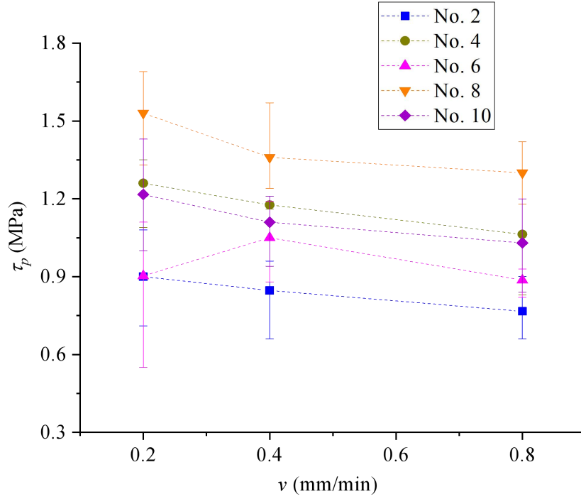
Figure 11. Effect of shear rate on the peak shear strength. Experimental condition: T = -5 °C, d = 2 mm and \sigma_n = 0.5 MPa.
