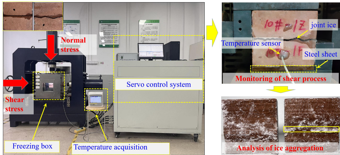
Figure 4. Shear experiment procedure and equipment
