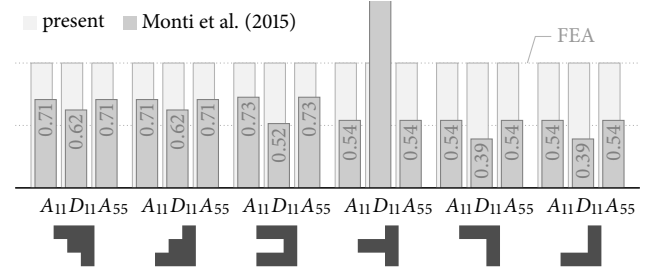
Figure 11. Slab extension, bending, and shear stiffnesses A_{11} (N/mm), D_{11} (Nmm), and A_{55} (N/mm) of the present model and the equivalent isotropic slab approach by Monti et al. (2015) normalized to the finite element analysis (FEA) reference stiffness. The bending–extension coupling stiffness B_{11} (N) is not shown because it is always zero in the model of Monti et al. (2015) and agrees exactly between reference and present model, see Table 3.
