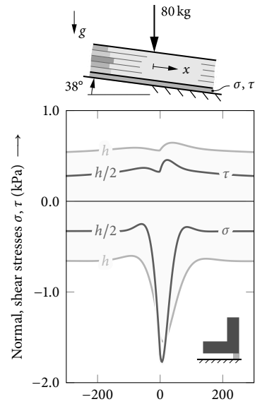
Figure 15. Effect of changes of the slab thickness h on shear and normal stress in the weak layer under skier loading, shown for profile F .
