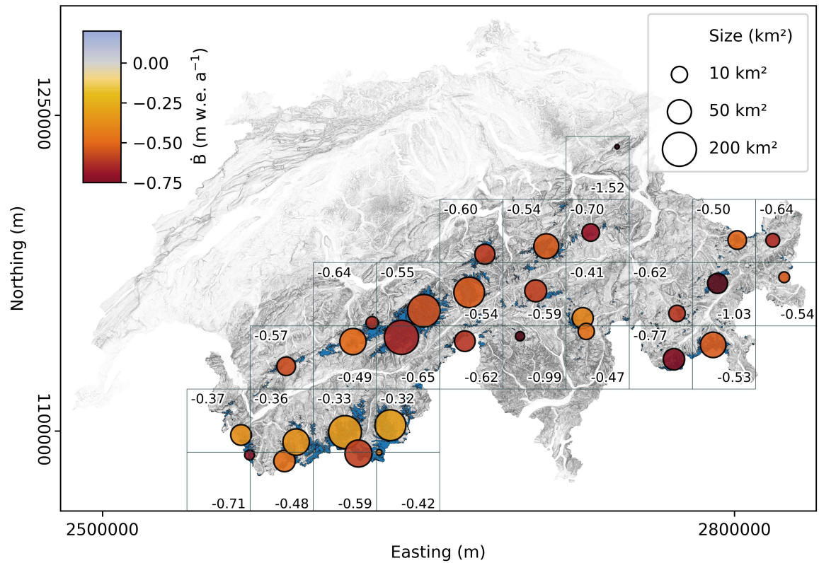
Figure 7. Area-weighted geodetic mass balance rates (colours and numbers) for 30 km × 30 km tiles (grey squares). The location of each circle is the average glacier centroid weighted by area in the tile, and their sizes indicate the glacier area in ca. 1931.
