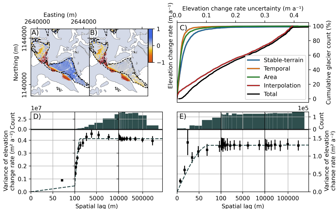
Figure 4. Error figure ensemble. A+B) Differences of an individual DEM before ( A ) and after ( B ) coregistration. The arrows indicate the locations and directions of the images used for generating the ca. 1931 DEM. The dashed lines indicate the theoretical viewshed of the stereo-pair (pre-calculated by swisstopo). C) Histogram-Cumulative histograms showing the magnitude of the different components for the elevation change uncertainty of each individual glacier. D+E) variograms of interpolated ( D ) and stable-terrain ( E ) elevation difference uncertainties, showing the variance of all pairs of pixels at a given distance (or lag) as a function of that lag. The individual markers show the empirically derived variance, their error bars show their 95% confidence intervals, and the dashed line shows the variogram model (sum of two spherical models). The histograms above the variograms show the pairwise sample count for each empirically derived variance marker.
