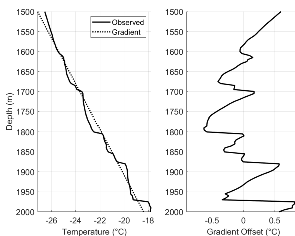
Figure 5. Offsets from the mean ice temperature gradient highlight the influence of large (c. 50 m) convection cells forming in the borehole fluid in a deep section of the NEEM ice temperature profile measured in 2011. These borehole fluid convection cells contribute to disturbance uncertainty associated with an equilibrating borehole temperature profile when the borehole logging technique is used. This uncertainty is avoided when sensors or cables are frozen into the ice in other measurement techniques.
