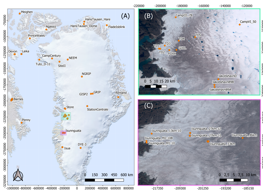
Figure 1. (A): Overview of the drill site locations of temperature profiles contained in the database (plot created using QGreenland, Moon et al. (2021)). Note, locations where several drill sites exist close to each other, only the common name is shown, e.g. Agassiz. The green and purple box indicates regions where numerous profiles have been drilled. (B): Zoomed view of the region near Jakobshavn glacier. (C): Zoomed view of the region near Isunnguata Sermia glacier. Panels (B) and (C) show positions plotted on top of Sentinel-2 multispectral satellite imagery, 10 m resolution from 2019 (MacGregor et al., 2020). All maps are displayed in EPSG: 3413 polar stereographic projection, with the Easting and Northing given in meters.
