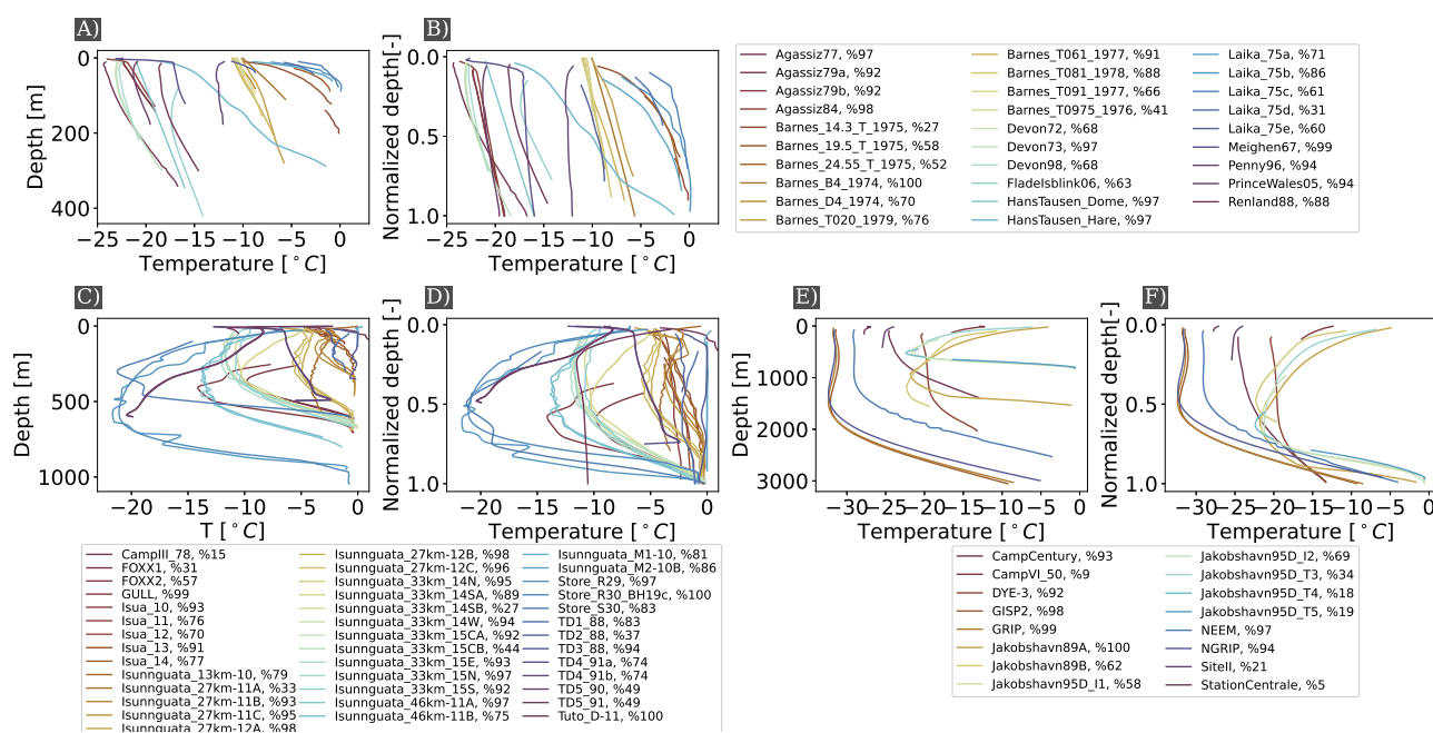
Figure 3. Overview of all ice temperature profiles in the database expressed in both absolute depth (A),(C),(E) and normalized depth (B),(D),(F). For visibility, the profiles are divided into local ice caps (A)-(B), marginal ice-sheet sites (C)-(D), and inland ice-sheet sites (E)-(F). The local ice thickness coverage of each individual profile is given as a percentage.
