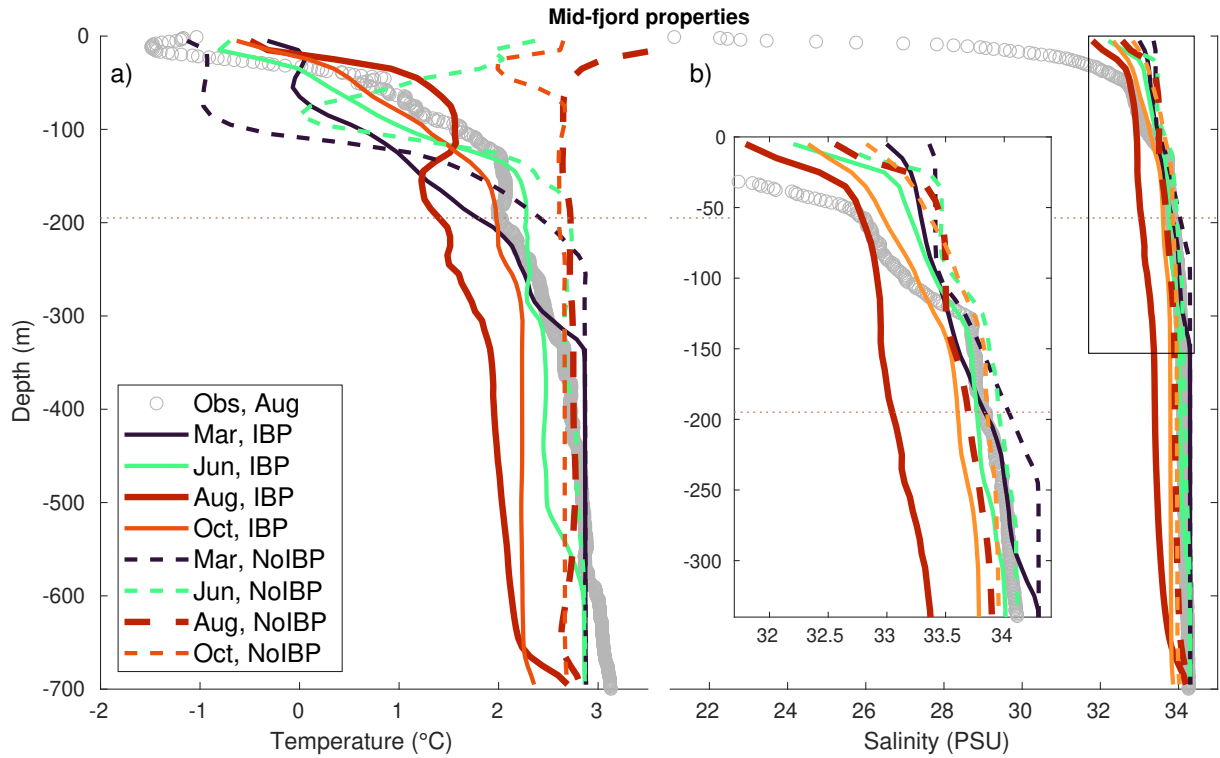
Figure 8. Mid-fjord temperature and salinity profiles for March (winter), June (early season), August (peak season) and October (late season) for both IBP (solid lines), NoIBP (dashed lines). Grey circles indicate the XCTD profiles in August 2014 (Beaird et al., 2017). The dotted horizontal line marks 195 m depth, which coincides in IBP with isopycnal 26.5 \text{ kg m}^{-3} and the inflow/outflow border in August, and in the observations with isopycnal 26.9 \text{ kg m}^{-3} . Mid-fjord location is indicated with a red star and vertical dotted lines in Fig. 3 and in Fig. 1, and as an outlined red star in Fig. 1.
