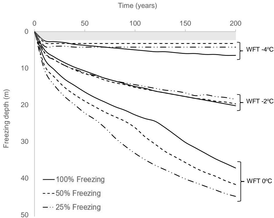
Figure 6. Mid-Holocene permafrost aggradation with variable freezing degrees. MAAT was set to -4°C (Park et al., 2019), and freezing proportions were taken as 100%, 50% and 25%. The shaded/grayish zone represents a hypothetical, conservative, active layer, which is taken as 2 m thick. We note that active layer in Adventdalen is usually \leq 1 m, and 2 m was chosen due to the higher temperature during the mid-Holocene.
