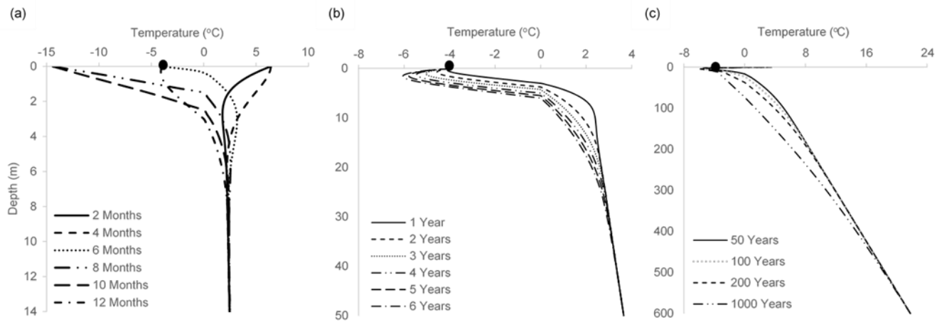
Figure 4. 1-D freezing model results for: (a) 1 year; the model starts (and finishes) at spring, defined as mid-time between minimum and maximum surface T (e.g. May), followed by summer increase in temperature (solid and dashed lines), cooling and start of freezing during fall (dotted line, e.g. November), followed by colder winter months (two-points dashed line and wide dashed line) and concluding in the spring (one point dashed line); (b) 6 years (starting in spring). (c) 50 to 1000 years. MAAT -4 \pm 12^{\circ}\text{C} , WFT set at 0^{\circ}\text{C} , 100% freezing. Full black circles denote -4^{\circ}\text{C} . Note the different scale between (a) (b) and (c).
