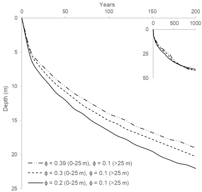
585 Figure 10. Simulations as in Fig. 9, but with WFT of -2^{\circ}\text{C} .
